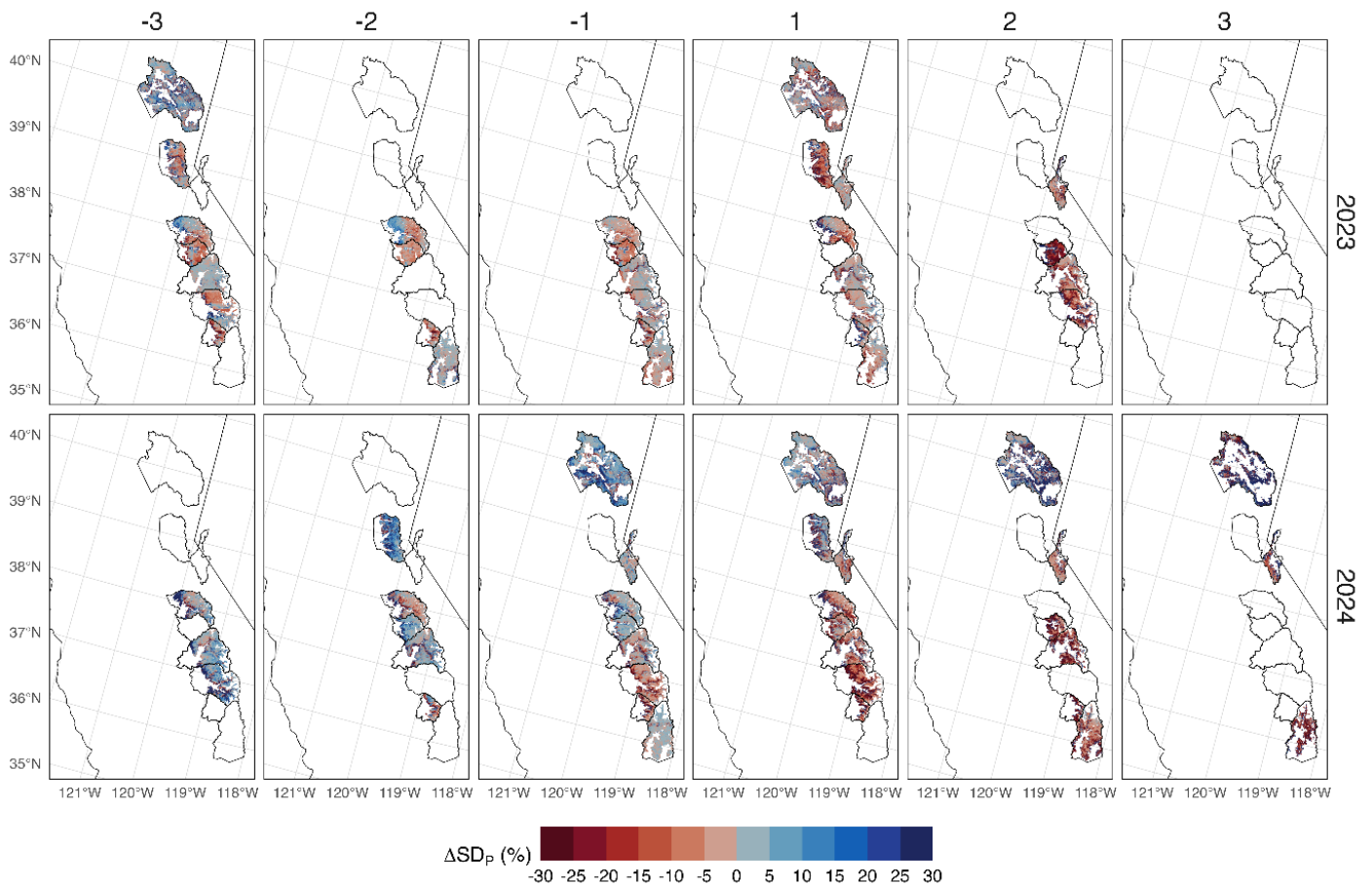
Figure 4. Maps of post-fire snow depth percent difference ( \Delta\text{SD}_P ) for water years 2023 and 2024—the years with the most lidar acquisitions—across nine study basins by month since peak SWE. See Figure S4 for maps from other years.
