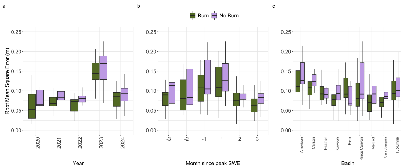
Figure 2. Cross validated root mean squared error (CV-RMSE) for burned (redgreen) and unburned (bluepurple) pixels for every acquisition by (a) year of flight, (b) month since peak SWE, and (c) basin.
