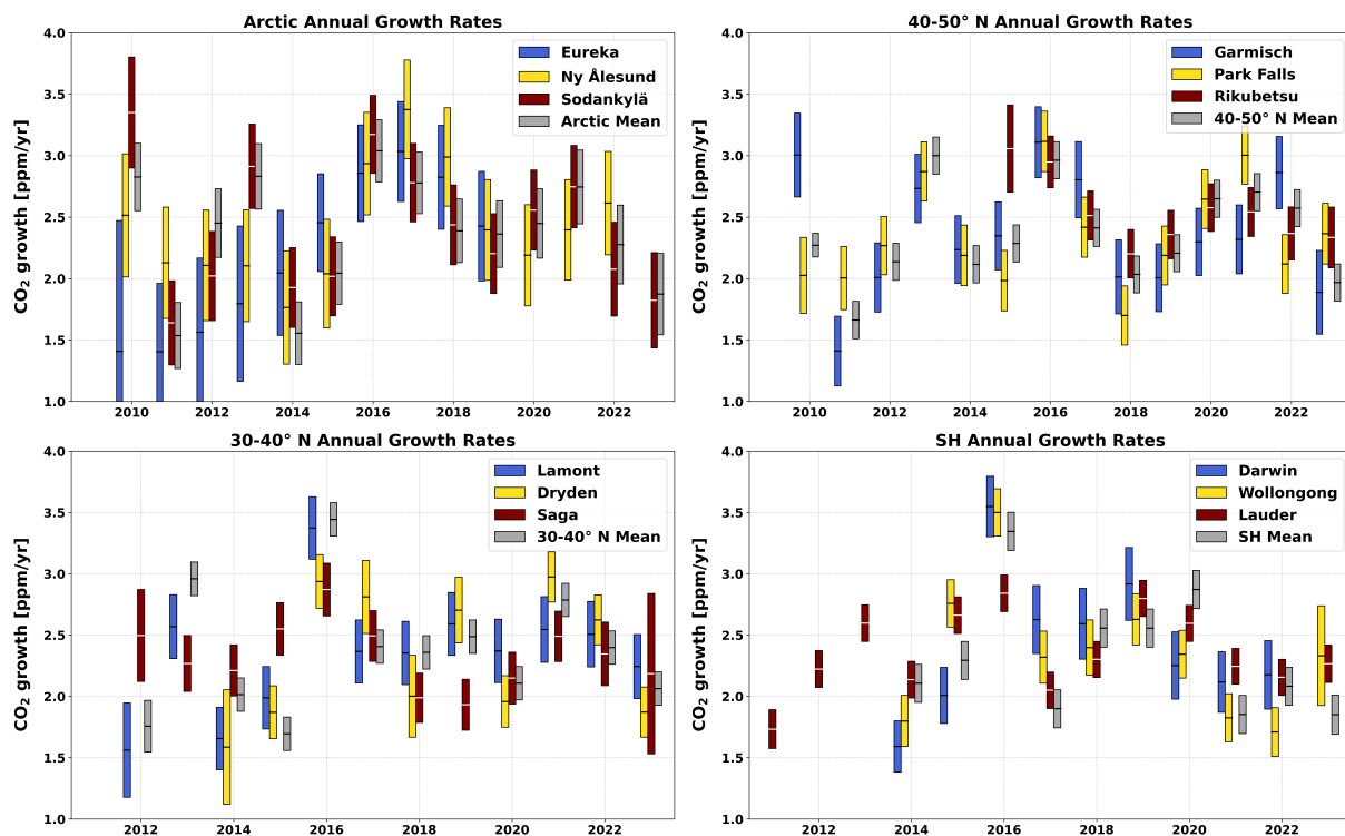
Figure A5. Annual CO 2 growth rates derived from TCCON stations, covering 2009–2024. Each panel corresponds to a different study region: (top left) Arctic sites, (top right) 40–50°N, (bottom left) 30–40°N, and (bottom right) Southern Hemisphere sites. Colored bars show annual growth rates for individual stations, and grey bars indicate the average of all sites within the region. The central line within each bar indicates the median growth rate, and the bar length reflects the associated uncertainty.
