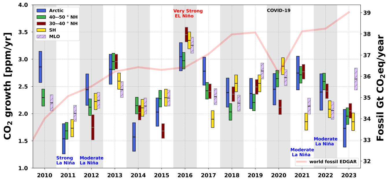
Figure 4. Annual growth rates and their uncertainty ranges for the four TCCON regions and MLO, calculated using the DLM method shown by year. The central line within each bar indicates the median growth rate, and the bar length reflects the associated uncertainty. The red line represents global fossil fuel CO 2 emission trends from EDGAR.
