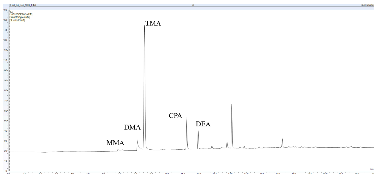
Figure S1. Chromatogram showing the retention times of MMA, DMA, TMA, CPA and DEA of an amine sample.
