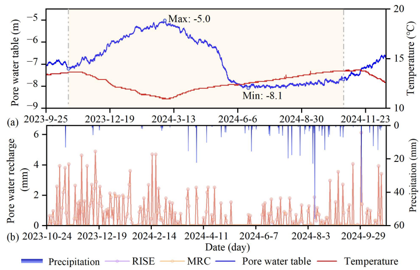
Fig. 9. Temporal dynamics of pore water table depth, temperature, precipitation, and recharge in the gully region of the Loess Plateau.
