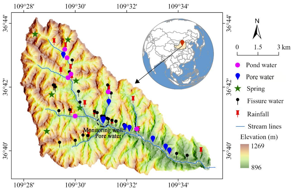
Fig. 2. The geographical location and sampling sites for rainfall, pond water, pore water, spring water, and fissure water in the Nianzhuang catchment.
