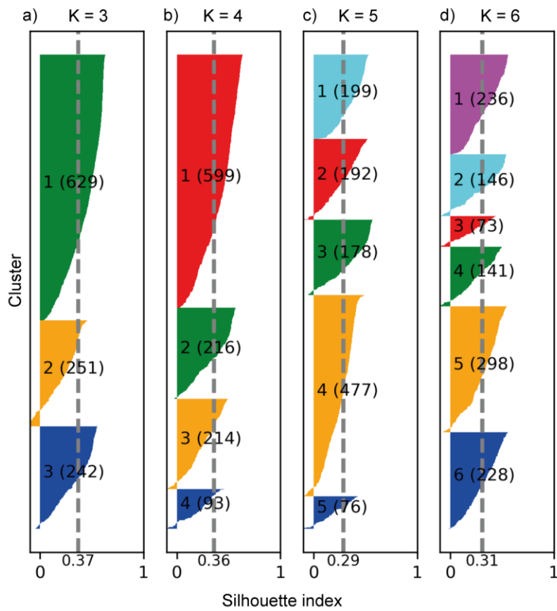
Figure 8 Silhouette index analysis for the Endelave dataset. Four clustering routines were run with different number of clusters, K, (a) three, (b) four, (c) five and (d) six. The sorted silhouette indices are shown for each cluster with the average index indicated by the grey dashed line.
