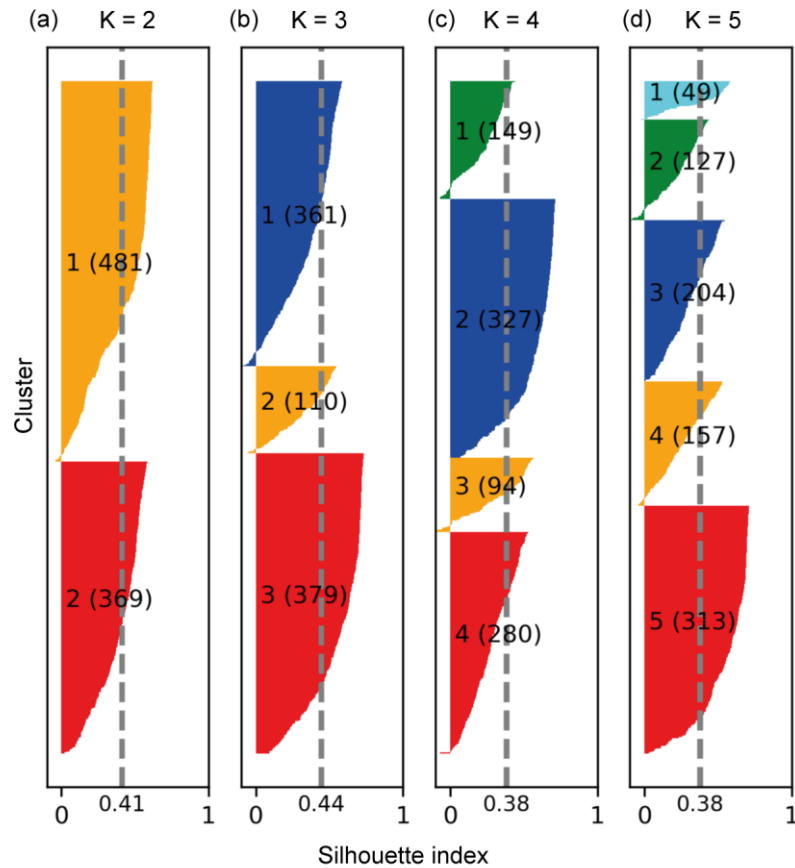
Figure 3 Silhouette index analysis for the Kompedal dataset. Four clustering routines were run with different number of clusters, K , (a) two, (b) three, (c) four and (d) five. The sorted silhouette indices are shown for each cluster with the average index indicated by the grey dashed line.
