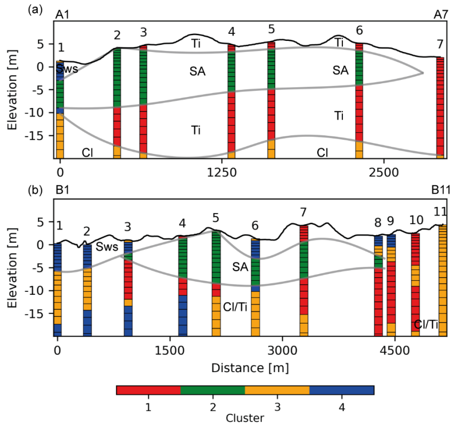
Figure 10 Clustering sections from Endelave where the partitioning of data is shown at every sounding location. (a) Section 1 (b) Section 2 in Figure 2. The grey lines track selected cluster boundaries. A is increasing in the Southeast direction. B is increasing in the South direction.
