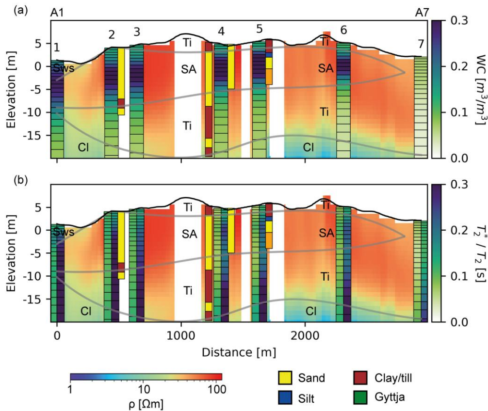
Figure 11 Profile of 7 SNMR soundings (bars) and TEM \rho (background). Section 1 in Figure 2 Figure 2 Figure 2b . (a) SNMR WC (b) a split bar with T_2^* (left) and T_2 (right). Grey lines are tracking transitions between clusters in Figure 10 Figure 10 Figure 10 . A is increasing in the Southeast direction.
