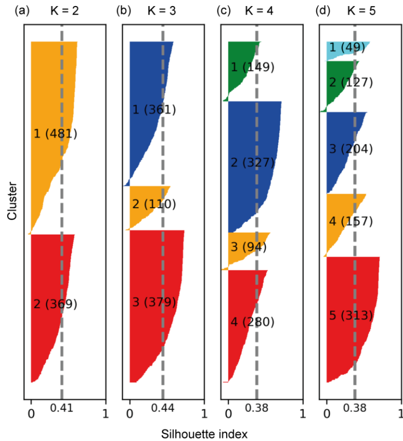
Figure 3 Silhouette index analysis for the Kompedal dataset. Four clustering routines were run with different number of clusters, K, (a) two, (b) three, (c) four and (d) five. The sorted silhouette values-indices are shown for each cluster with the average value-index indicated by the grey dashed line.
