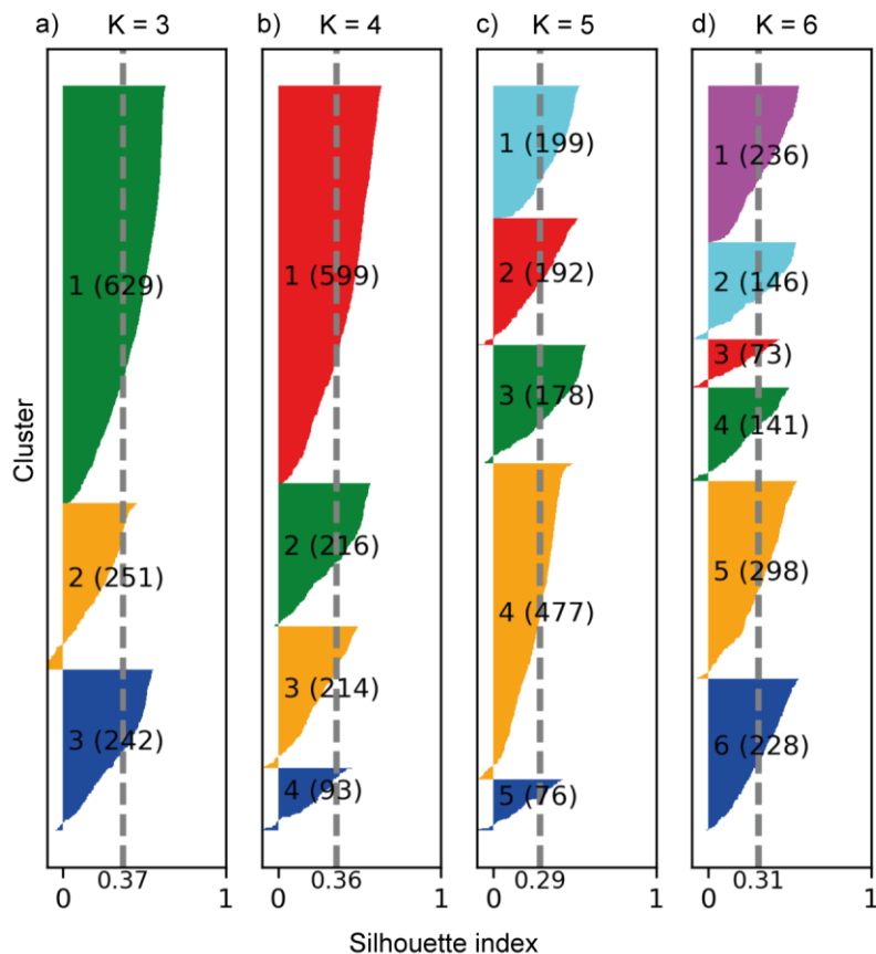
Figure 8 Silhouette index analysis for the Endelave dataset. Four clustering routines were run with different number of clusters, K, (a) three, (b) four, (c) five and (d) six. The sorted silhouette values-indices are shown for each cluster with the average value-index indicated by the grey dashed line.
