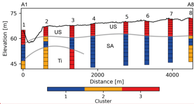
15 16 Figure 55 Clustering section from Kompedal where the partitioning of data is shown at every sounding. The grey 17 lines track selected cluster boundaries. See Table 1 for cluster descriptions. A is increasing in the South direction.
