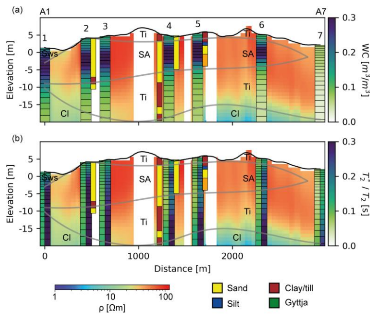
Figure 11: Profile of 7 SNMR soundings (bars) and TEM \rho (background). Section 1 in Figure 2. (a) SNMR WC (b) a split bar with T_2^* (left) and T_2 (right). Grey lines are tracking transitions between clusters in Figure 9. A is increasing in the Southeast direction.
