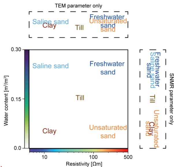
Figure 14. Different hydrogeological units resolved with TEM and SNMR. In dashed boxes, only one method is used, and the overlapping units show the ambiguities found. T_2^* can be implemented to further separate units. Colors in text are not related to colorbars.
