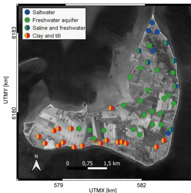
Figure 13.12 Sounding locations where salt water or fresh water has been identified. Locations with only clay and till clusters are shown with red and yellow. Map data: © Google Maps 2024, UTM Zone: 32N.
