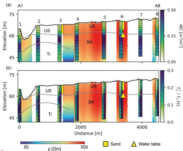
16 Figure 66 Profile of 8 SNMR soundings (bars) and TEM profile (background). Section 1 in Figure 2 Figure 2a . (a) 17 SNMR WC, (b) a split bar with T_2^* (left) and T_2 (right). Boreholes at sounding location 3 and 6 are shifted \sim 40 m to 18 avoid overlapping with the bars. Grey lines are tracking transitions between clusters in Figure 5 Figure 5 . A is 19 increasing in the South direction.
