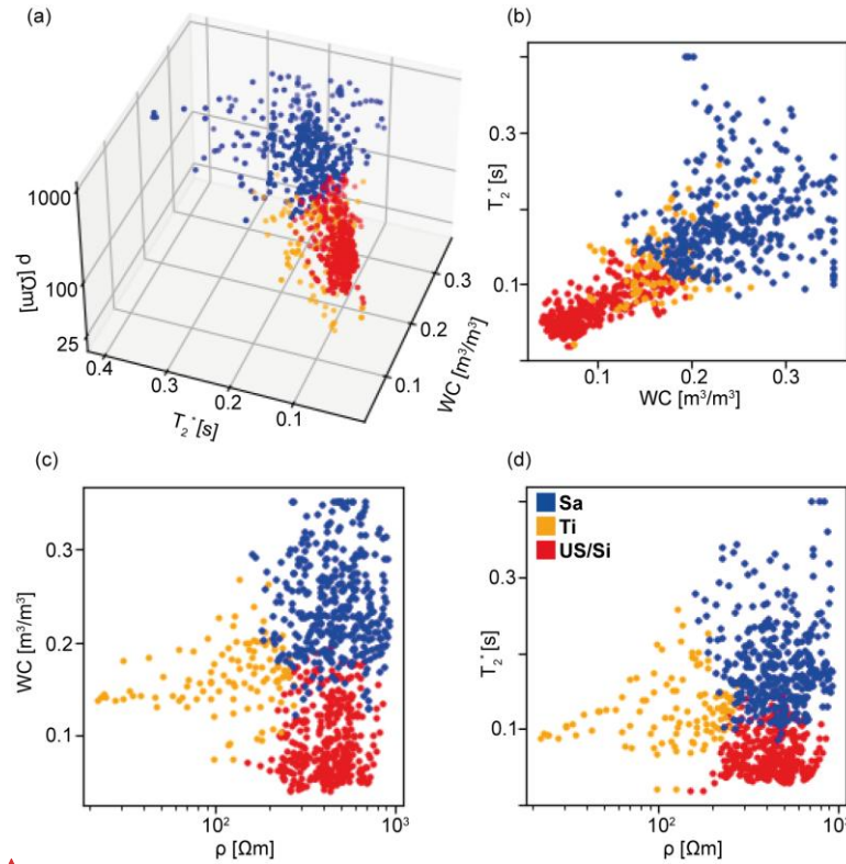
3 ▲ 4 Figure 44 Clustering results from the Kompedal survey on three parameters: WC , T_2^* and \rho . (a) all three parameters 5 in a scatter, (b) WC and T_2^* , (c) \rho and WC , and (d) \rho and T_2^* . The color of each datapoint defines the assigned 6 cluster; 1-blue, 2-yellow, and 3-red, and their interpreted geology seen in table 1.
