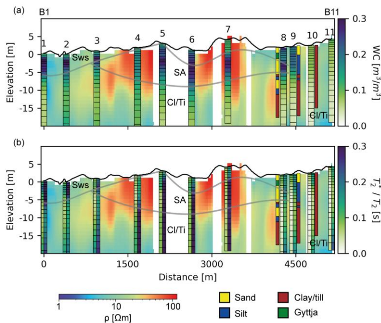
Figure 12: Profile of 11 SNMR soundings (bars) and TEM \rho (background). Section 2 in Figure 2. (a) SNMR WC (b) a split bar with T_2^* (left) and T_2 (right). Grey lines are tracking transitions between clusters in Figure 10. B is increasing in the South direction.
