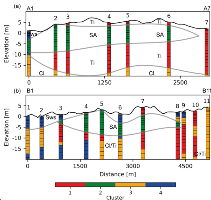
Figure 109 Clustering sections from Endelave where the partitioning of data is shown at every sounding location. (a) Section 1 (b) Section 2 in Figure 2. The grey lines track selected cluster boundaries. A is increasing in the Southeast direction. B is increasing in the South direction.
