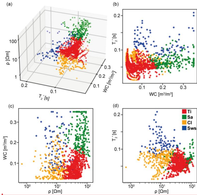
6 ▲ 7 Figure 98 Clustering results from the Endelave survey on WC, T_2^* and \rho . (a) all three in a scatter, (b) WC and T_2^* , 8 (c) \rho and WC, and (d) \rho and T_2^* . The color of each datapoint defines the assigned cluster , and their 9 interpreted geology , abbreviations seen in table 2.
