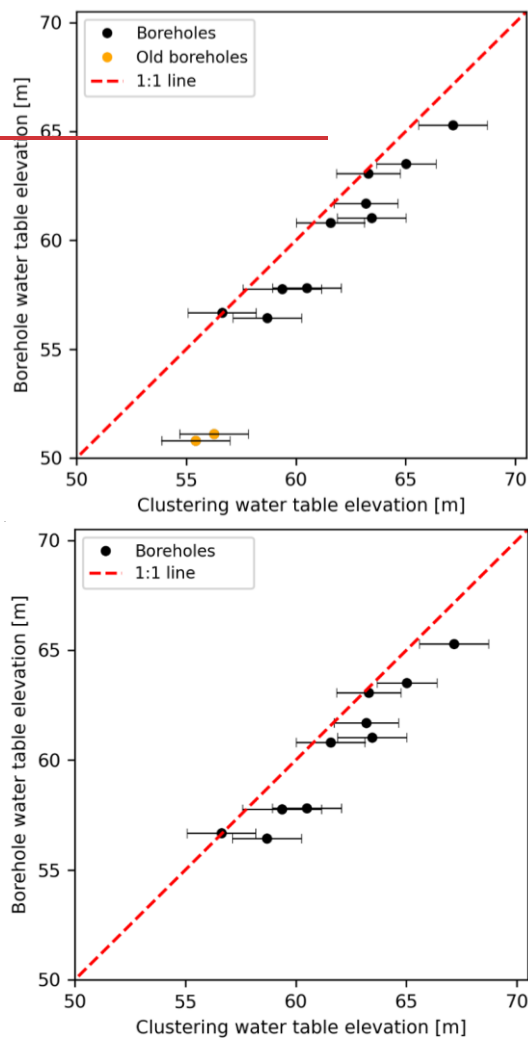
5 Figure Z7 Borehole water table compared to the clustering water table at 12 SNMR locations with boreholes within 6 500 m. The red line has a slope of 1 and the error bars on the clustering estimates are based on the inversion 7 layer thickness just below the water table estimate to provide a type of uncertainty. Yellow points have water table 8 measurements over 40 years old.
