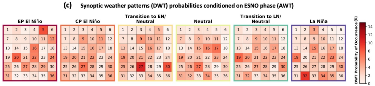
Figure 3: Statistical relationships between climate and weather patterns in the climate emulator. (a) Synthetic daily weather types (DWTs) classified based on synoptic weather patterns derived from k-means clustered PCs of sea level pressure and sea level pressure gradients extracted from a domain representing where 99 % of wave energy that reaches the site of interest is generated. Probability of DWT occurrence based on seasonality (b) and ENSO phase (annual weather type; AWT, c)
