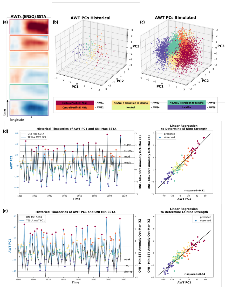
Figure 2: Synthetic annual weather types (AWTs) in the stochastic climate emulator classified based on ENSO phase and strength. (a) Six AWTs are generated using k-means clustering of leading principal components (PCs) of sea-surface temperature anomaly Hovmöller plots. (b) AWT PCs from historical datasets compared to (c) simulated AWT PCs highlights the climate emulator's ability to produce new weather types, dependent on the statistics of historical observations, but with the ability to extrapolate beyond observed events. (d & e) A linear regression between the leading AWT PC and historical ONI (maximums or minimums) enables classification of simulated AWTs by El Niño or La Niña strength.
