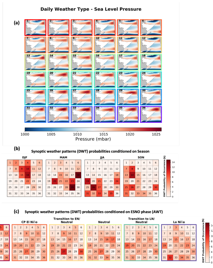
Figure 3: Statistical relationships between climate and weather patterns in the climate emulator. (a) Synthetic daily weather types (DWTs) classified based on synoptic weather patterns derived from k-means clustered PCs of sea level pressure and sea level pressure gradients extracted from a domain representing where 99 % of wave energy that reaches the site of interest is generated. Probability of DWT occurrence based on seasonality (b) and ENSO phase (annual weather type; AWT, c)
