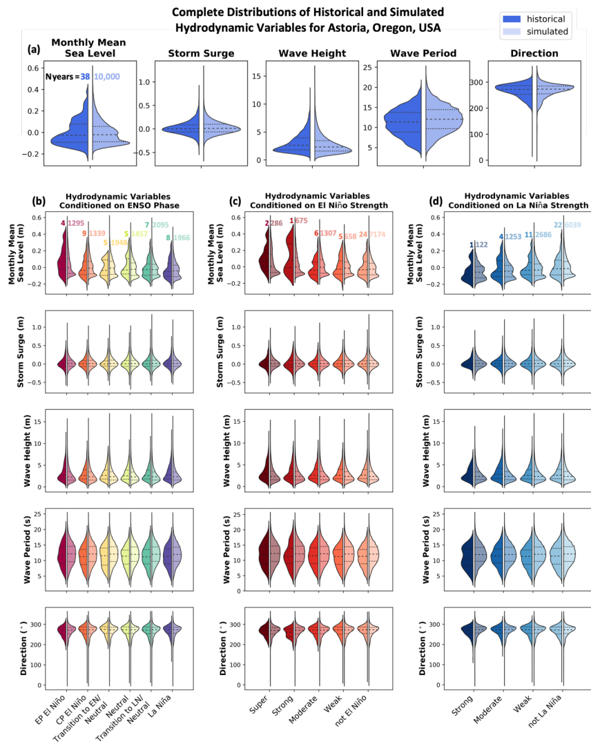
Figure 4: Split violin plots comparing the historical (left, darker colors) and simulated (right, lighter colors) probability distribution functions (pdfs) of the hydrodynamic outputs of the stochastic climate emulator. Comparisons are shown for (a) the entire historical (38 years) and simulated (10,000 years) periods and (b) conditioned on ENSO phase (Annual Weather Type; AWT), (c) El Niño intensity, (d) La Niña intensity. Dashed lines show the 0.25, 0.5, and 0.75 quantiles of each distribution, and numbers bordering distributions reflect the number of years of data included in each distribution (though data is in hourly or monthly resolution). Note, since ENSO phase does not align to calendar year, the simulated distributions conditioned on ENSO contain 100 partial years (the N years sums to 10,100).
