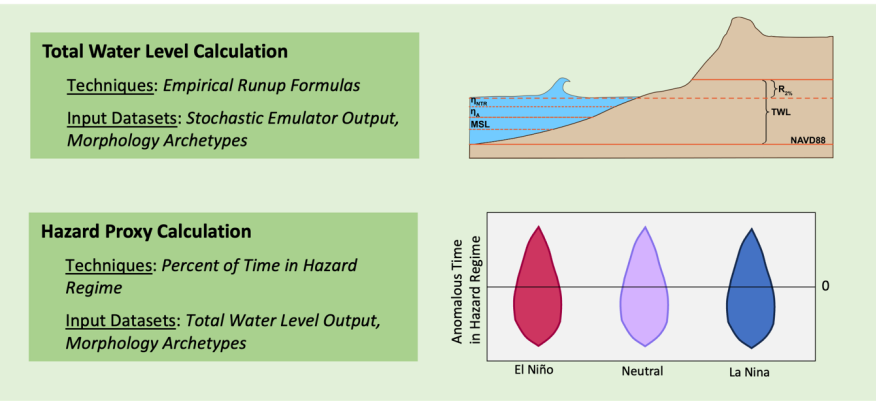
325 Figure 1: A methodological overview of the techniques and datasets employed in this analysis. A stochastic climate emulator is used to generate climate-aware simulations of hydrodynamic data, while total water level calculations and hazard proxies are used to assess the influence of climate and weather on hazard exposure.
