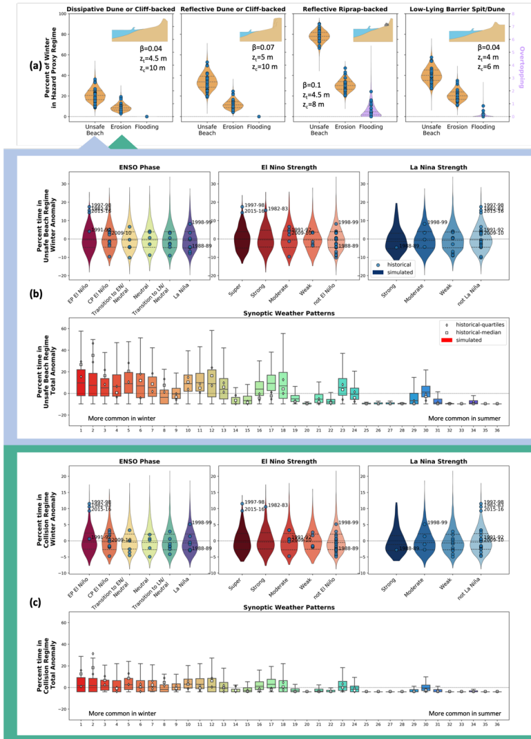
605 Figure 6: (a) Percentage of time spent in the three hazard proxy regimes for four representative beach morphologies for the PNW during winter; violin plots show simulated winters while scatter points show historical winters. Note overtopping is shown on a different y-axis. Inset sketches and morphologic variables show key features for each beach, where \beta is beach slope, z_t is backshore feature toe elevation, and z_c is backshore feature crest elevation. For the dissipative sandy-dune-backed morphology, we conditioned the unsafe beach and erosion proxies on ENSO phase, El Niño Strength, La Niña strength, and synoptic weather pattern in (b) and (c) respectively. Violin plots show the full simulated distributions of winter impact anomalies, while boxplot whiskers show up to the 0.05 and 0.95 quantiles of the simulated anomalies for the full (not just winter) distribution. 610
