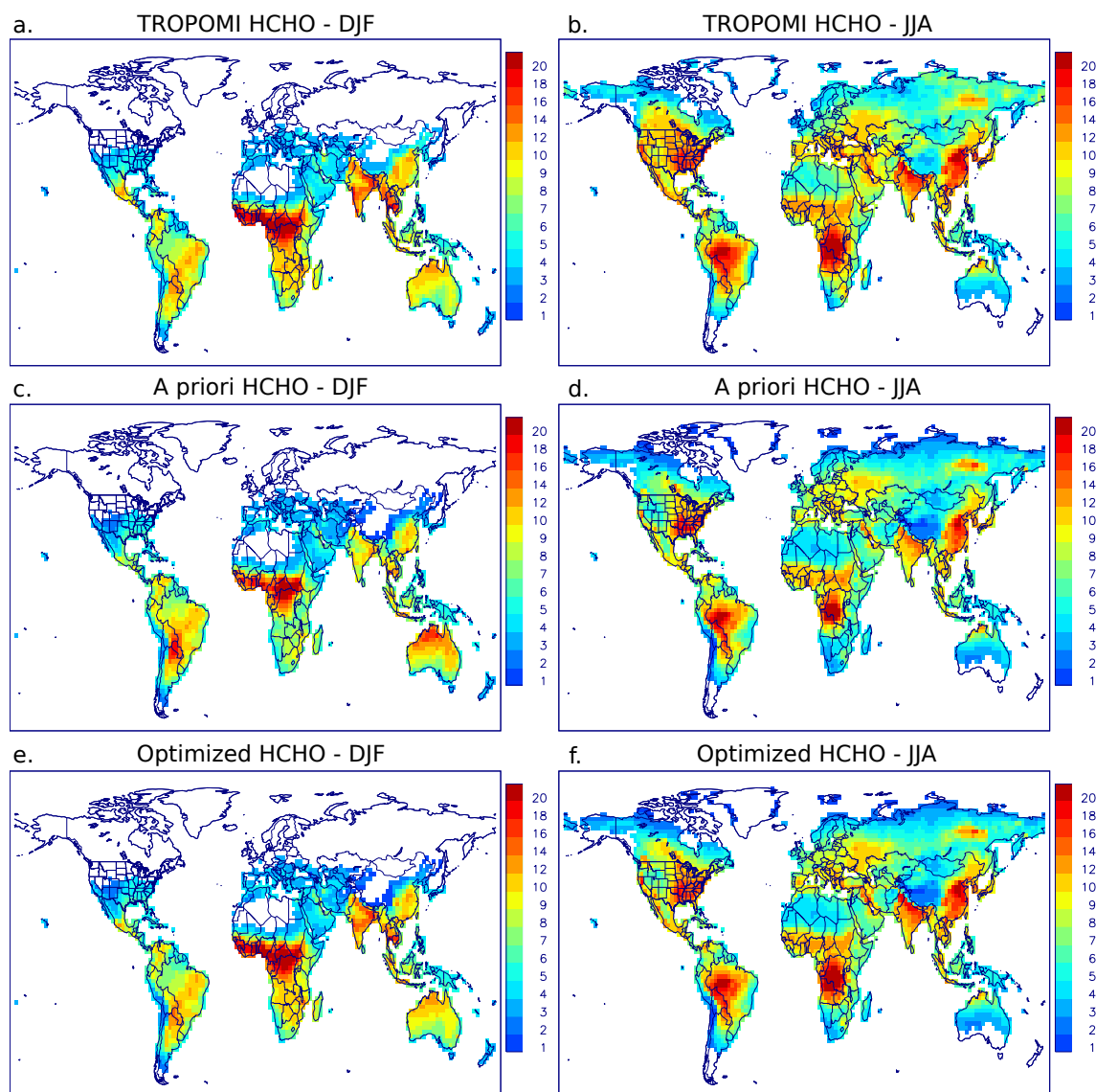
Figure 1. HCHO columns averaged over December, January, February (DJF) and June, July, August (JJA) in 2021 ( 10^{15} molec. \text{cm}^{-2} ). (a, b): TROPOMI bias-corrected columns. (c, d): Columns from a priori model. (e, f): Columns optimized through the inversion constrained by TROPOMI HCHO columns (OPHCHO).
