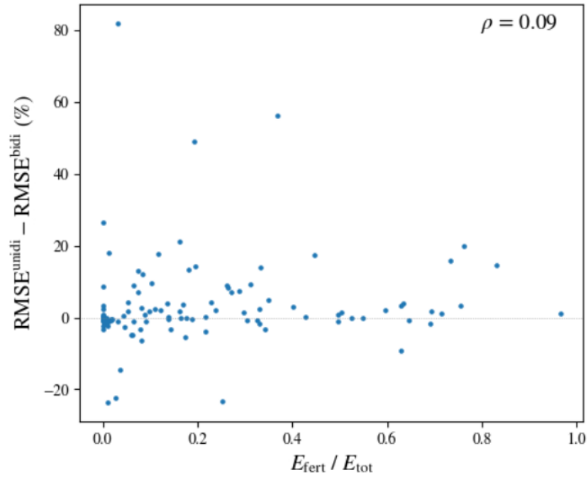
Scatterplot RMSE differences as a function of fraction of fertilizer emissions.
