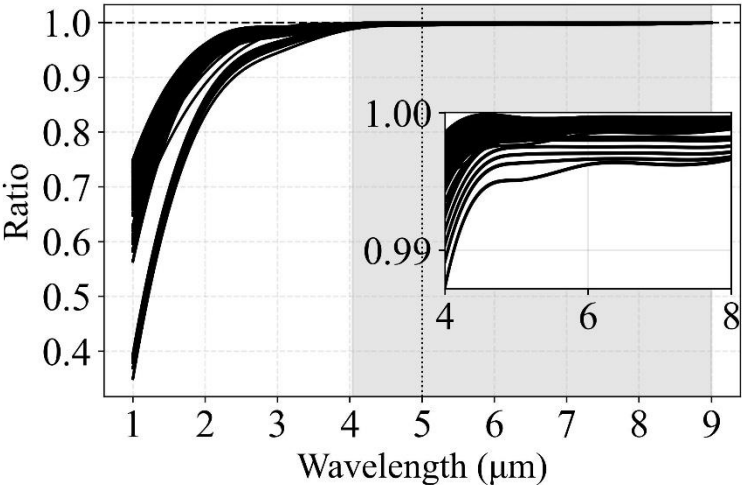
Figure 2: Ratio of spectral irradiance at each wavelength to the total spectral irradiance, illustrating the cumulative contribution of different wavelengths and different conditions typical of Davos. The grey shaded area represents the spectral interval contributing more than 98% of the total solar irradiance (TSI). The vertical dotted line marks the maximum upper limit of wavelength adopted for the study. The horizontal line at 1 represents the normalized maximum contribution of shortwave solar radiation. The inset highlights the long-wavelength region (4–8 μm), where the residual contribution becomes negligible.
