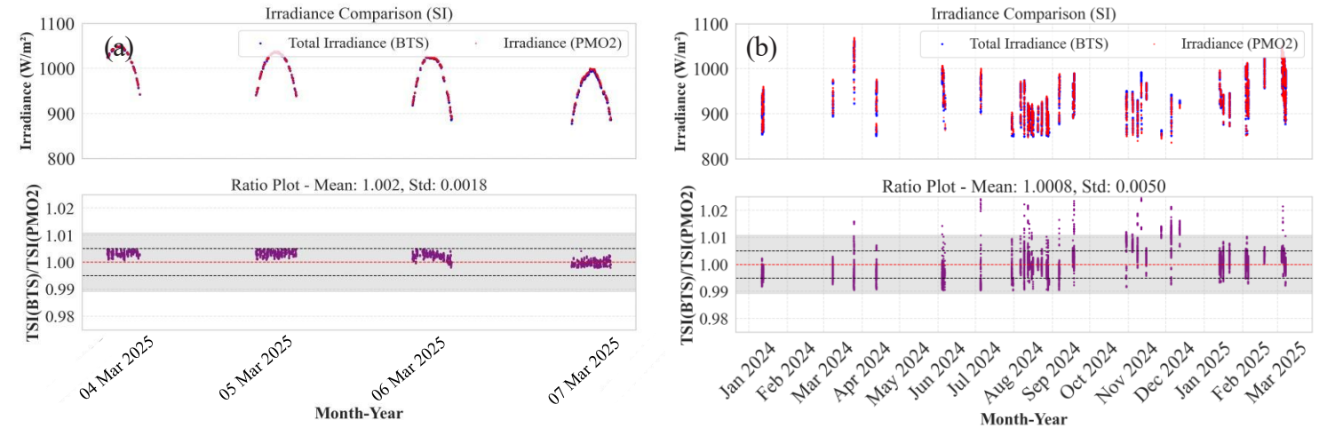
Figure 6: Top panel shows the time series of total solar irradiance (TSI) measurements obtained from the BTS spectroradiometer and the cavity radiometer (PMO2). Bottom panels display the ratio between the TSI measurements from both instruments. The grey shaded region represents the combined uncertainty of the BTS spectroradiometer, the extended region of the spectrum (2150 to 5000nm) and PMO2 measurements, with the red line indicating the degree of agreement between the two instruments. The black dashed lines mark the \pm 0.5\% bounds which is the standard deviation. Panel (a) illustrates traceability to SI during 4 th March 2025 to 7 th March 2025, while (b) presents SI traceability for the full analysis period from January 2024 to March 2025.
