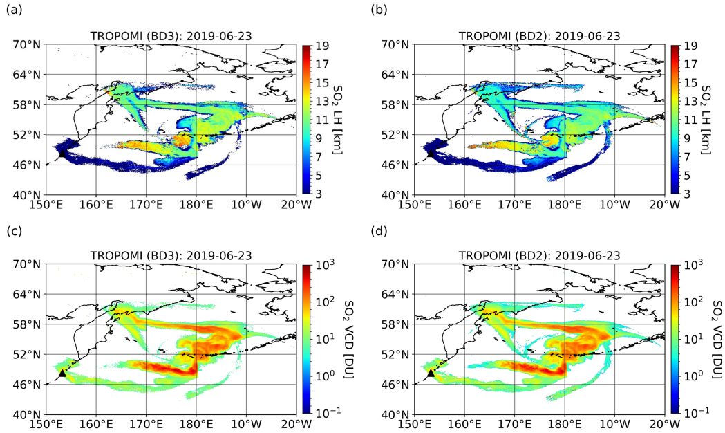
Figure 8. Sulfur dioxide retrievals from TROPOMI UV measurements on 23 June 2019 for the Raikoke eruption (see Table 4). Panels (a) and (b) show the SO 2 LRs retrieved using BD3 (310–326 nm) and BD2 (305–326 nm), respectively. Panels (c) and (d) display the corresponding SO 2 VCDs. The volcano location is marked by a black triangle.
