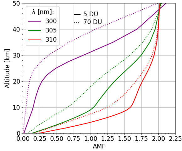
Figure B1. SO 2 AMF distributions as a function of the altitude, for different wavelengths and SO 2 VCDs.
