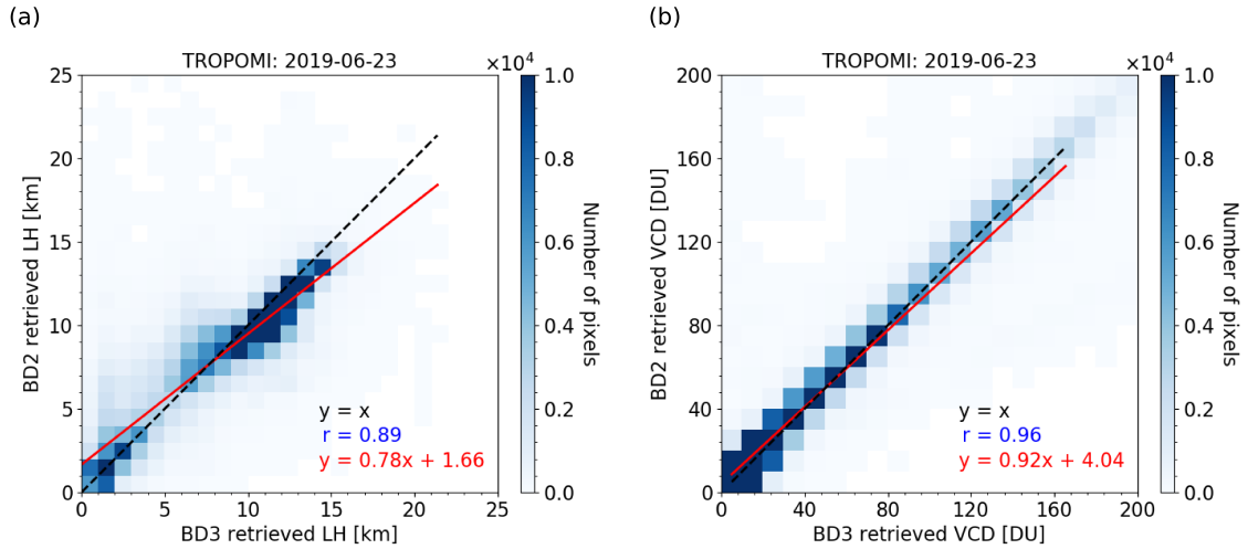
Figure 9. SO 2 LRs per 1 km 2 bin (a) and VCDs per 10 DU 2 bin (b) retrieved from TROPOMI BD3 (310–326 nm) and BD2 (305–326 nm) measurements on 23 June 2019 for the Raikoke eruption (see Table 4). Each plot includes the 1:1 line ( y = x ), the correlation coefficient ( r ), and the linear fit ( y = ax + b ).
