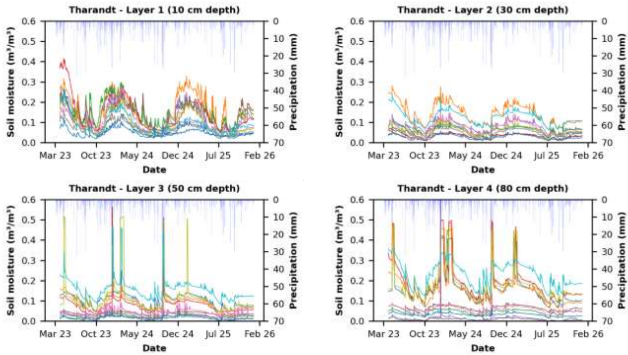
Figure 5 Observed soil moisture at Tharandt plot - Layer 1, 10 cm, Layer 2, 30 cm, Layer 3, 50 cm and Layer 4, 80 cm, each line represents the soil moisture of one of the 11 profiles, soil moisture raw measurements; no correction for potential sensor spikes or artefacts was performed.
