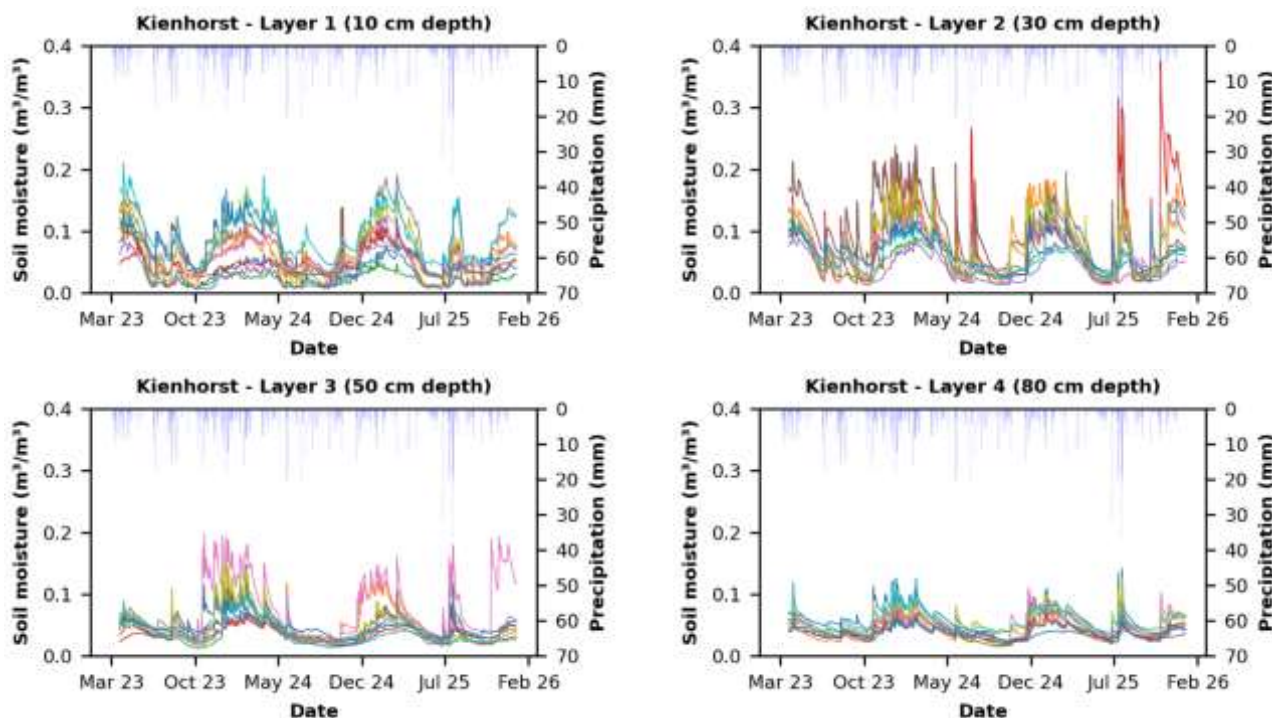
Figure 4 Observed soil moisture at Kienhorst plot – Layer 1, 10 cm, Layer 2, 30 cm, Layer 3, 50 cm and Layer 4, 80 cm, each line represents the soil moisture of one of the 11 profiles, soil moisture raw measurements; no correction for potential sensor spikes or artefacts was performed.
