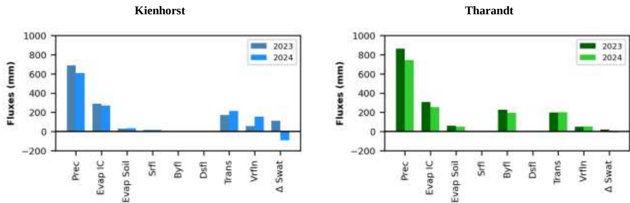
Figure 14 Calculated water balance components based on the mean model parameterisation of the individual 11 profiles for Kienhorst and Tharandt plot – Prec = precipitation, Evap IC = interception evaporation, Evap soil = soil evaporation, Srfl = surface runoff, Byfl = bypass flow, Dsfl = lateral or downslope movement of matric water to streamflow, Trans = transpiration, Vrfln = vertical drainage to groundwater, Gwfl = discharge of groundwater to streamflow, Δ Swat = change of soil water storage
