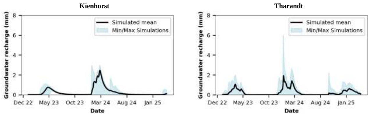
Figure 12 Simulated time series of daily groundwater recharge based on model parameterisation of the individual 11 profiles for Kienhorst and Tharandt plot - mean as well as minimum and maximum values of the 30 best simulations exemplary for soil profile 1
