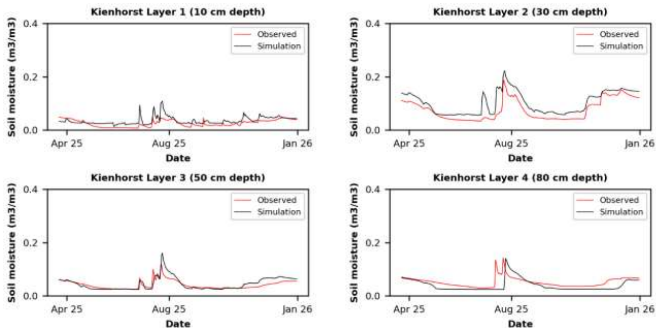
Figure 8 Soil moisture - Observed (red) versus simulated (black) based on the best parameter set of the 30 best simulatins during validation period exemplary for profile 1 at Kienhorst plot - Layer 1, 10 cm, Layer 2, 30 cm, Layer 3, 50 cm and Layer 4, 80 cm
