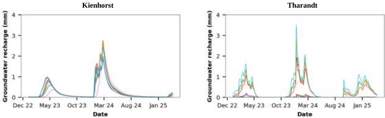
Figure 11 Simulated time series of daily groundwater recharge based on model parameterisation of the individual 11 profiles for Kienhorst and Tharandt plot - mean of the 30 best simulations per soil profile
