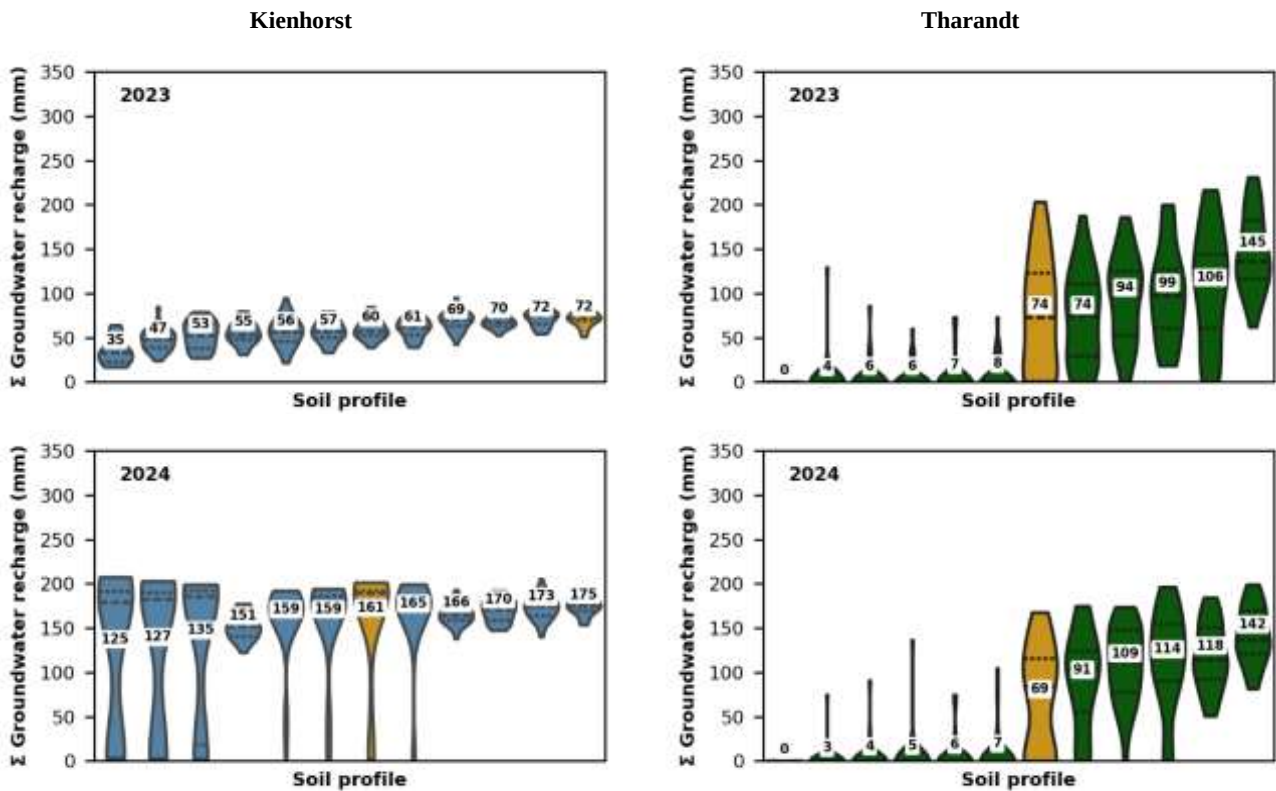
Figure 13 Calculated cumulative groundwater recharge volume ranges based on the parameter sets of the 30 best simulations for the individual 11 soil profiles (blue/green) as well the average value given as a number for each profile - separated for 2023 (upper figures) and 2024 (lower figures) at Kienhorst and Tharandt plot, furthermore the calculated cumulative groundwater recharge volume ranges based on the parameter sets of the 30 best simulations for the mean value of the 11 soil profiles (orange), the violins display the upper bound as the third quartile (75th percentile), the lower bound as the first quartile (25th percentile) as well as the median, the outer edges of the violin extend to the actual minimum and maximum values of the data.
