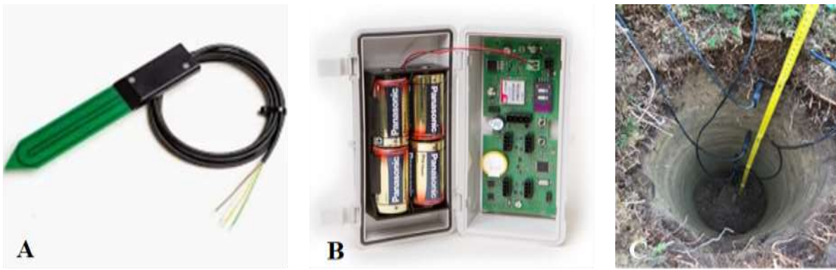
165 Figure 2 SMT100 Sensor (Truebner Company)(A), Datalogger TrueLog200 (Truebner Company)(B), soil profile with installed sensors 170 (photograph by Fichtner, 2023) (C)
