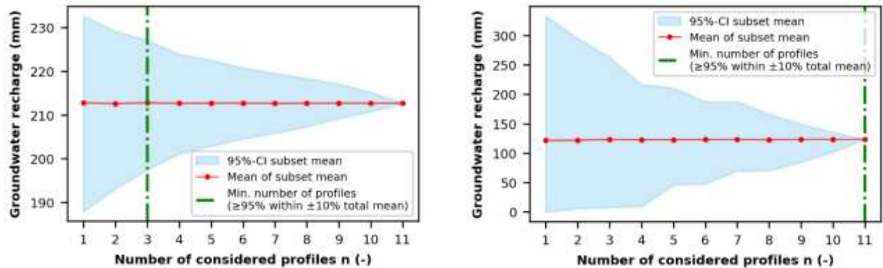
Figure 15 Results of the Monte-Carlo subsampling based on 330 the randomly drawn groundwater recharge subsets for Kienhorst and Tharandt plot - the blue band shows the 95% confidence interval of the subset means, the red line represents the average subset mean for each sample size and the green vertical line marks the minimum number of soil profiles required for 95% of all subset means to fall within \pm 10\% of the overall mean.
