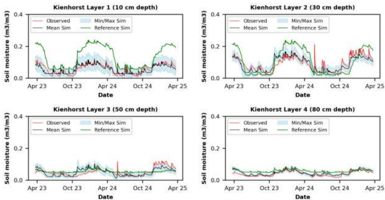
Figure 6 Soil moisture - Observed (red) versus reference simulation (green) as well as average of the 30 best calibrated simulations (black) and their uncertainty bandwidth (blue) exemplary for soil profile 2 at Kienhorst plot - Layer 1, 10 cm, Layer 2, 30 cm, Layer 3, 50 cm and Layer 4, 80 cm
