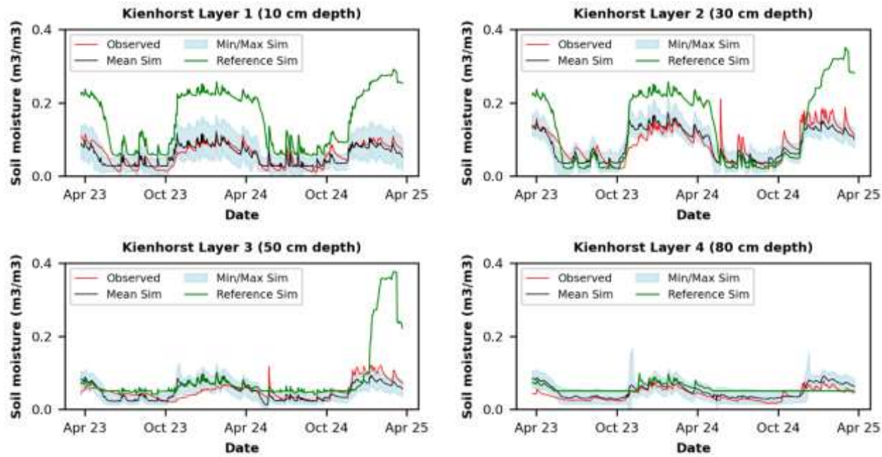
360 Figure 6 Soil moisture - Observed (red) versus reference simulation (green) as well as average of the 30 best calibrated simulations (black) and their uncertainty bandwidth (blue) exemplary for soil profile 2 at Kienhorst plot - Layer 1, 10 cm, Layer 2, 30 cm, Layer 3, 50 cm and Layer 4, 80 cm
