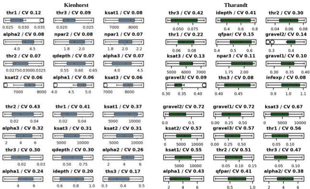
430 Figure 10 Parameter variation for the 12 parameters with the highest coefficient of variation for the Kienhorst and Tharandt plot – based on the average of calibrated parameter values derived from the 30 best simulations (upper figures) and based on the individual parameters of the 30 best simulations for soil profile 1 (lower figures)
