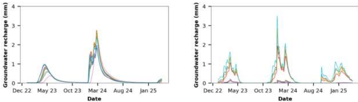
480 Figure 11 Simulated time series of daily groundwater recharge based on model parameterisation of the individual 11 profiles for Kienhorst and Tharandt plot - mean of the 30 best simulations per soil profile
