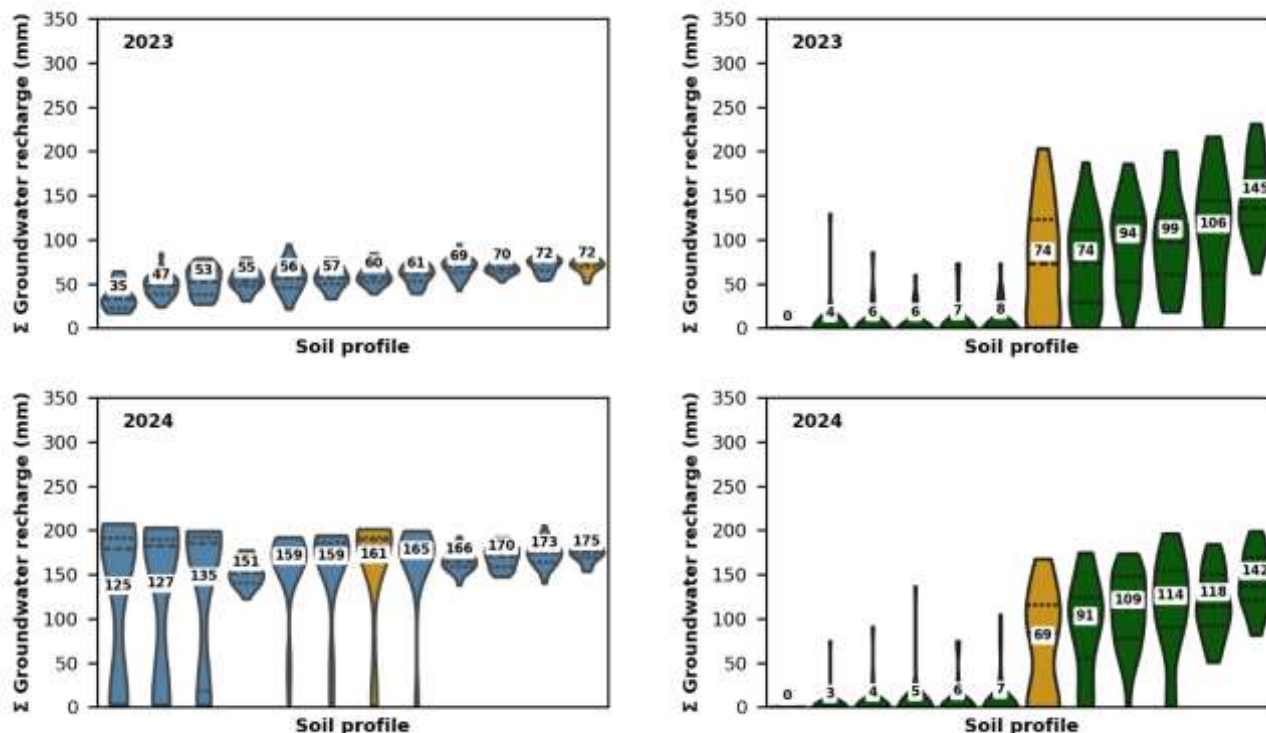
Figure 13 Calculated cumulative groundwater recharge volume ranges based on the parameter sets of the 30 best simulations for the individual 11 soil profiles (blue/green) as well the average value given as a number for each profile - separated for 2023 (upper figures) and 2024 (lower figures) at Kienhorst and Tharandt plot, furthermore the calculated cumulative groundwater recharge volume ranges based on the parameter sets of the 30 best simulations for the mean value of the 11 soil profiles (orange), the violins display the upper bound as the third quartile (75th percentile), the lower bound as the first quartile (25th percentile) as well as the median, the outer edges of the violin extend to the actual minimum and maximum values of the data.
