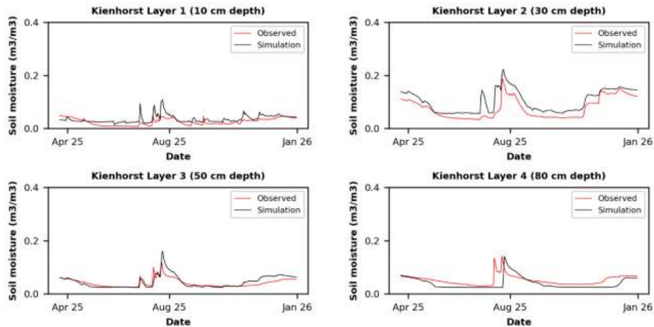
415 Figure 8 Soil moisture - Observed (red) versus simulated (black) based on the best parameter set of the 30 best simulatins during validation period exemplary for profile 1 at Kienhorst plot - Layer 1, 10 cm, Layer 2, 30 cm, Layer 3, 50 cm and Layer 4, 80 cm
