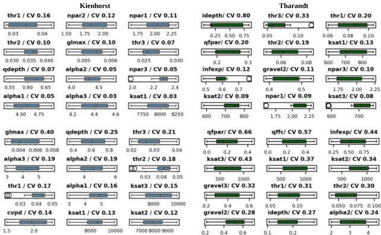
Figure 10 Parameter variation for the 12 parameters with the highest coefficient of variation for the Kienhorst and Tharandt plot – based on the average of calibrated parameter values derived from the 30 best simulations (upper figures) and based on the individual parameters of the 30 best simulations for soil profile 1 (lower figures)
