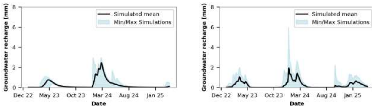
500 Figure 12 Simulated time series of daily groundwater recharge based on model parameterisation of the individual 11 profiles for Kienhorst and Tharandt plot - mean as well as minimum and maximum values of the 30 best simulations exemplary for soil profile 1
