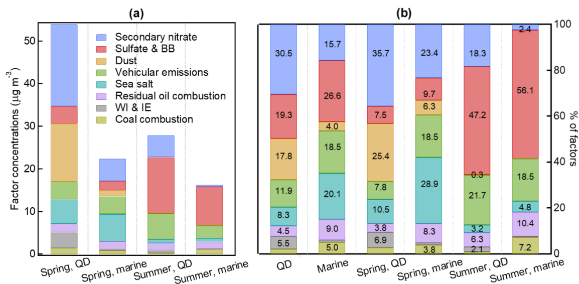
Figure 5: The averaged (a) concentrations and (b) relative percentage contributions of identified source factors to PM 2.5 as determined by PMF analysis. Sulfate & BB refers to sulfate & biomass burning. WI & IE denotes waste incineration & industrial emissions. “marine” refers to the BS and YS.
