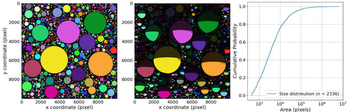
Figure 2. Example of a noise-free, shadowed, and colored synthetic test scene with n = 2336 pebbles. The parameters for generating this scene are: r_{min} = 12 ; r_{max} = 1500 ; \sigma = 0 . The size distribution of the pebbles is shown on the right and is highly skewed.
