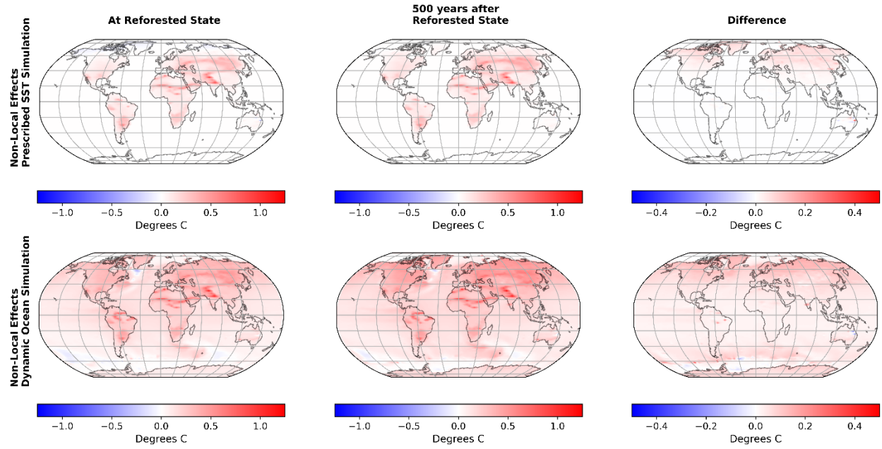
Figure A12: Non-local effects of reforestation of 25% of grid cells on surface temperature ( T_{\text{surf\_land}} and SST) when the Reforested State is reached (left panels), 500 years following the reach of the Reforested State (middle panels), and difference between these two timesteps (right panels) in the Prescribed SST Simulation and in the Dynamic
