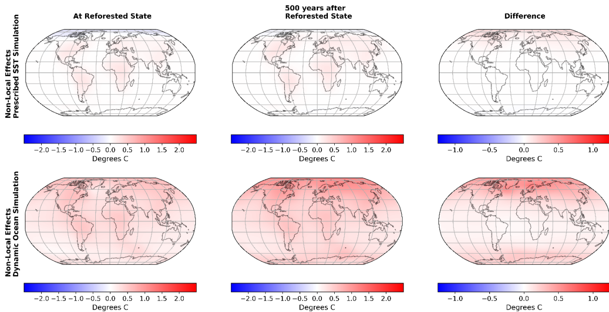
Figure A11: Non-local effects of reforestation of 50% of grid cells on Surface Air Temperature ( T_{air} ) when the Reforested State is reached (left panels), 500 years following the reach of the Reforested State (middle panels), and difference between these two timesteps (right panels) in the Prescribed SST Simulation and in the Dynamic Ocean Simulation. Note the difference in color scale between the maps.
