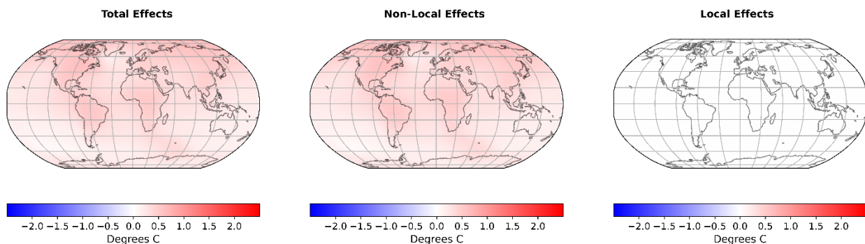
510 Figure A4: Total, non-local, and local biogeophysical effects of reforestation of 50% of grid cells on Surface Air Temperature ( T_{air} ) when the Reforested State is reached in the Dynamic Ocean Simulation. Due to the single-layer energy-moisture balance model of the atmosphere, heat is efficiently transported between neighboring grid cells via
