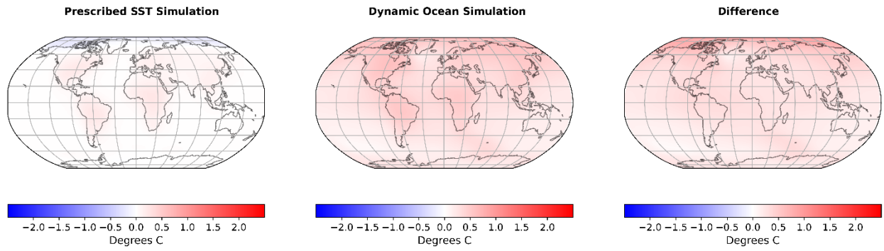
Figure A7: Non-local biogeophysical effects of reforestation of 50% of grid cells on Surface Air Temperature ( T_{air} ) when the Reforested State is reached in the Prescribed SST Simulation and in the Dynamic Ocean Simulation, and 530 difference between the non-local effects of these two simulations.
