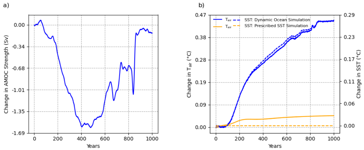
Figure A10: a) Change in the strength of the meridional overturning circulation following reforestation of 50% of grid cells b) Change in Surface Air Temperature ( T_{air} ) and SST over time following reforestation of 50% of grid cells in the Dynamic Ocean Simulation (blue) and in the Prescribed SST Simulation (orange).
