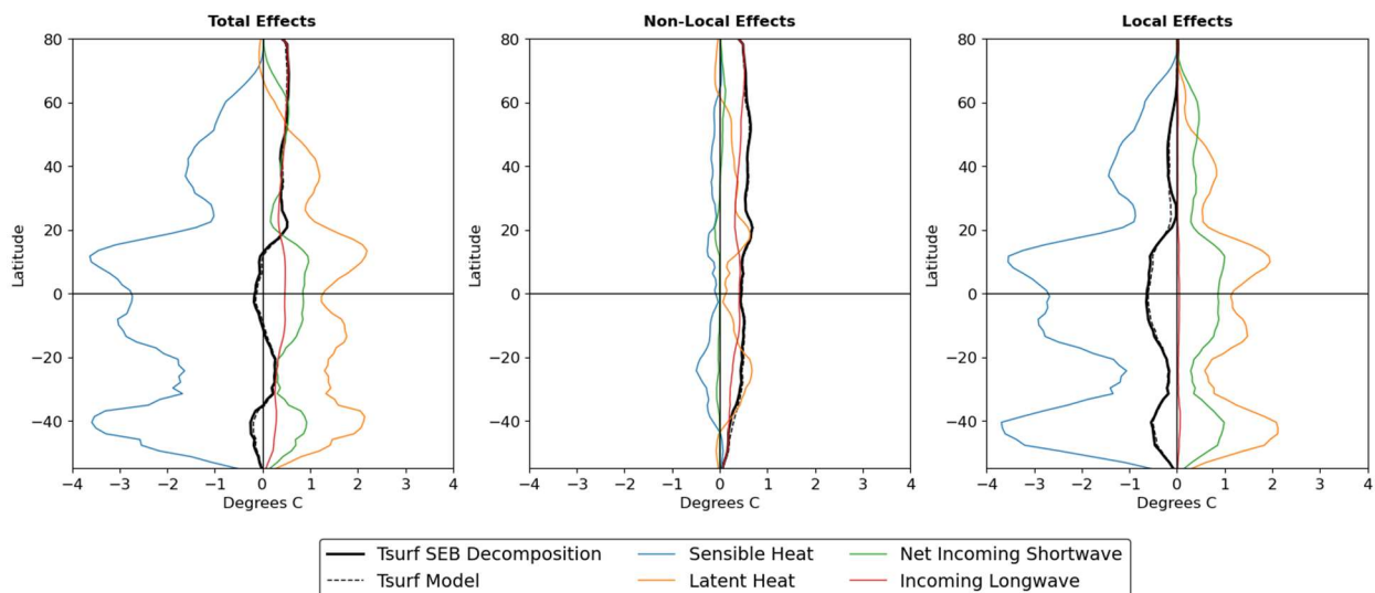
Figure 3: Surface Energy Balance decomposition of total, non-local, and local biogeophysical effects over land
