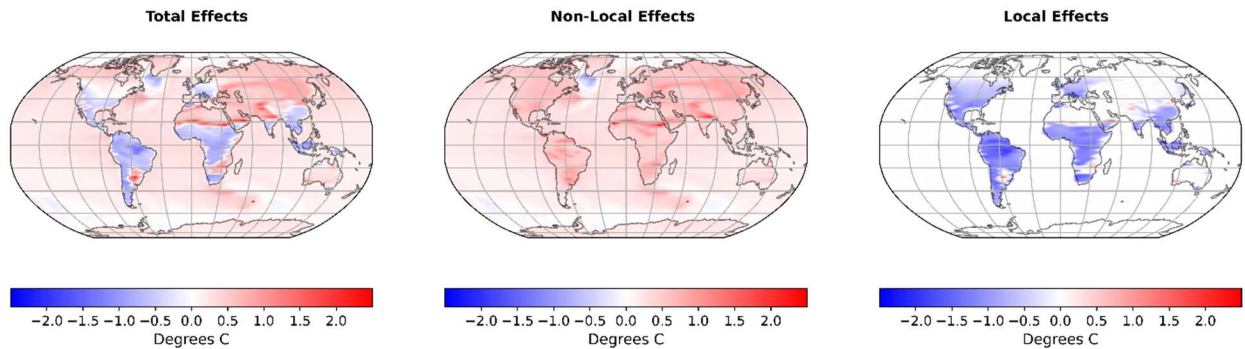
Figure 2: Total, non-local, and local biogeophysical effects of reforestation of 50% of grid cells on surface temperature ( T_{surf\_land} and SST) when the Reforested State is reached in the Dynamic Ocean Simulation. Maps of
