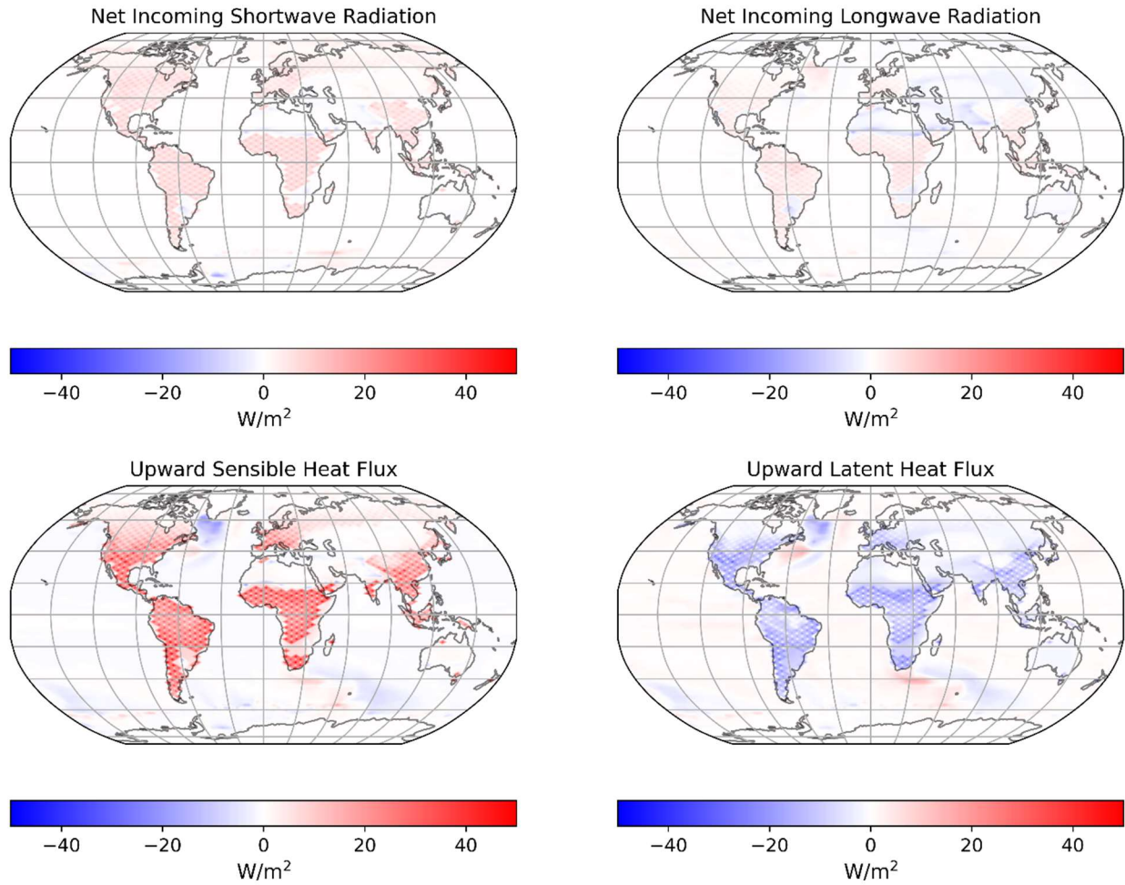
505 Figure A3: Change in net incoming shortwave radiation, net incoming longwave radiation, upward sensible heat flux and upward latent heat flux between the end of the Deforestation Simulation and when the Reforested State is reached in the Dynamic Ocean Simulation, following reforestation of 50% of grid cells.
