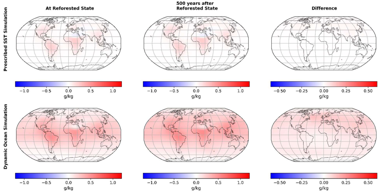
Figure A5: Change in surface specific humidity in g/kg after reforestation of 50% of grid cells when the Reforested State is reached (left panels), 500 years following the reach of the Reforested State (middle panels), and difference between these two timesteps (right panels) in the Prescribed SST Simulation and in the Dynamic Ocean Simulation. Note the difference in color scale between the maps.
