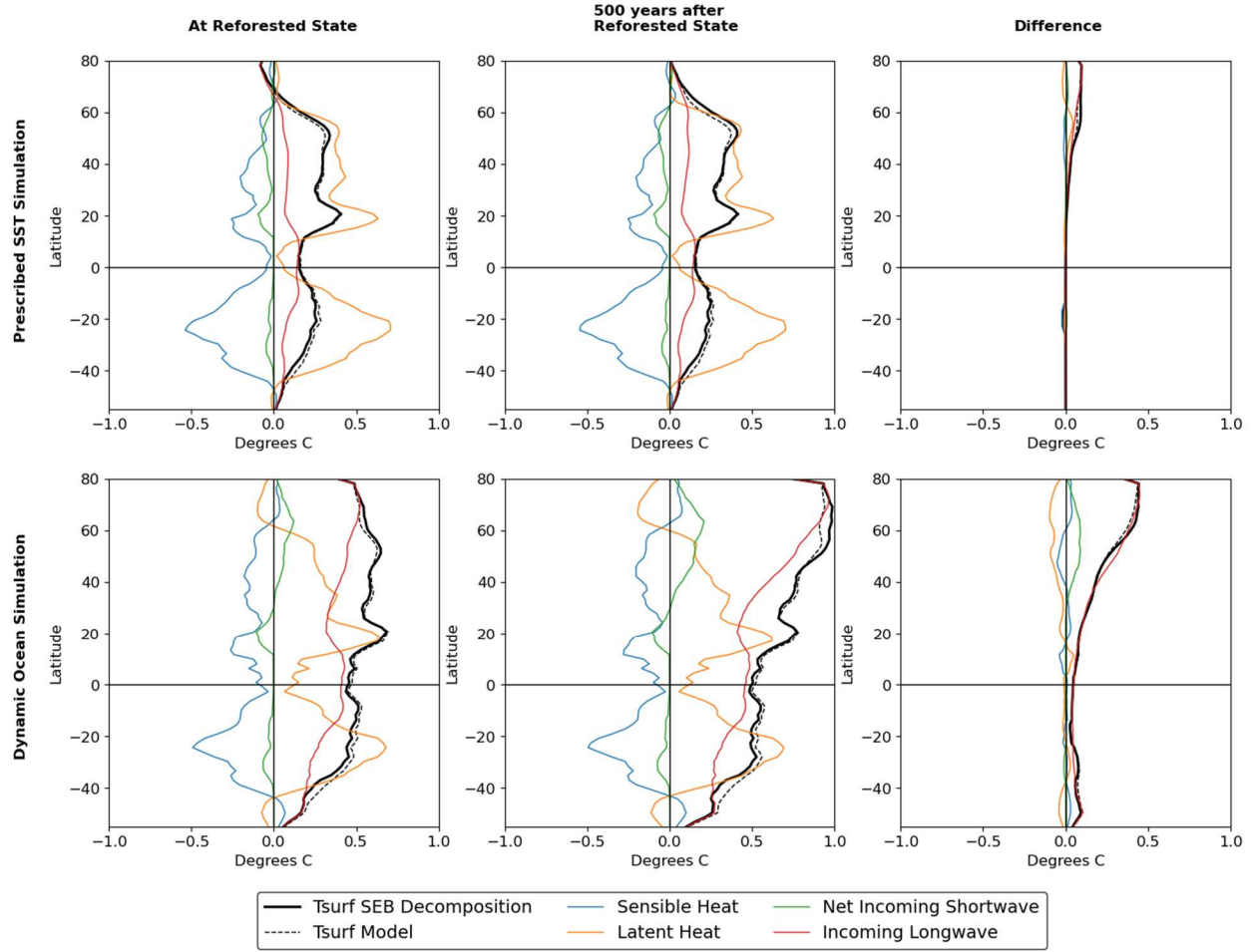
Figure 7: Surface Energy Balance decomposition of the non-local biogeophysical effects over land after reforestation of 50% of grid cells when the Reforested State is reached (left panels), 500 years following the reach of the Reforested State (middle panels), and difference between the two surface energy balance decompositions (right panels), for both the Prescribed SST Simulation and the Dynamic Ocean Simulation.
