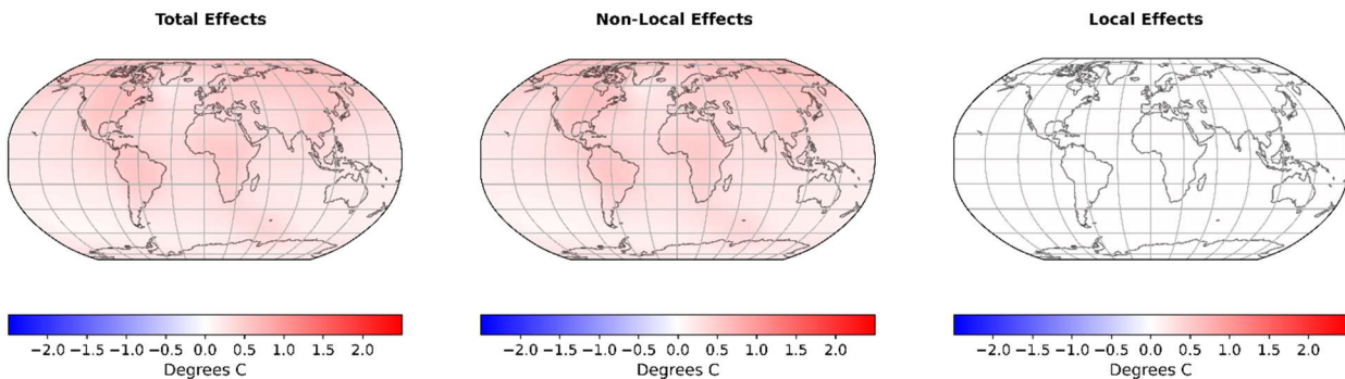
510 Figure A4: Total, non-local, and local biogeophysical effects of reforestation of 50% of grid cells on Surface Air Temperature ( T_{\text{air}} ) when the Reforested State is reached in the Dynamic Ocean Simulation. Due to the single-layer energy-moisture balance model of the atmosphere, heat is efficiently transported between neighboring grid cells via
