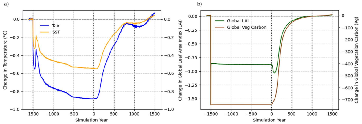
Figure A1: a) Change in T_{air} and SST from the initial spin-up when 100% of grid cells are deforested at simulation year -1500 and subsequently reforested at year 0. b) Change in global Leaf Area Index (combined for all PFTs) and global vegetation carbon (combined for all PFTs) from the initial spin-up when 100% of grid cells are deforested at simulation year -1500 and subsequently reforested at year 0. Year 500 refers to the Reforested State, when the growth of PFTs is stabilizing and vegetation has almost recovered to its pre-deforestation state.
