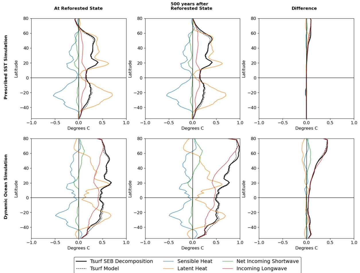
Figure 7: Surface Energy Balance decomposition of the non-local biogeophysical effects over land after
