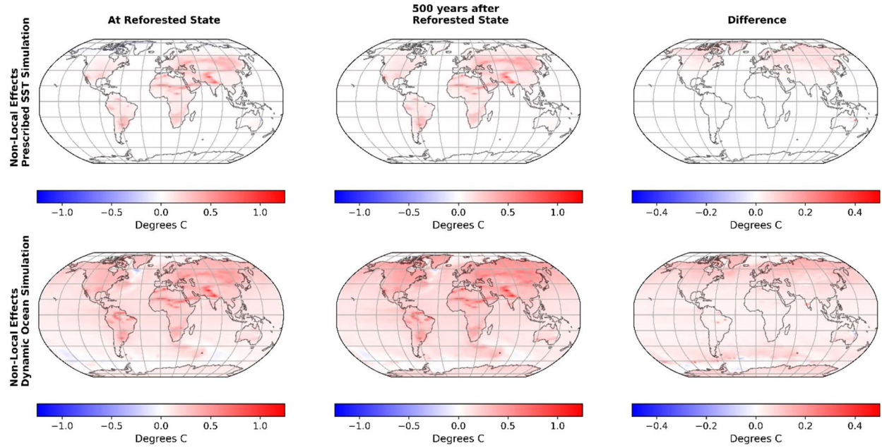
Figure A12: Non-local effects of reforestation of 25% of grid cells on surface temperature ( T_{\text{surf\_land}} and SST) when the Reforested State is reached (left panels), 500 years following the reach of the Reforested State (middle panels), and difference between these two timesteps (right panels) in the Prescribed SST Simulation and in the Dynamic Ocean Simulation. Note the difference in color scale between the maps.
