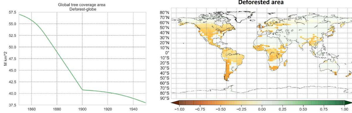
Figure B1: Change in global tree coverage area between 1850 and 1950 in the deforest-glob experiment in the UVic ESCM (left panel) and fraction of grid cell deforested by 1950 (right panel).
