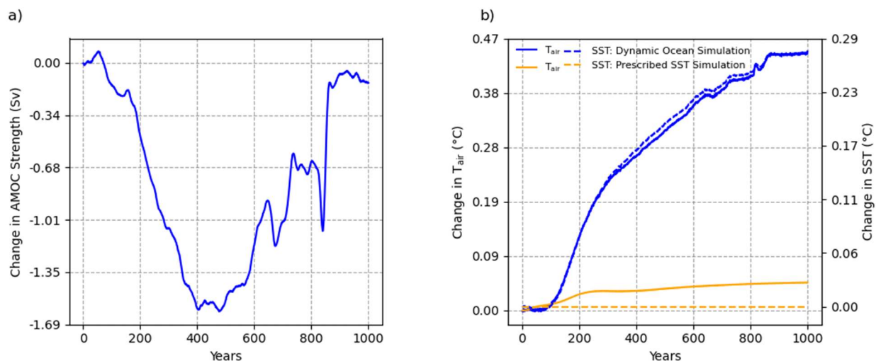
Figure A10: a) Change in the strength of the meridional overturning circulation following reforestation of 50% of grid cells b) Change in Surface Air Temperature ( T_{\text{air}} ) and SST over time following reforestation of 50% of grid cells in the Dynamic Ocean Simulation (blue) and in the Prescribed SST Simulation (orange).
