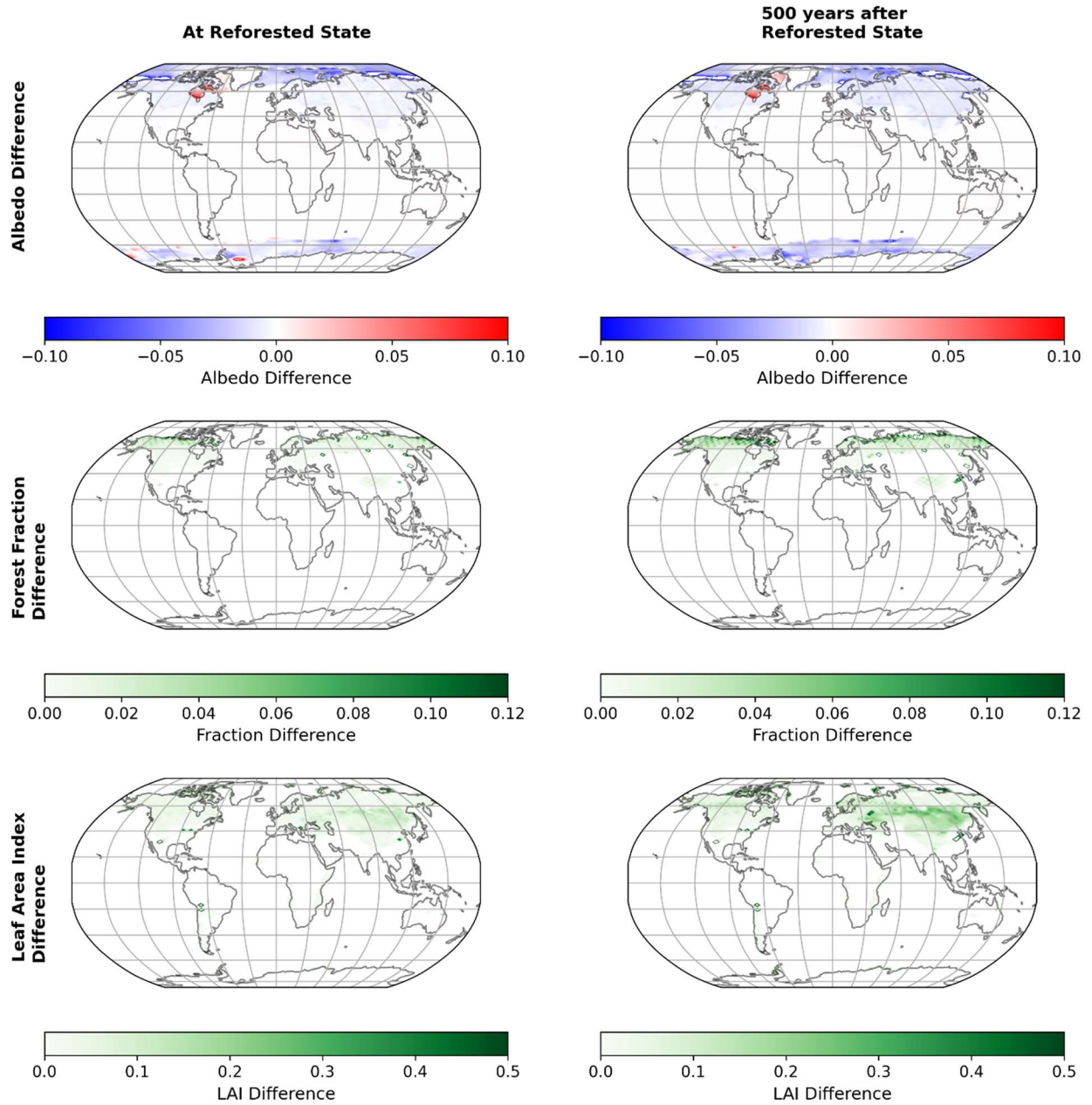
Figure A9: Difference between the Dynamic Ocean Simulation and the Prescribed SST Simulation in albedo, fraction of grid cell covered by forest (shrubs, broadleaf trees, and needleleaf trees), and LAI for all PFTs combined, when the Reforested State is reached and 500 years following the reach of the Reforested State.
