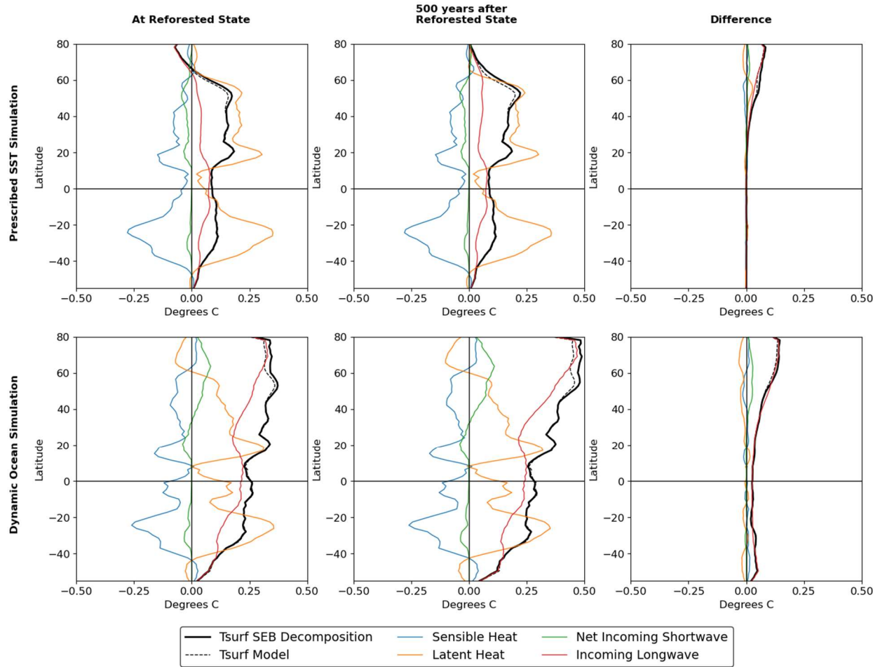
Figure A13: Surface Energy Balance decomposition of the non-local biogeophysical effects over land after reforestation of 25% of grid cells when the Reforested State is reached (left panels), 500 years following the reach of the Reforested State (middle panels), and difference between the two surface energy balance decompositions (right panels), for both the Prescribed SST Simulation and the Dynamic Ocean Simulation.
