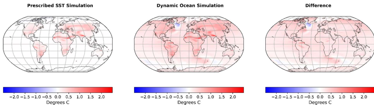
Figure 4: Non-local biogeophysical effects of reforestation of 50% of grid cells on surface temperature ( T_{\text{surf\_land}} and SST) when the Reforested State is reached in the Prescribed SST Simulation and in the Dynamic Ocean Simulation, and difference between the non-local effects of these two simulations (Dynamic Ocean Simulation minus Prescribed SST Simulation).
