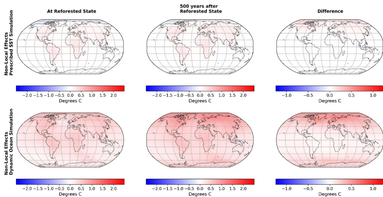
Figure A11: Non-local effects of reforestation of 50% of grid cells on Surface Air Temperature ( T_{\text{air}} ) when the Reforested State is reached (left panels), 500 years following the reach of the Reforested State (middle panels), and difference between these two timesteps (right panels) in the Prescribed SST Simulation and in the Dynamic Ocean Simulation. Note the difference in color scale between the maps.
