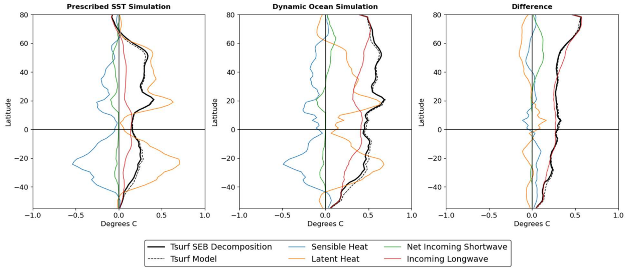
Figure 5: Surface Energy Balance Decomposition of non-local biogeophysical effects over land after reforestation of 50% of grid cells when the Reforested State is reached in the Prescribed SST Simulation and in the Dynamic Ocean Simulation, and difference between the two surface energy balance decompositions (Dynamic Ocean Simulation minus Prescribed SST Simulation).
