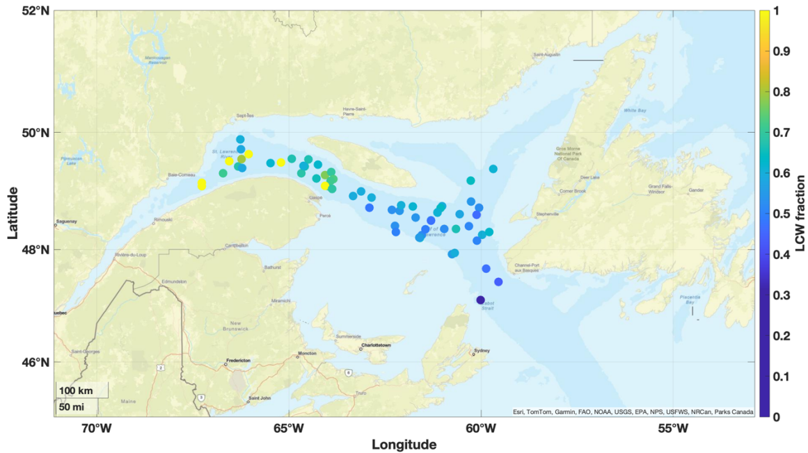
Figure 5: LCW fraction on the \sigma_\theta = 27.26 \text{ kg/m}^3 isopycnal deep water in the Laurentian Channel calculated using the linear fraction model with \theta , S_p and mean age ( \Gamma ) observations, plotted on a map. The endmembers used in the calculations are provided in Table 1 with all the data presented here being collected during the two TREx surveys in 2022.
