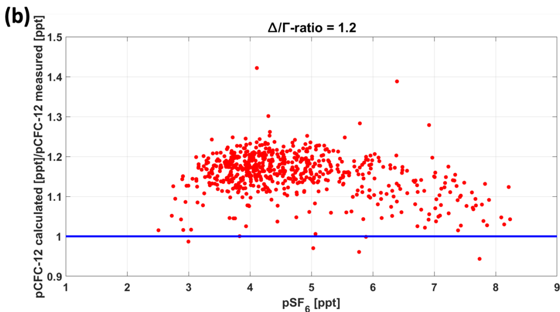
495 Figure B1: a) Comparison of calculated mean ages from CFC-12 and SF 6 with different \Delta/\Gamma -ratio. The saturations for each tracer were assumed to be time dependent. b) Display of the relationship between calculated and measured pCFC-12 against pSF 6 concentrations using a ratio of \Delta/\Gamma=1.2 for the calculations.
