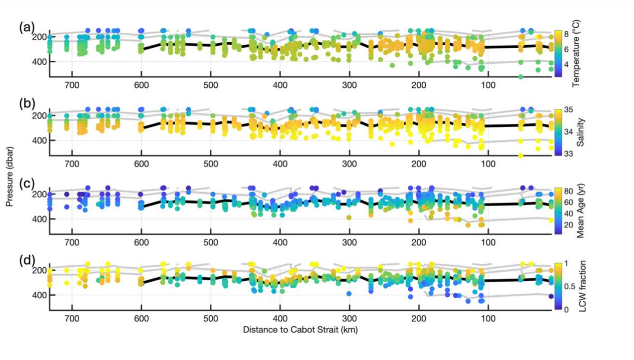
Figure 4: Display of (a) Temperature, (b) Salinity, (c) Mean age and (d) LCW fraction throughout the Laurentian Channel (shown as distance from Cabot Strait, calculated as described in Section 3.4, where greater distance corresponds to samples collected further toward the LSLE) versus depth. The LCW fractions here are calculated using the linear fraction model, with endmembers of all properties being the mean of each range. The black line indicates the \sigma_{\theta} = 27.26 \text{ kg/m}^3 isopycnal and grey lines represent the 26.5, 26.75, 27, and 27.5 isopycnals. (As a reference, the LSLE starts approximately at a distance of 600 km from Cabot Strait).
