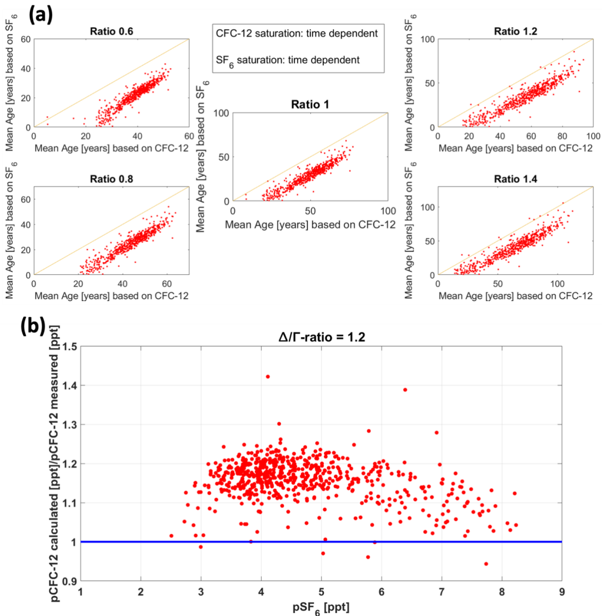
495 Figure B1: a) Comparison of calculated mean ages from CFC-12 and SF 6 with different \Delta/\Gamma -ratio. The saturations for each tracer were assumed to be time dependent. b) Display of the relationship between calculated and measured pCFC-12 against pSF 6 concentrations using a ratio of \Delta/\Gamma=1.2 for the calculations.
