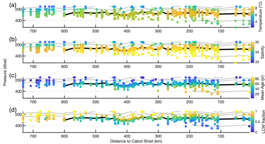
Figure 4: Display of (a) Temperature, (b) Salinity, (c) Mean age and (d) LCW fraction throughout the Laurentian Channel (shown as distance from Cabot Strait, calculated as described in Section 3.4, where greater distance corresponds to samples collected further toward the LSL) versus depth. The LCW fractions here are calculated using the linear fraction model, with endmembers of all properties being the mean of each range. The black line indicates the \sigma_\theta = 27.26 \text{ kg/m}^3 isopycnal and grey lines represent the 26.5, 26.75, 27, and 27.5 isopycnals. (As a reference, the LSL starts approximately at a distance of 600 km from Cabot Strait).
