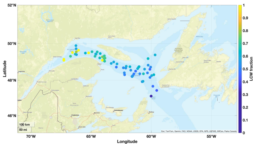
Figure 5: LCW fraction on the \sigma_{\theta} = 27.26 \text{ kg/m}^3 isopycnal deep water in the Laurentian Channel calculated using the linear fraction model with \theta , S_p and mean age ( T ) observations, plotted on a map. The endmembers used in the calculations are provided in Table 1 with all the data presented here being collected during the two TReX surveys in 2022.
