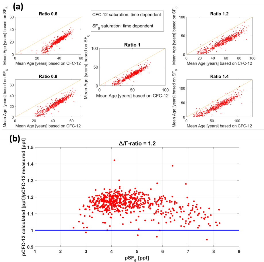
500 Figure B1: a) Comparison of calculated mean ages from CFC-12 and SF 6 with different \Delta/T -ratio. The saturations for each tracer were assumed to be time dependent. b) Display of the relationship between calculated and measured pCFC-12 against pSF 6 concentrations using a ratio of \Delta/T=1.2 for the calculations.
