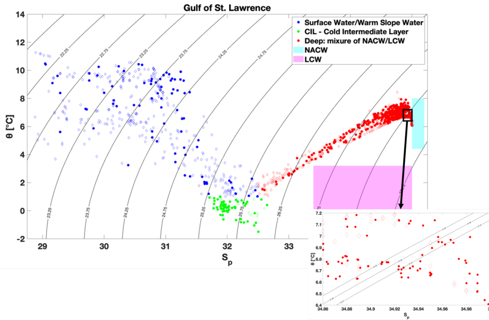
Figure 2: Potential Temperature ( \theta ) vs Practical Salinity ( S_p ) plot from the bottle data of the two cruises in 2022, showing the three main layers of the GSL, as indicated by different colors with density lines of \sigma_\theta (TRex 2 – dots; DFO's AZMP survey/TRex 4 – diamonds). The pink and the cyan areas represent the \theta vs S_p ranges of LCW and NACW, as defined in Jutras et al. (2020). In addition, a zoomed in area around the density of \sigma_\theta = 27.26 \text{ kg/m}^3 is shown, with density lines at 27.25, 27.26 and 27.27.
