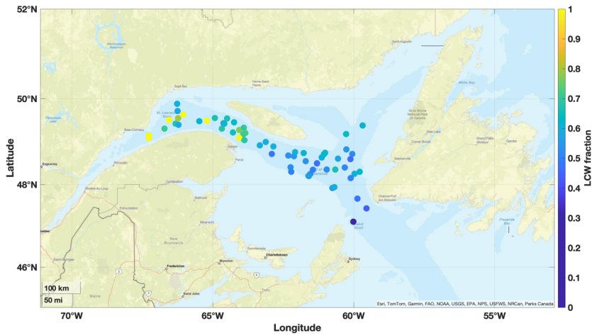
Figure 5: LCW fraction on the \sigma_\theta = 27.26 \text{ kg/m}^3 isopycnal deep water in the Laurentian Channel calculated using the linear fraction model with \theta , S_p and mean age ( T ) observations, plotted on a map. The endmembers used in the calculations are provided in Table I with all the data presented here being collected during the two TReX surveys in 2022.
