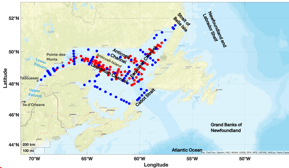
170 Figure 1: The Gulf of St. Lawrence, with its main Channels and Straits identified, together with the Lower and Upper Estuary. Sampling stations from the expeditions in June 2022 (TRex 2 – red dots) and November 2022 (DFO’s AZMP survey/TRex 4 – blue dots) are displayed.
