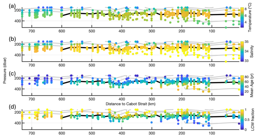
Figure 4: Display of (a) Temperature, (b) Salinity, (c) Mean age and (d) LCW fraction throughout the Laurentian Channel (shown as distance from Cabot Strait, calculated as described in Section 3.4, where greater distance corresponds to samples collected further toward the LSLE) versus depth. The LCW fractions here are calculated using the linear fraction model, with endmembers of all properties being the mean of each range. The black line indicates the \sigma_{\theta} = 27.26 \text{ kg/m}^3 isopycnal and grey lines represent the 26.5, 26.75, 27, and 27.5 isopycnals. (As a reference, the LSLE starts approximately at a distance of 600 km from Cabot Strait).
