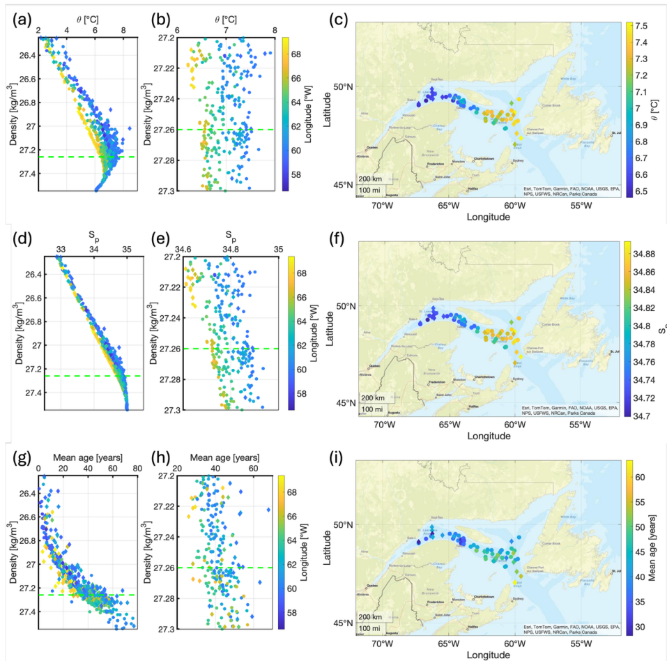
Figure 3: Potential Temperature (a), Practical Salinity (d), and Mean ages (g) measured within the deep-water layer in the GSL (density > 26.25 \text{ kg/m}^3 ), with the colorbar representing the longitude. Figures b, e, and h represent a zoomed in area around the \sigma_{\theta} = 27.26 \text{ kg/m}^3 isopycnal (green dotted line), respectively, and plots c, f, and i show the properties interpolated onto the 27.26 isopycnal from observations with densities between 27.25 and 27.27, mapped over the GSL. All the data presented here was collected during the two surveys in 2022, with the dots representing the measurements from TRex2 survey, and the diamonds the measurements from the DFO AZMP survey/TRex 4 cruise.
