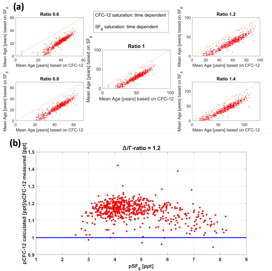
Figure B1: a) Comparison of calculated mean ages from CFC-12 and SF 6 with different \Delta T -ratio. The saturations for each tracer were assumed to be time dependent. b) Display of the relationship between calculated and measured pCFC-12 against pSF 6 concentrations using a ratio of \Delta T=1.2 for the calculations.
