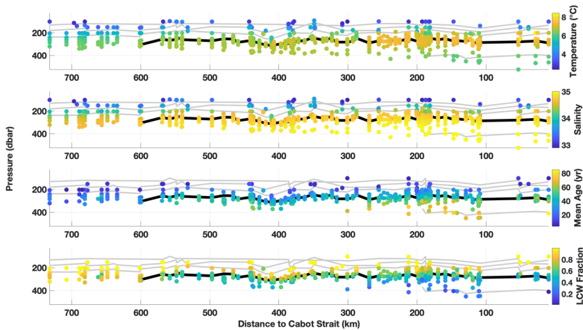
Figure 7. Display of Temperature, Salinity, Mean age and LCW fraction throughout the Laurentian Channel (shown as distance from Cabot Strait, where greater distance corresponds to locations further toward the LSLE) versus depth. The black line indicates the \sigma_{\theta} = 27.26 \text{ kg/m}^3 isopycnal and grey lines represent the 26.5, 26.75, 27, and 27.6 isopycnals. (As a reference, the LSLE starts approximately at a distance of 600 km from Cabot Strait).
