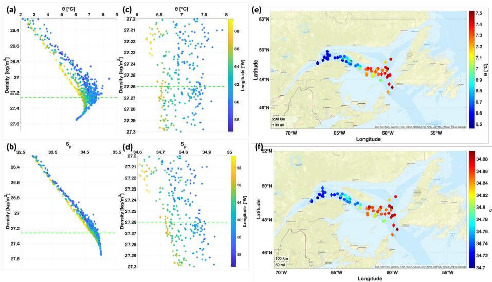
Figure 3: Potential Temperature (a) and Practical Salinity (b) measured within the deep-water layer in the GSL (density > 26.25 kg/m 3 ), with the colorbar representing the longitude. Figures c and d represent a zoomed in area around the \sigma_{\theta} = 27.26 kg/m 3 isopycnal (green dotted line) and plots e and f show these measurements plotted on a map of the GSL against longitude and latitude. All the data presented here was collected during the two surveys in 2022, with the dots represent the measurements from the earlier survey (TReX 2) and the diamonds the measurements from the later cruise (DFO's AZMP survey/TReX 4).
