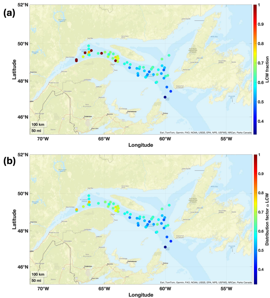
Figure 5: a) LCW fraction on the \sigma_{\theta} = 27.26 \text{ kg/m}^3 isopycnal deep water in the Laurentian Channel from 0, S_p and mean age ( T ) observations plotted on a map. The endmembers used in this calculation are provided in Table 1. b) LCW mixing factor on the \sigma_{\theta} = 27.26 \text{ kg/m}^3 isopycnal in the Laurentian Channel from the 2-IG-TTD analysis, using observed mean ages ( T ), plotted on a map of the GSL. All the data presented here was collected during the two TReX surveys in 2022.
