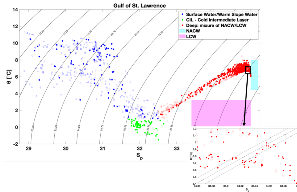
310 Figure 2: Potential Temperature ( \theta ) vs Practical Salinity ( S_p ) plot from the bottle data of the two cruises in 2022, showing the three main layers of the GSL, as indicated by different colors with density lines of \sigma_\theta (TRex 2 – dots; DFO's AZMP survey/TRex 4 – diamonds). The pink and the cyan areas represent the \theta vs S_p ranges of LCW and NACW, as defined in Jutras et al. (2020). In addition, a zoomed in area around the density of \sigma_\theta = 27.26 \text{ kg/m}^3 is shown, with density lines at 27.25, 27.26 and 27.27.
