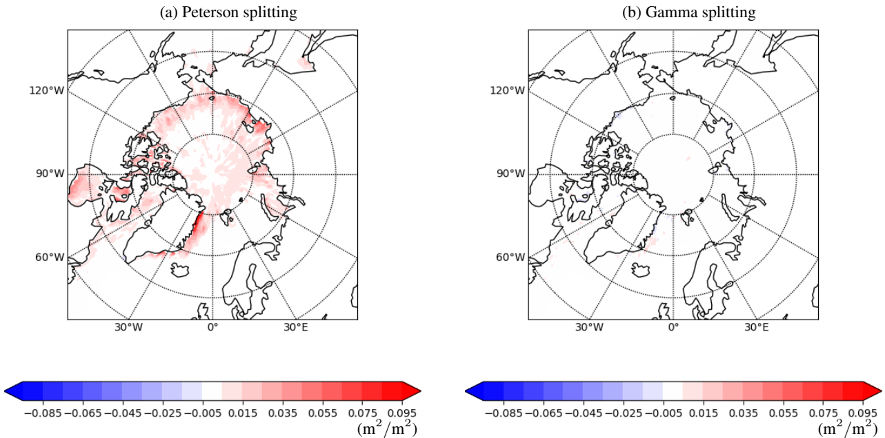
Figure 5. Errors in analysis of sea ice concentration comparing to ESA CCIv3 . Shown is the difference in RMSE using (a) the Peterson splitting, and (b) the Gamma splitting, compared to background splitting. In red are regions of worse sea ice concentration, which is notable across large areas of the Arctic domain when using Peterson splitting.
