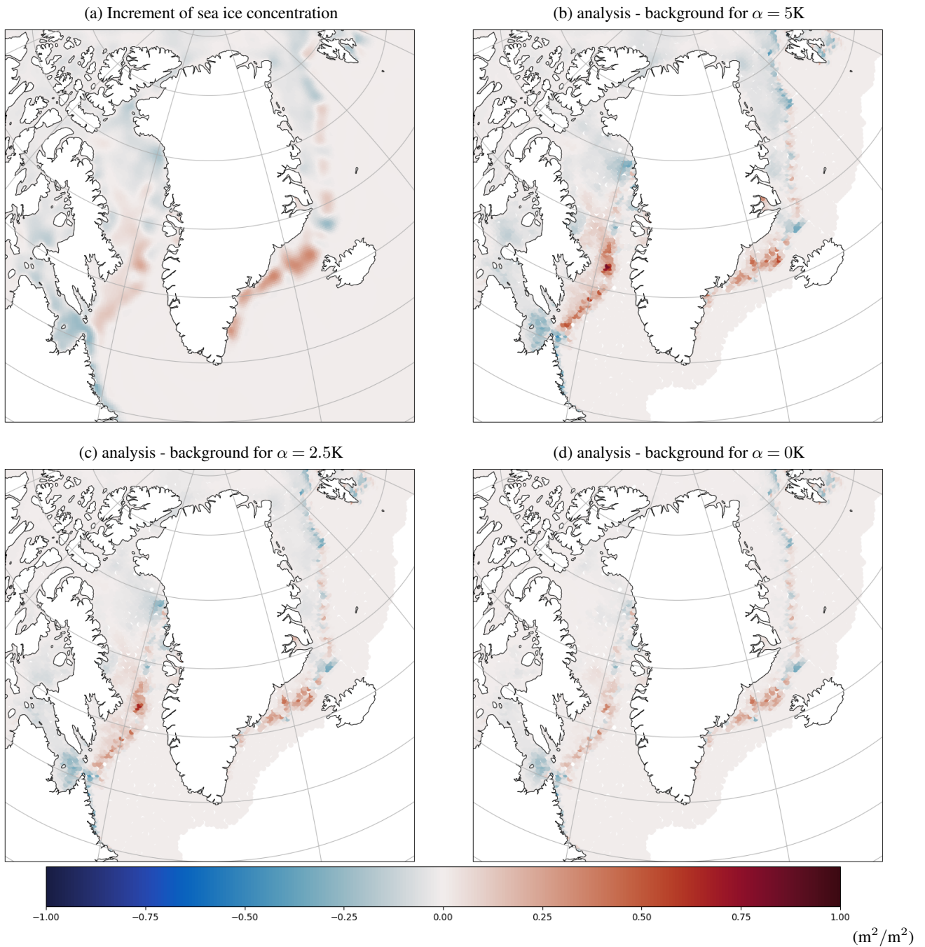
Figure 8. Greenland and Labrador Sea sea ice concentration increment and effective increments for various strengths of the ice induced temperature increment for the first analysis cycle 2010-01-01:2010-01-05
