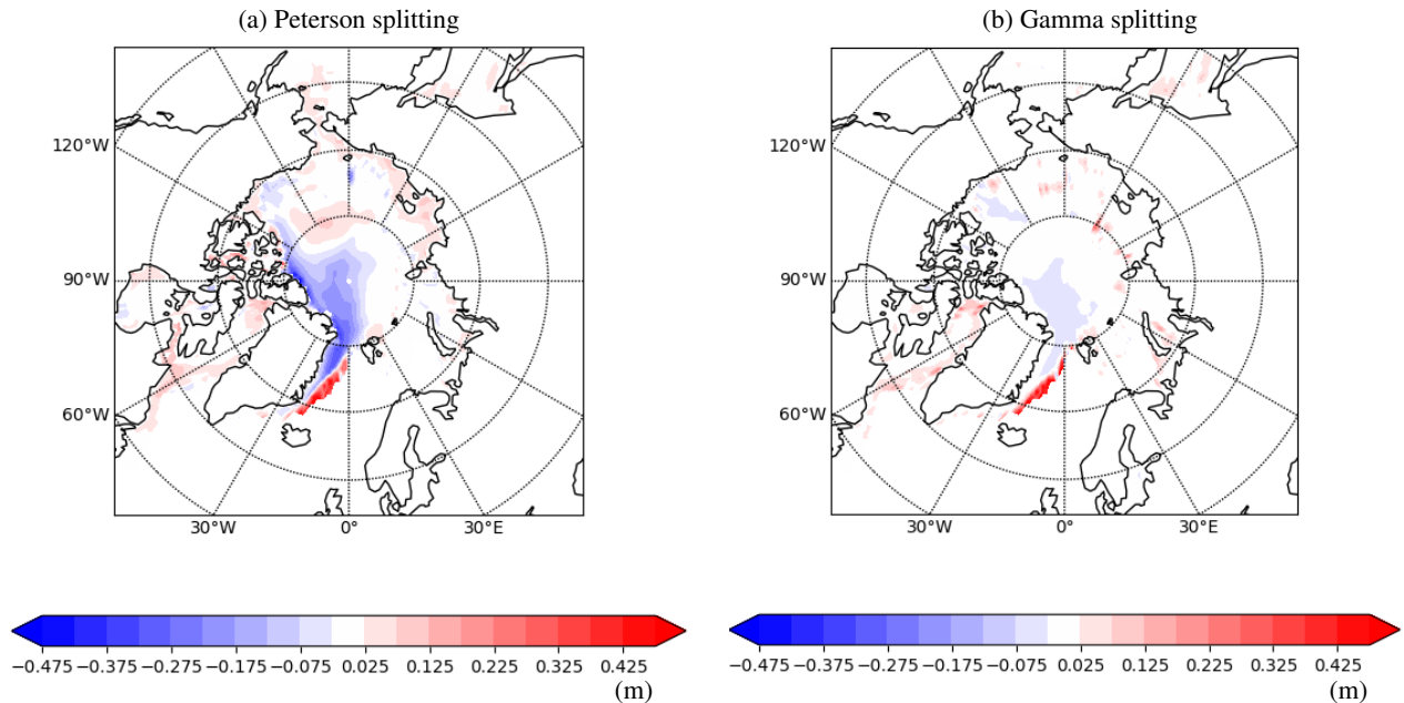
Figure 4. Errors in analysis of sea ice thickness comparing to CS2SMOS merged CryoSat-2 and SMOS ice thickness for the entire 2010–2014 experimental period. Shown is the difference in RMSE using (a) the Peterson splitting, and (b) the Gamma splitting, compared to background splitting. In red are regions of worse sea ice thickness, which is notable around the ice edge in the Atlantic.
