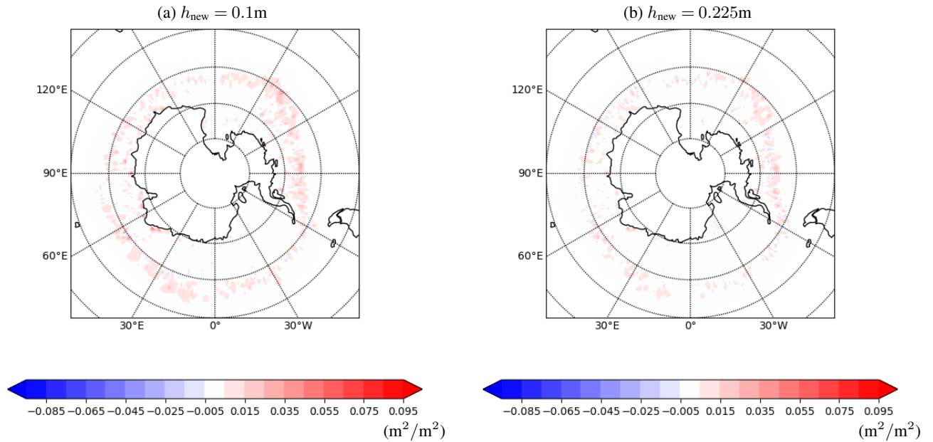
Figure 6. Southern hemisphere SIC o-b RMSE differences compared to using a thickness of new sea ice h_{\text{new}} = 0.45\text{m} for the entire 2010–2014 experimental period. Larger errors are seen around the ice edge when thinner ice is assumed to be missing at open water points.
