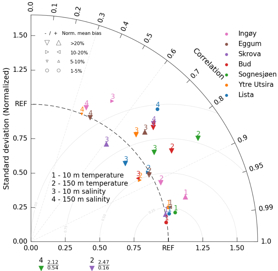
Figure 7. Temperature statistics from measurements Taylor diagram showing the correlation coefficient, normalized standard deviation, root-mean-square difference (grey curved lines) and normalized mean bias (bias divided by the Norkyst model from observed standard deviation, indicated by symbol type and size) between modelled and observed temperature and salinity at 10 and 150 m depth at the seven fixed coastal hydrographical hydrographic stations along the Norwegian coast, using for the period 2012-2023. First column denotes parameter and depth, next column list Colors denote the different statistical elements while coastal stations. The two triangles below the measures are displayed for the positions off Lista (southern tip of Norway). Using horizontal axis represent salinity at 150 m depth at
