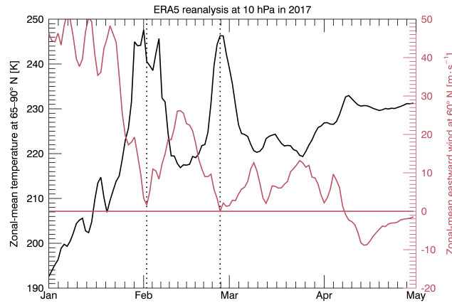
Figure 2. SSW criteria for spring 2017. The zonal mean eastward wind at 60^\circ N is represented in red and the mean temperature from 65\text{--}90^\circ N at 10 hPa is shown in black. Two minor SSWs in February are marked by dotted lines.
