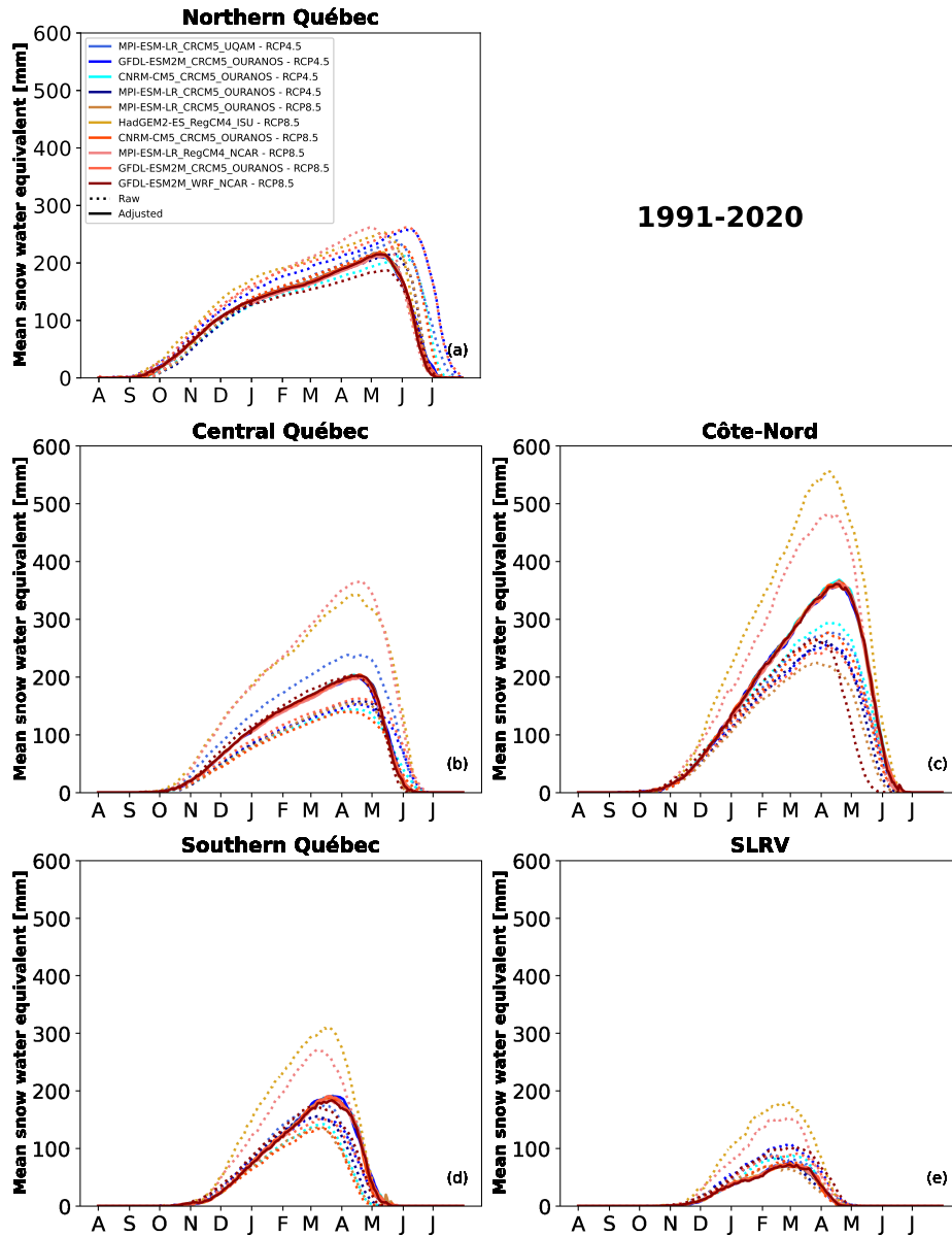
Figure 15. Mean annual cycle of SWE for the five analysis regions for 1991–2020. Raw simulations are represented with dotted lines, and adjusted ones with solid lines. Each colour corresponds to a simulation.
