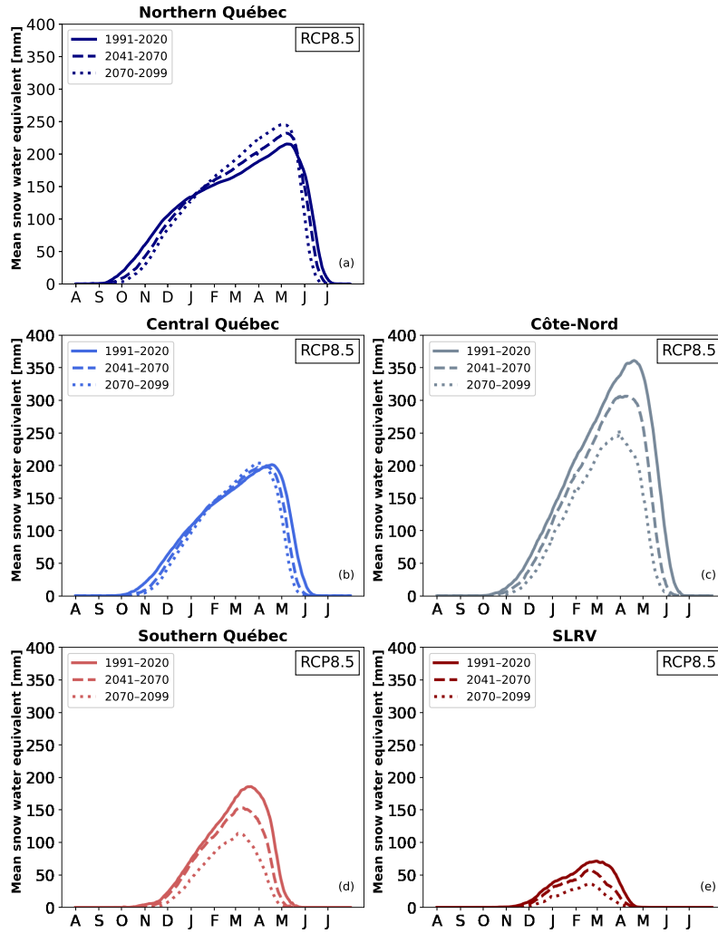
Figure 8. Annual cycle of SWE for the RCP8.5 ensemble in the five analysis regions.
