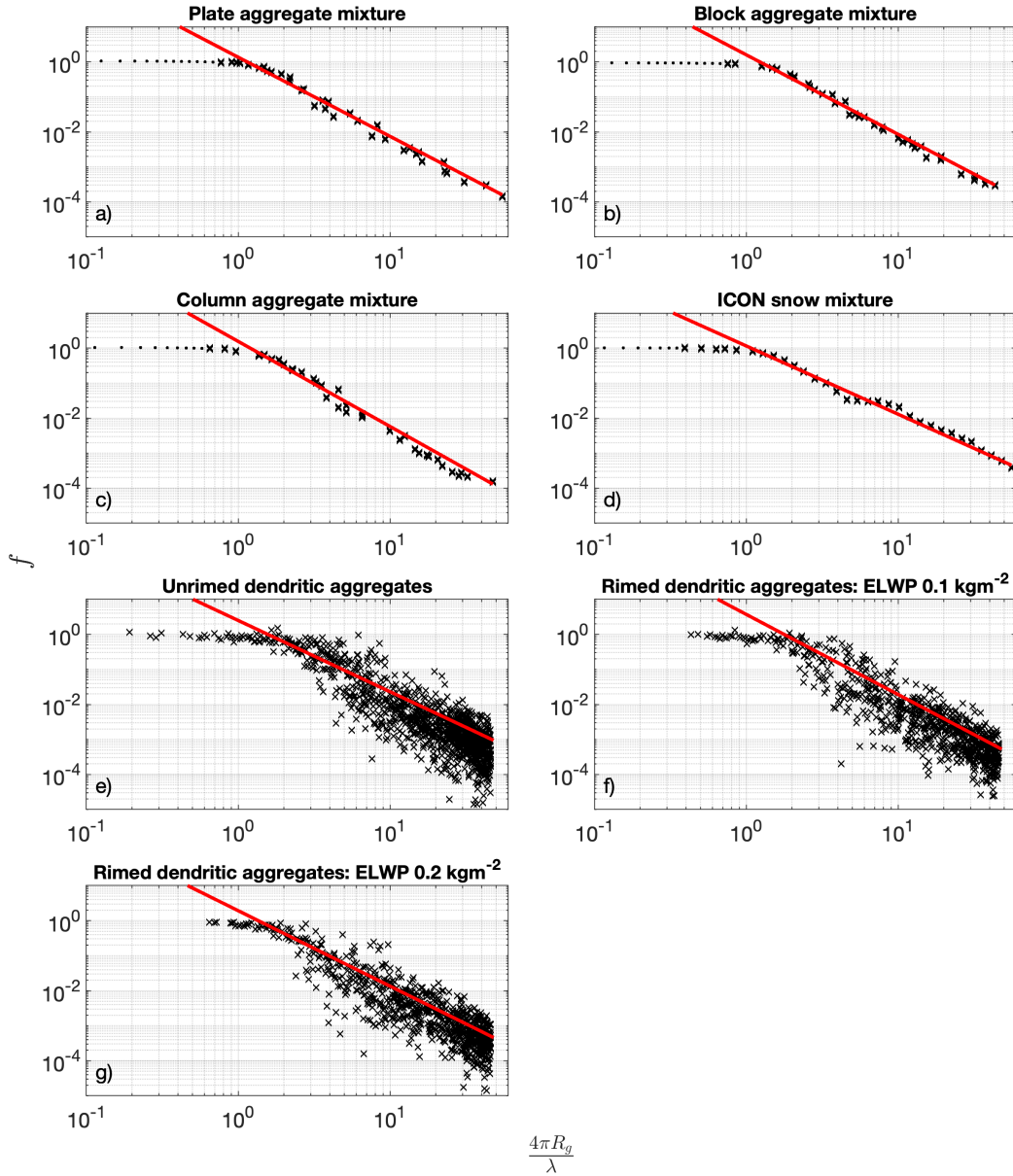
Figure 4. Comparison of f as a function of \frac{4\pi R_g}{\lambda} calculated from data and theory for the different particle habits in this study. The black markers show f calculated using Eq. 15. Panels a-d use data for the ARTS mixtures, where the dots and crosses represent that the particles are monomers and aggregates, respectively. Panels e-g use data for the aggregates from the rimed database. The red lines show the theoretical power law expression for f shown in Eq. 10, illustrating that power law scaling is evident in the data at \frac{4\pi R_g}{\lambda} \gtrsim 1 . Note for the ARTS particles R_g is computed directly for each particle; for the Mroz and Leinonen (2023) database we assumed R_g \approx 0.287D , following Table 1.
