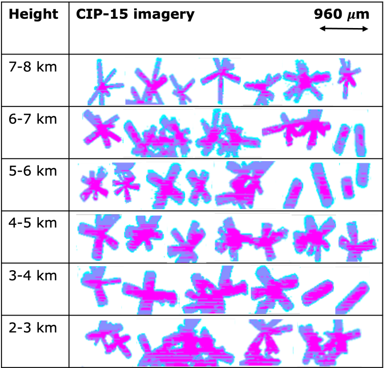
Figure 12. Examples of CIP-15 imagery at different heights on 28 February 2024. The pixel resolution is 15 \mu\text{m} .
