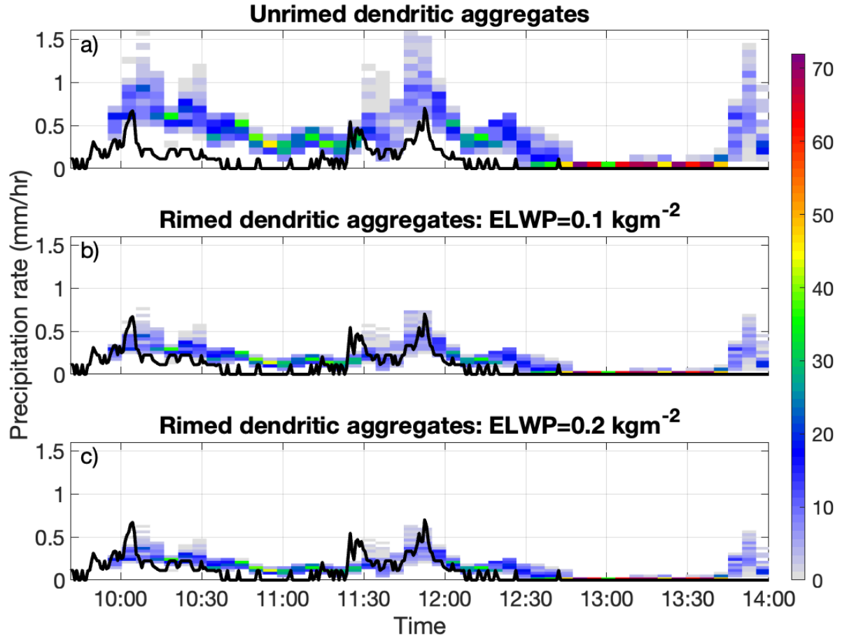
Figure 10. Sensitivity of S retrievals to the choice of particle habit. As in Fig. 9d, the histograms show S retrieved from the bottom \sim 500 m of cloud, while the black lines show the one-minute moving average precipitation rate measured from a drop counting rain gauge at Chilbolton. Panels a-c show results using the three particle habits from the database of Mroz and Leinonen (2023). Panel (a) uses unrimed dendritic aggregates, panel (b) uses rimmed dendritic aggregates with \text{ELWP}=0.1 \text{ kgm}^{-2} (i.e. the original result in Fig. 9d), and panel (c) uses rimmed dendritic aggregates with \text{ELWP}=0.2 \text{ kgm}^{-2} .
