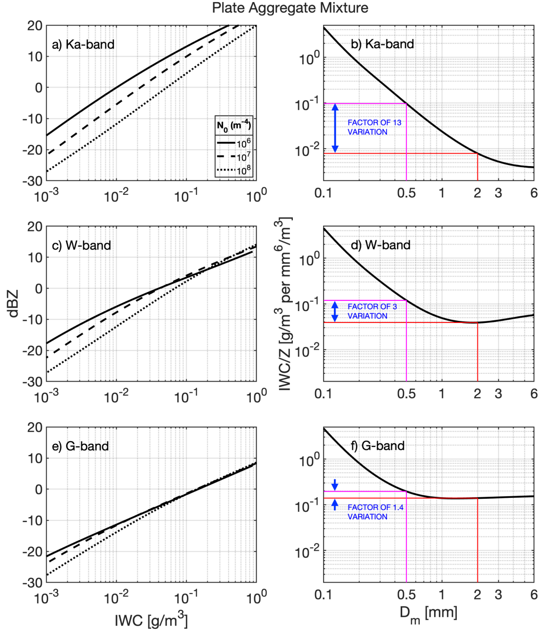
Figure 1. Simulations using the Large Plate Aggregate mixture from the ARTS database, assuming exponential PSDs. The different rows from top to bottom show simulations in the Ka-, W-, and G-band. The left column shows dBZ for a range of IWC, where the different linestyles represent different values of N_0 in the PSDs. The right column shows the ratio IWC/ Z for a range of D_m .
