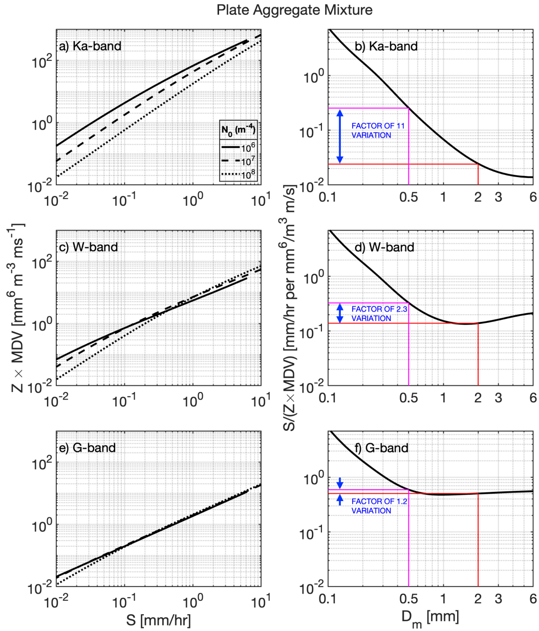
Figure 2. As in Fig. 1, but here the left column shows Z \times \text{MDV} for a range of S , and the right column shows the ratio S/(Z \times \text{MDV}) for a range of D_m .
