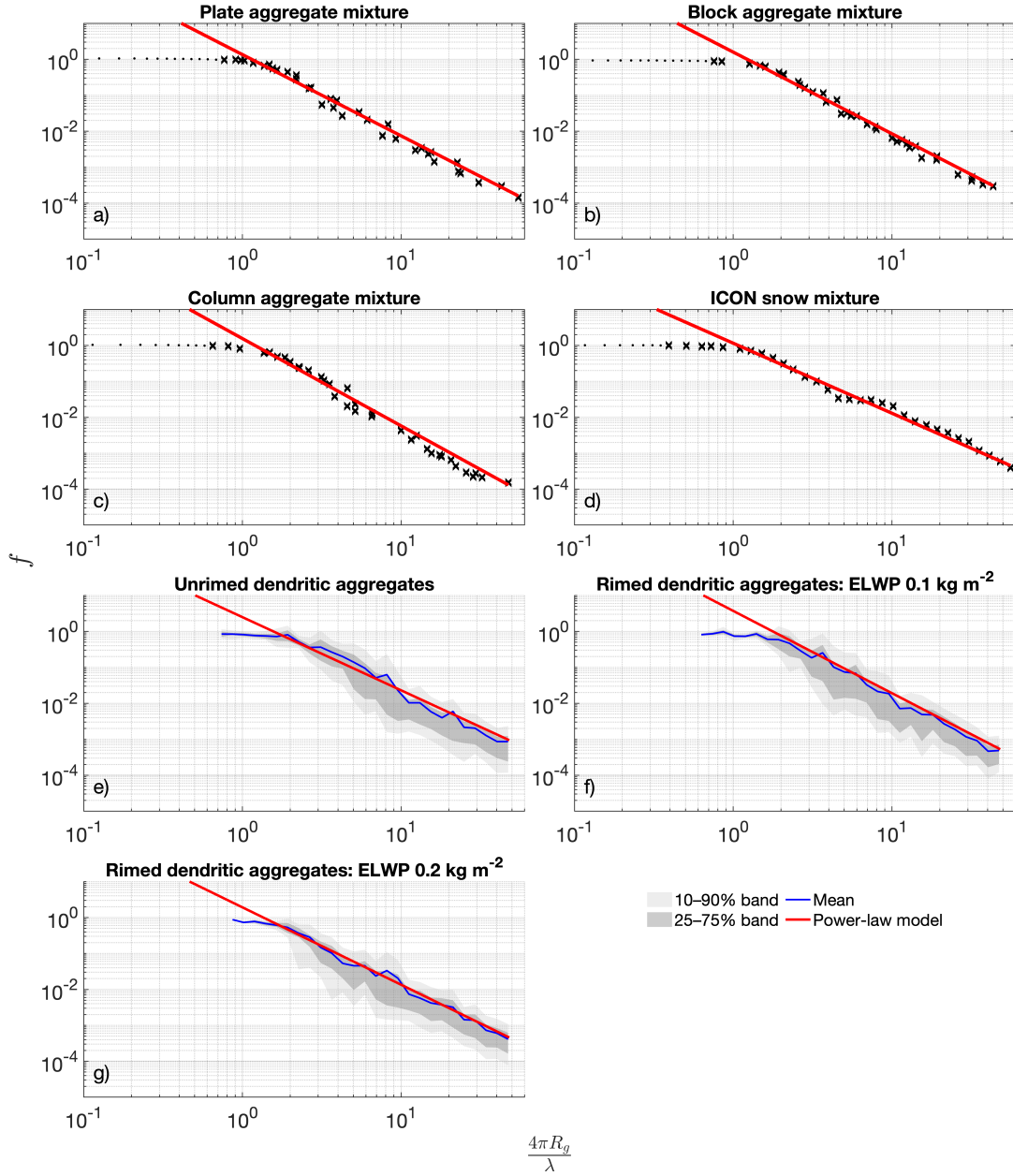
Figure 4. Comparison of f as a function of \frac{4\pi R_g}{\lambda} calculated from data and theory for the different particle habits used in this study. The black markers show f calculated using Eq. 15. Panels a-d use data for the ARTS mixtures, where the black dots and crosses represent that the particles are monomers and aggregates, respectively, with f computed using Eq. 15. Panels e-g use data for the rimed aggregates from the rimed database. For each logarithmic bin in x = \frac{4\pi R_g}{\lambda} , a kernel density estimate of \log_{10} f is used to obtain smooth quantiles. The red-light grey band shows the 10–90% range, the darker band shows the interquartile range, and the blue line shows the mean. Red lines in all panels show the theoretical power-law expression for f shown in (Eq. 10), illustrating that power-law scaling is evident in which captures the data at scaling for \frac{4\pi R_g}{\lambda} \gtrsim 1 . Note for the ARTS particles, R_g is computed directly for each particle; for the Mroz and Leinonen (2023) database we assumed R_g \approx 0.287D , following (Table 1).
