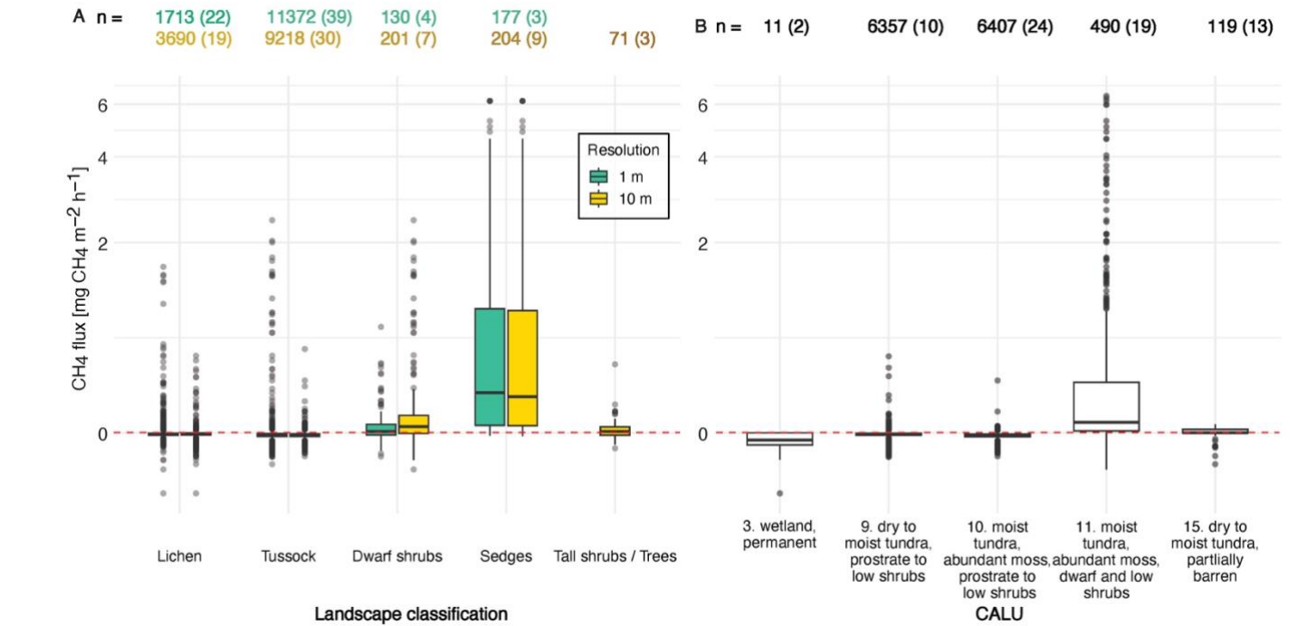
390 Figure 4. Comparison of observed CH 4 fluxes across site-specific landscape classification at two spatial resolutions and CALU (Circumarctic Land cover Units) classes. The numbers above the boxplots indicate the total number of unique measurements followed by the number of Sites of measurements in parentheses Panel A: CH 4 fluxes across five site-specific landscape classes with existing CH 4 flux measurements. Measurements were aggregated separately for 1 m and 10 m spatial resolution. Panel B: CH 4 fluxes grouped by CALU classes. CH 4 fluxes differed significantly between most CALU classes ( p < 0.001 , pairwise Wilcoxon test), except classes 10 and 3 (wetlands), where no significant difference was observed ( p = 0.054 ). Boxplots show the distribution of fluxes for each group. horizontal lines represent medians, boxes indicate the interquartile range, and whiskers extend to 1.5× the IQR. The red dashed lines indicate zero fluxes.
