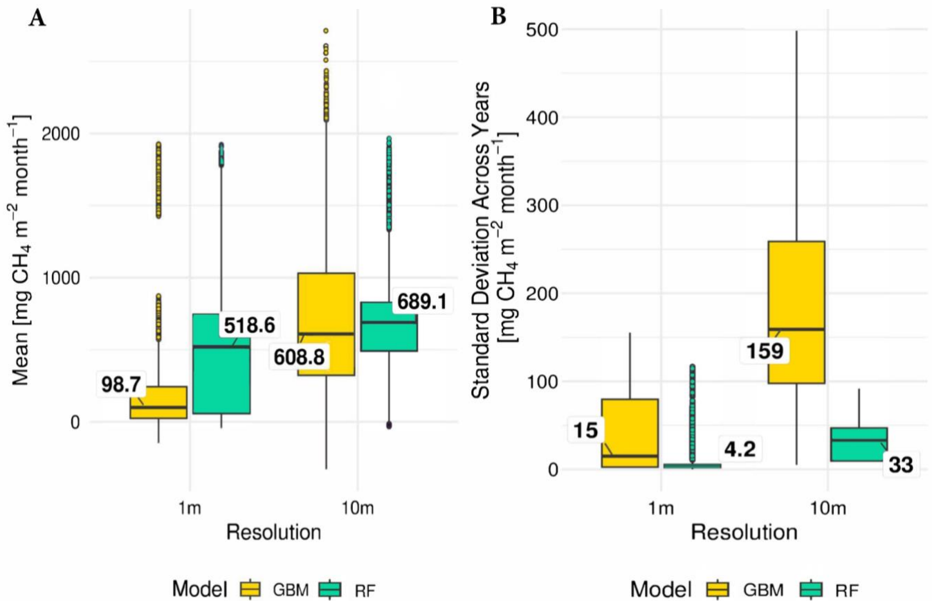
Figure 7. CH 4 fluxes and their interannual variability across the study area. (A) Pixel-wise monthly mean CH 4 flux predicted by RF and GBM models for July 2019-2024. Each point in the boxplots represents the mean July CH 4 flux of a single pixel, illustrating the spatial distribution of fluxes across the study area. (B) Pixel-wise interannual standard deviation of predicted CH 4 fluxes for July months from 2019 to 2024, calculated separately for each model and resolution. The box spans the interquartile range (IQR, 25th–75th percentile), the horizontal line indicates the median, whiskers extend to 1.5×IQR, and points beyond the whiskers represent potential outliers.
