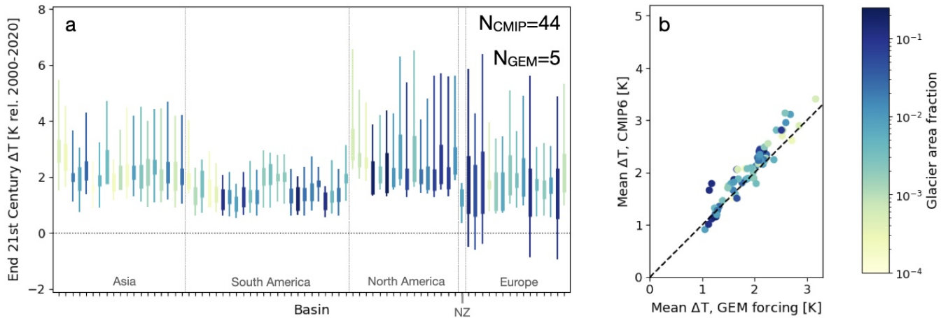
Figure C2. Comparable to main text Figure 5, but limited to models with assessed climate sensitivity within the “likely” range (Table C2). Panel a: Spread in end-of-century (2080-2100) basin-averaged temperature anomaly for (bars) the 5 members of the glacier model forcing ensemble and (whiskers) the 44 members of the CMIP6 archive with data sufficient for SPEI. Panel b: Ensemble means of the same variable, with the glacier model forcing ensemble mean on the x-axis and the CMIP6 ensemble mean on the y-axis; dashed black line shows 1:1 correspondence. Results are colored by basin glacier area fraction and shown in the same basin order as other figures.
