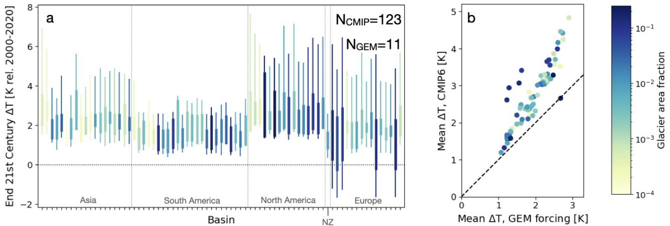
Figure 5. Panel a: Spread in end-of-century (2080-2100) basin-averaged temperature anomaly for (bars) the 11 members of the glacier model forcing ensemble and (whiskers) the 123 members of the CMIP6 archive with data sufficient for SPEI. Panel b: Ensemble means of the same variable, with the glacier model forcing ensemble mean on the x-axis and the CMIP6 ensemble mean on the y-axis; dashed black line shows 1:1 correspondence. Results are colored by basin glacier area fraction and shown in the same basin order as other figures; time series for each basin are shown in Figure D2.
