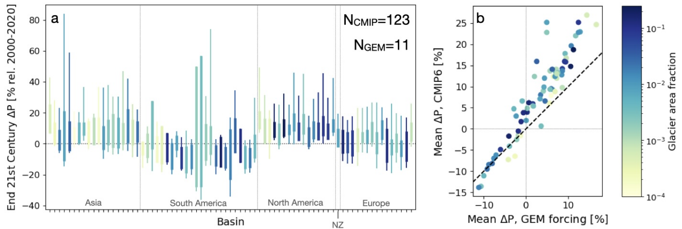
Figure 4. Panel a: Spread in end-of-century (2080-2100) percent change in total basin precipitation for (bars) the 11 members of the glacier model forcing ensemble and (whiskers) the 123 members of the CMIP6 archive with data sufficient for SPEI. Panel b: Ensemble means of the same variable, with the glacier model forcing ensemble mean on the x-axis and the CMIP6 ensemble mean on the y-axis; dashed black line shows 1:1 correspondence. Results are colored by basin glacier area fraction and shown in the same basin order as other figures; time series for each basin are shown in Figure D1.
