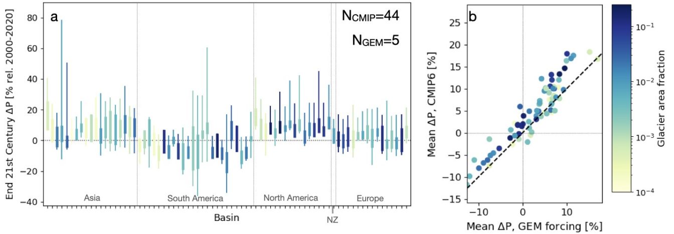
Figure C1. Comparable to main text Figure 4, but limited to models with assessed climate sensitivity within the “likely” range (Table C2). Panel a: Spread in end-of-century (2080-2100) basin-averaged precipitation anomaly for (bars) the 5 members of the glacier model forcing ensemble and (whiskers) the 44 members of the CMIP6 archive with data sufficient for SPEI. Panel b: Ensemble means of the same variable, with the glacier model forcing ensemble mean on the x-axis and the CMIP6 ensemble mean on the y-axis; dashed black line shows 1:1 correspondence. Results are colored by basin glacier area fraction and shown in the same basin order as other figures.
