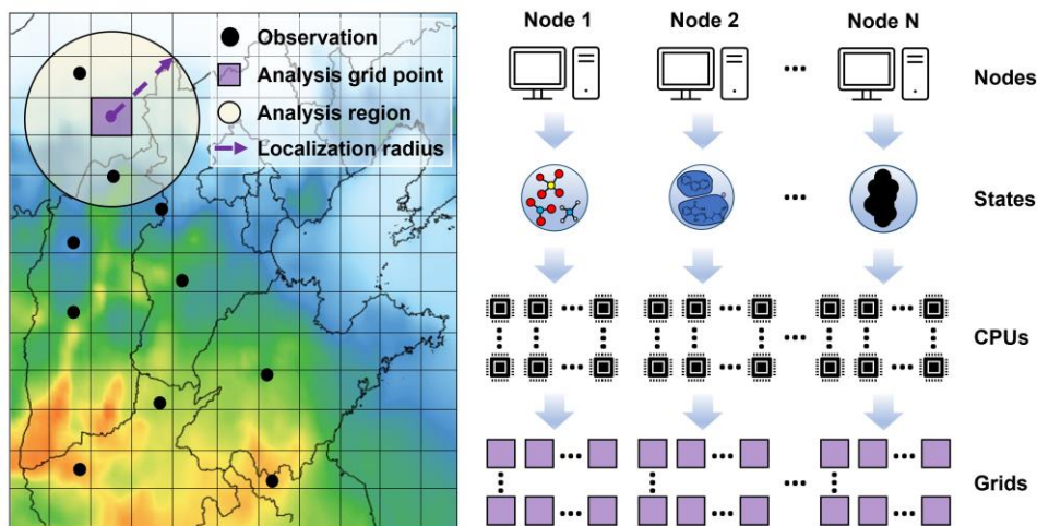
390 Figure 2. The scheme for domain localization and parallelization.
