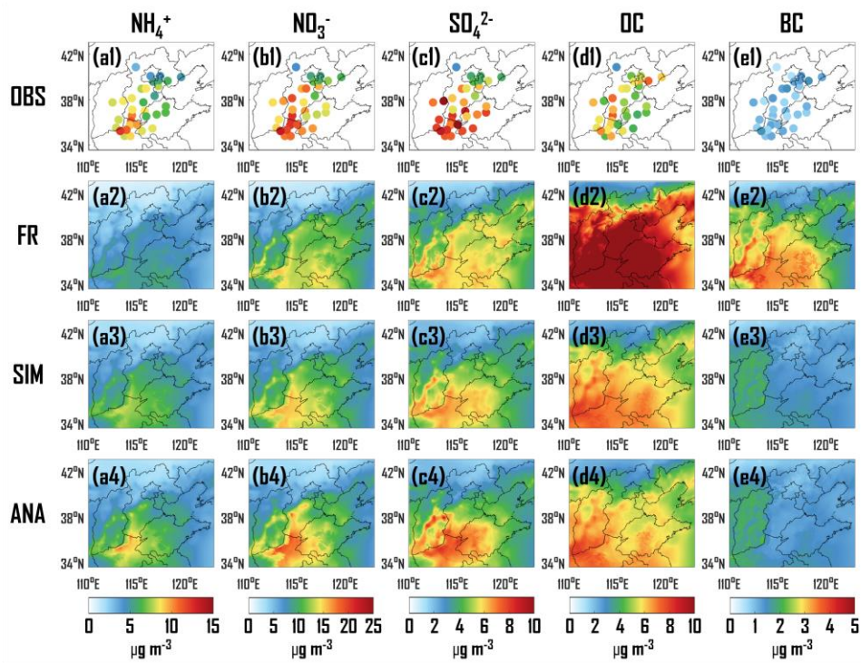
740 Figure 6. Spatial distribution of observation (OBS), free-run field (FRFR), ML-simulated background field (SIM) and analysis field (ANA) for NH 4 + (a1-a4), NO 3 - (b1-b4), SO 4 2- (c1-c4), OC (d1-d4) and BC (e1-e4).
