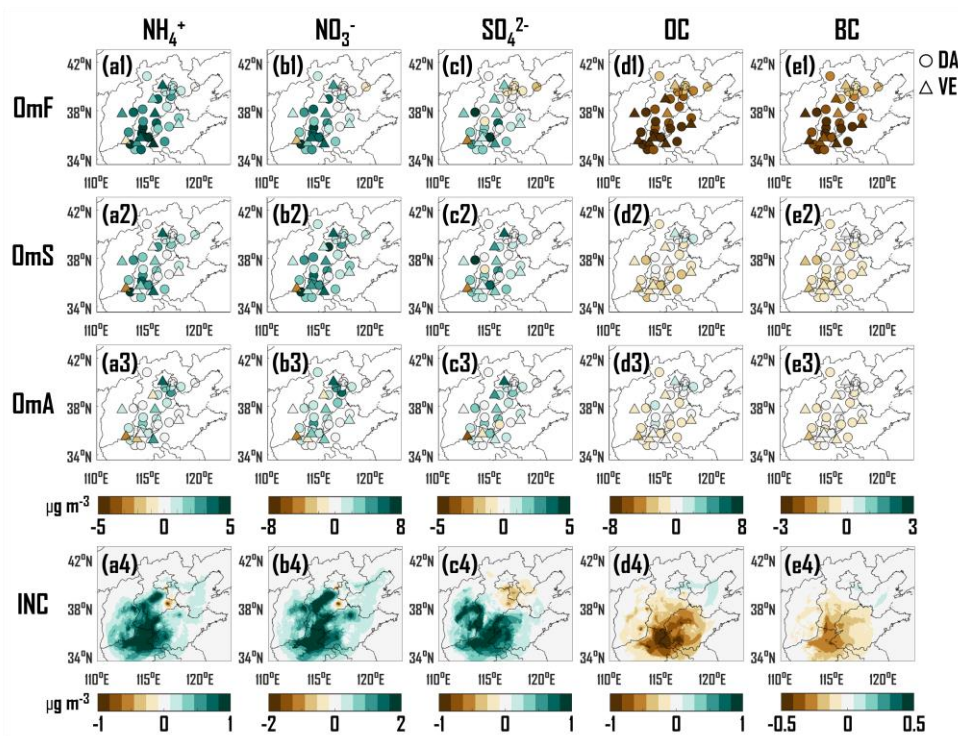
750 Figure 7. Spatial distribution of observation minus free-run field (OmF) , observation minus ML-simulated background field (OmS) , observation minus analysis field (OmA) and analysis field minus background field (INC) for \text{NH}_4^+ (a1-a4), \text{NO}_3^- (b1-b4), \text{SO}_4^{2-} (c1-c4), OC (d1-d4) and BC (e1-e4). The circle indicates the DA sites with data assimilation, and the upward-pointing triangle indicates the VE sites without data assimilation.
