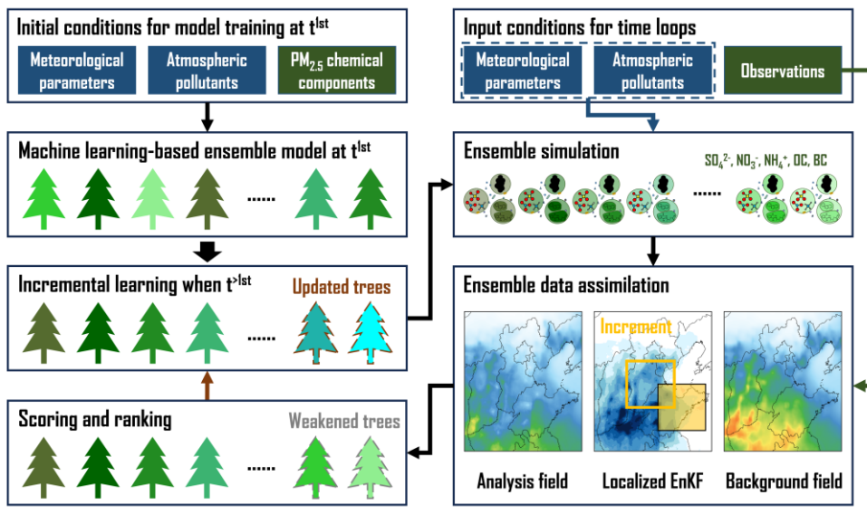
Figure 1. The framework of OIRF-LEnKF v1.0.
