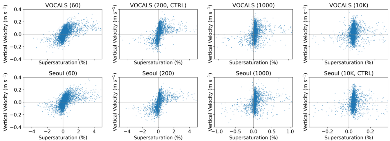
Figure 8. Scatterplot of the vertical velocity as a function of the supersaturation for the last 15 min of the simulations. Only 350 0.1% of randomly selected grid points away from chamber boundaries are included in the plot.
