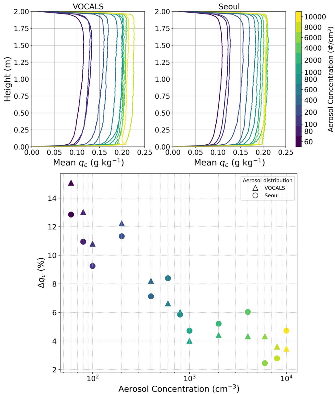
Figure 3. Top panels: Vertical profiles of time-averaged cloud water mixing ratio ( q_c ) from 0 to 2 m height for VOCALS (left) and Seoul (right) aerosol cases at varying aerosol concentrations (60–10K \text{cm}^{-3} ). Each colored line corresponds to a different aerosol concentration (see legends). Profiles are averaged over the quasi-equilibrium period (15–30 min). Bottom panel: \Delta q_c as a function of aerosol concentration, where each point represents the averaged value for the quasi-equilibrium period (15–30 min) of each aerosol distribution. Large \Delta q_c indicates a strong increase of q_c with height, whereas small or negligible \Delta q_c would indicate a nearly uniform vertical q_c profile. Triangles denote VOCALS cases; circles denote Seoul cases.
