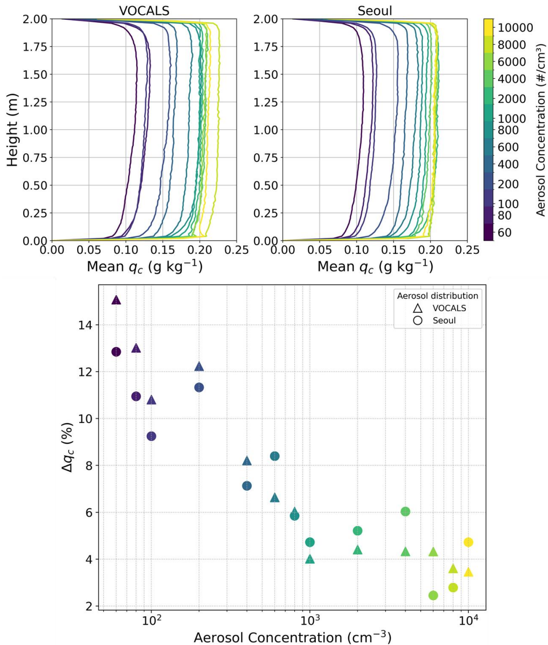
240 Figure 3. Top panels: Vertical profiles of time-averaged cloud water mixing ratio ( q_c ) from 0 to 2 m height for VOCALS (left) and 245 Seoul (right) aerosol cases at varying aerosol concentrations (60–10K \text{cm}^{-3} ). Each colored line corresponds to a different aerosol concentration (see legends). Profiles are averaged over the quasi-equilibrium period (15–30 min). Bottom panel: \Delta q_c as a function of aerosol concentration, where each point represents the averaged value for the quasi-equilibrium period (15–30 min) of each aerosol distribution. Large \Delta q_c indicates a strong increase of q_c with height, whereas small or negligible \Delta q_c would indicate a nearly uniform vertical q_c profile. Triangles denote VOCALS cases; circles denote Seoul cases.
