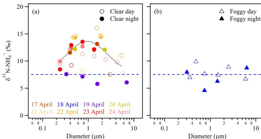
Figure 4. \delta^{15}\text{N} of size-segregated p\text{NH}_4^+ during (a) clear and (b) foggy conditions. The dashed blue line indicates the mean \delta^{15}\text{N-NH}_4^+ for foggy periods. The dotted curve represents LogNormal distribution fits for clear conditions, excluding 19N and 21D, where no distinct bell-shaped size dependence was identified.
