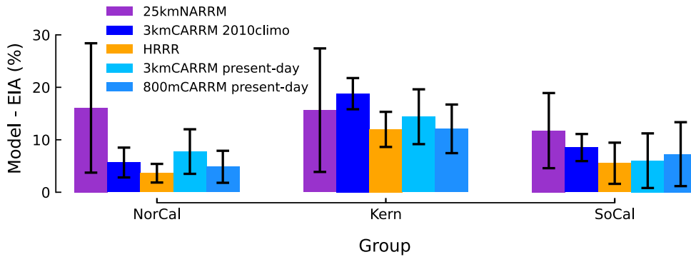
Figure 9. Multi-year mean monthly absolute errors Absolute bias (relative to EIA) of multi-year, plant-aggregated wind CFs by plant (%) from PySAM simulations compared to monthly EIA data: E3SM-25kmNARRM E3SM-25km NARRM (darkorchid), SCREAM-3kmCARRM SCREAM-3km CARRM 2010climo (blue), HRRR (orange), SCREAM-3kmCARRM SCREAM-3km CARRM present-day (deepskyblue), and SCREAM-800m CARRM present-day (dodgerblue). Each dot represents Bar heights indicate the mean absolute difference between bias averaged over the multi-year mean climatological monthly CF cycle , and error bars denote the corresponding EIA value for each plant standard deviation . The black horizontal bar shows the mean absolute error (MAE) for each group, averaged over all months and plants.
