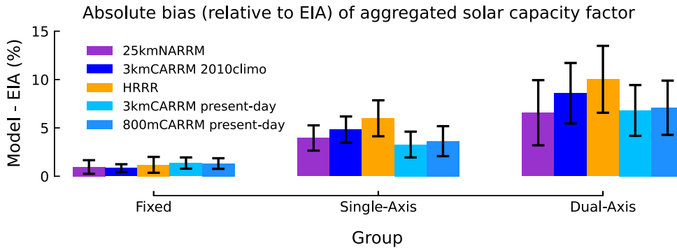
Figure 16. As in Fig. 10-9 but for solar CFs.
