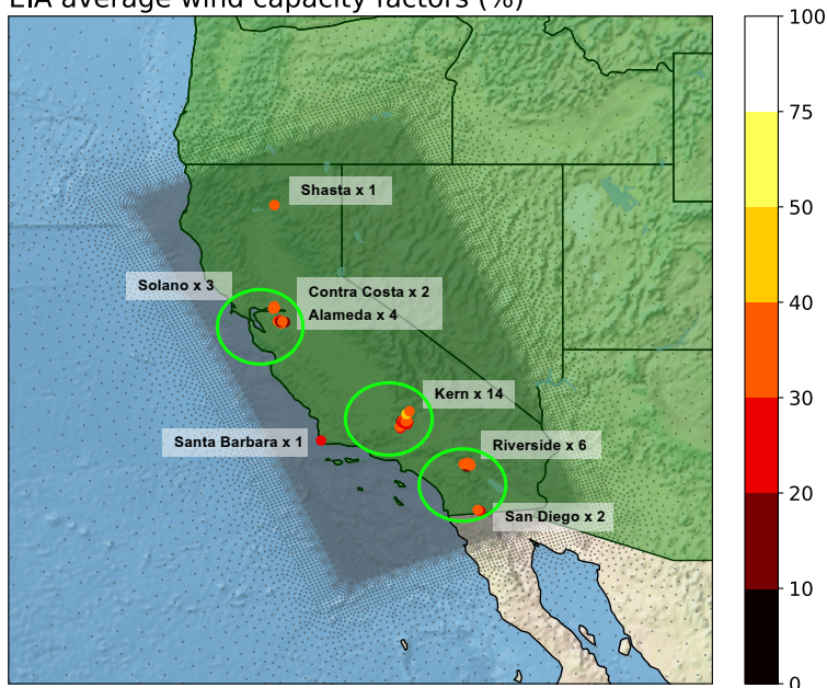
Figure 2. Clusters of wind plants across California, grouped by geographic proximity. Each cluster is marked with a green ellipse and annotated with the county name and number of plants. EIA plants are aggregated to the 3kmCARRM model grid; each filled dot represents the mean wind CF (%) from valid monthly EIA records between 2013 and 2023 2024 .
