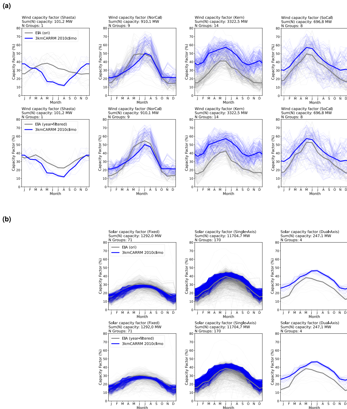
Figure A3. Seasonal variation in the (a) wind and (b) solar CFs (%) estimated using PySAM from SCREAM-3kmCARRM 2010climo, before (upper) and after (bottom) applying the “independent-plant ratio > 15%” threshold (i.e., excluding years dominated by imputed plant data). The years before filtering are 2013–2023, 2024, while the remaining valid years after filtering are {2013, 2014, 2015, 2016, 2023, 2024} for wind and {2014, 2016, 2020, 2021, 2022, 2023, 2024} for solar, respectively. Each subplot column corresponds to a cluster in Fig. 2 for wind or solar CFs, with Shasta also included here. Simulations are shown in blue, and EIA records in gray. Light lines represent individual years; bold lines represent the multi-year climatology.
