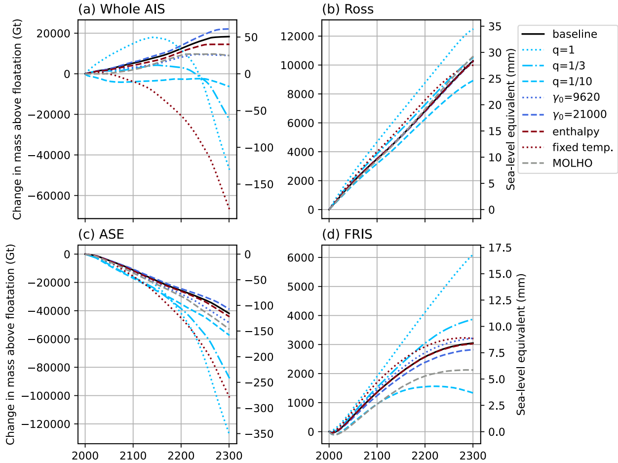
Figure C1. Mass change for the whole ice sheet (a) and regions of interest (b–d) from control simulations for the parameter and model fidelity sensitivity studies.
