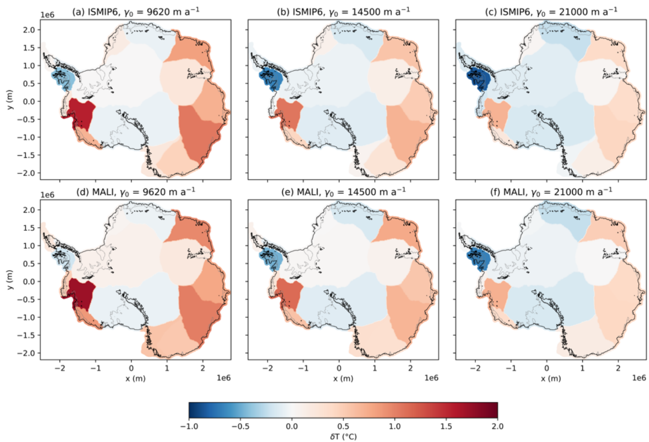
Figure B2. Temperature correction to ocean thermal forcing provided by ISMIP6 (a–c) and used in MALI simulations (d–f) for the three different values of the sub-shelf melt parameter, \gamma_0 .
