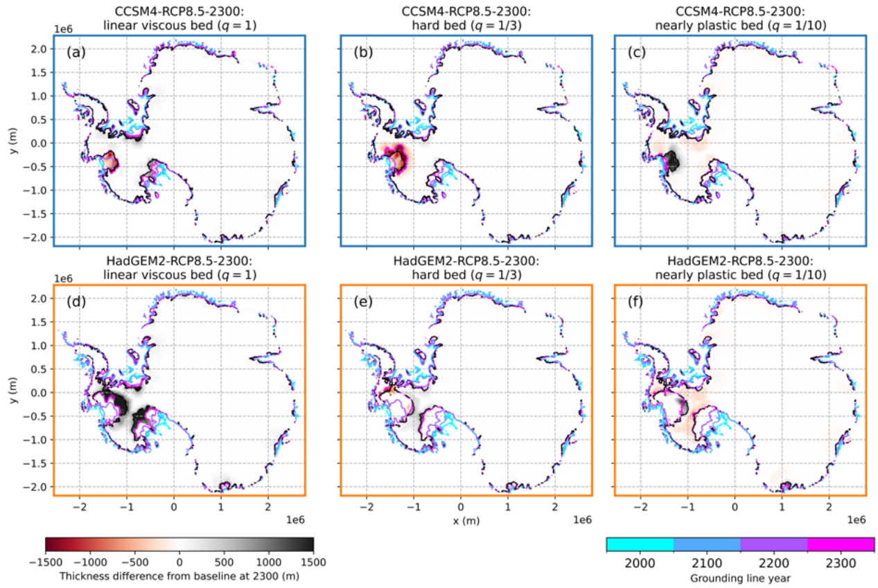
Figure D2. Maps of thickness relative to baseline runs ( q = 1/5 ) at 2300 for experiments with q values of 1 (a, d), 1/3 (b, e), and 1/10 (c, f). Grounding lines from the sensitivity experiments are shown by colored curves at 2000, 2100, 2200, and 2300, while the grounding lines at 2300 from baseline simulations are shown in black.
