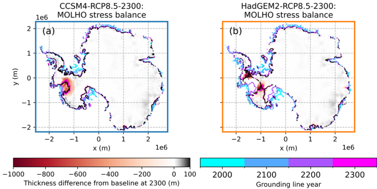
Figure D4. Maps of thickness relative to the baseline runs at 2300, for experiments using the depth-integrated solver. Grounding lines from the sensitivity experiments are shown by colored curves at 2000, 2100, 2200, and 2300, while the grounding lines at 2300 from baseline simulations are shown in black.
