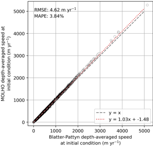
Figure A1. Depth-averaged speed from the MOLHO and Blatter-Pattyn solvers for all grounded ice cells at the initial condition. Red dotted curve denotes linear least-squares fit to the data ( R^2 = 0.9991 ). Dashed grey curve is 1:1 line. RMSE: root mean square error; MAPE: mean absolute percent error.
