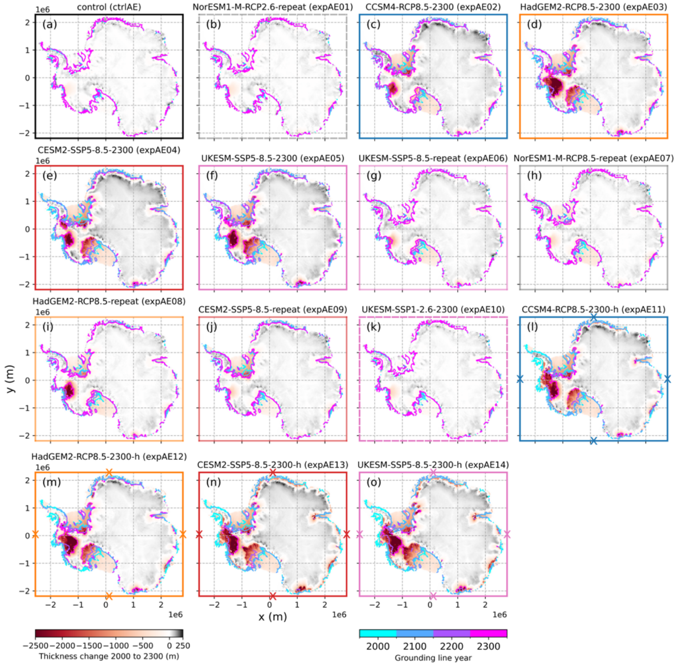
Figure 4. Maps of ice thickness change from 2000–2300 from the baseline ensemble submitted to ISMIP6-Antarctica-2300, with grounding line positions at 2000, 2100, 2200, and 2300. Axis border colors and line styles match the corresponding mass change curves in Fig. 3.
