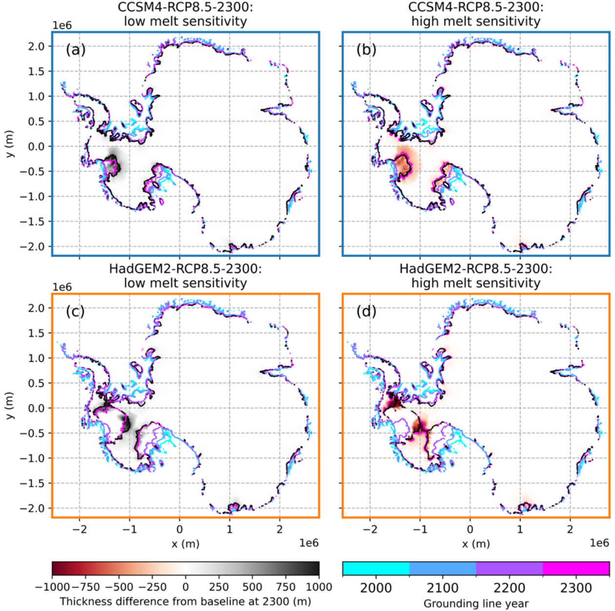
Figure D1. Maps of thickness relative to baseline runs ( \gamma_0 = 14500 \text{ m a}^{-1} ) at 2300 for low melt sensitivity ( \gamma_0 = 9620 \text{ m a}^{-1} ) (a, c) and high melt sensitivity ( \gamma_0 = 21000 \text{ m a}^{-1} ) (b, d) experiments. Grounding lines from the sensitivity experiments are shown by colored curves at 2000, 2100, 2200, and 2300, while the grounding lines at 2300 from baseline simulations are shown in black.
