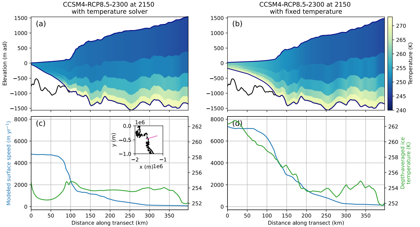
Figure 13. Modeled ice geometry and temperature (a, b) and surface flow speeds and depth-averaged temperature (c, d) taken from a transect down the center of Thwaites Glacier at 2150 from the CCSM4-RCP8.5-2300 simulations with an evolving temperature field (a, c) and with a fixed temperature field (b, d). Inset in (c) shows the location of the transect in pink, with the c. 2000 ASE grounding line in black.
