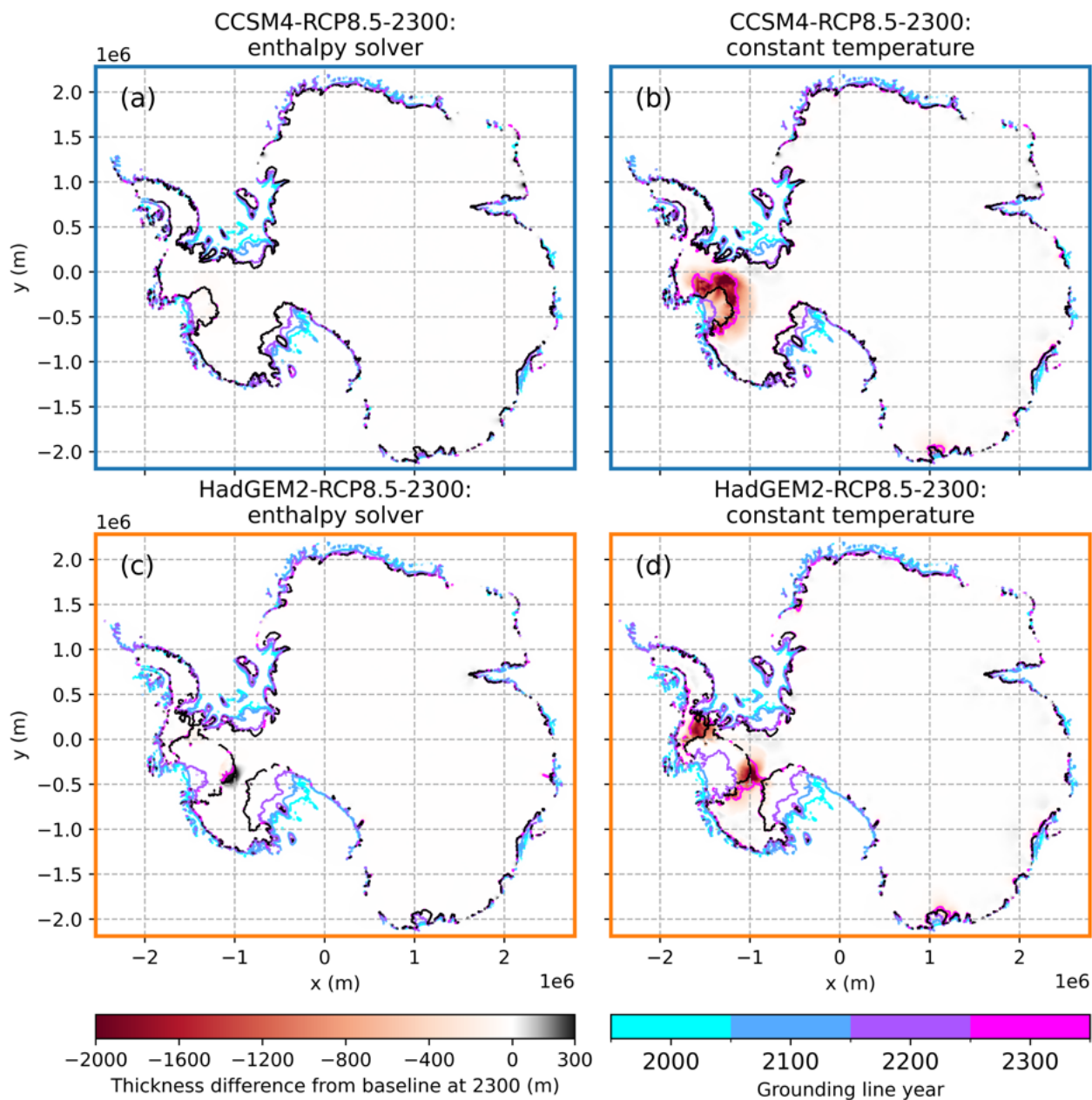
Figure D3. Maps of thickness relative to the baseline runs using the temperature formulation at 2300, for experiments using the enthalpy formulation (a, c) and a fixed temperature field (b, d). Grounding lines from the sensitivity experiments are shown by colored curves at 2000, 2100, 2200, and 2300, while the grounding lines at 2300 from baseline simulations are shown in black.
