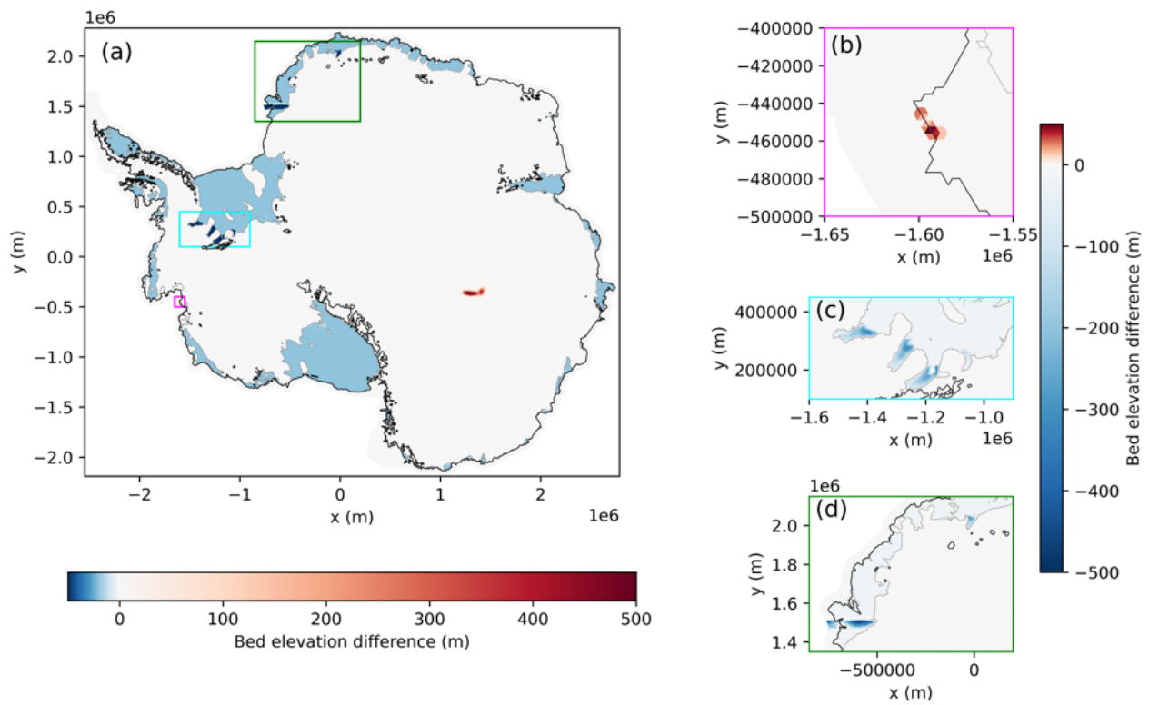
Figure B1. Difference in bed elevation used in MALI simulations relative to BedMachineAntarctica v2 (Morlighem et al., 2020). Negative values indicate a deeper bed in MALI.
