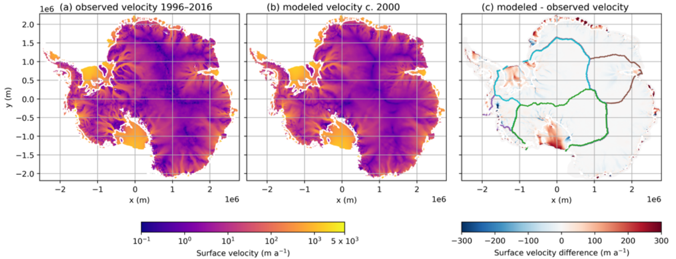
(a) Observed 1996–2016 composite surface velocities (Rignot et al., 2017). (b) MALI initial condition with a nominal date of 2000, following optimization to match observed 1996–2016 mean velocities in (a) and a ten-year relaxation simulation. (c) Difference between modeled and observed velocities. Colored contours represent the regions that we analyze throughout this study: purple — ASE; cyan — FRIS; green — Ross; brown — Amery. The grounding line is represented by the grey curves in all panels.
