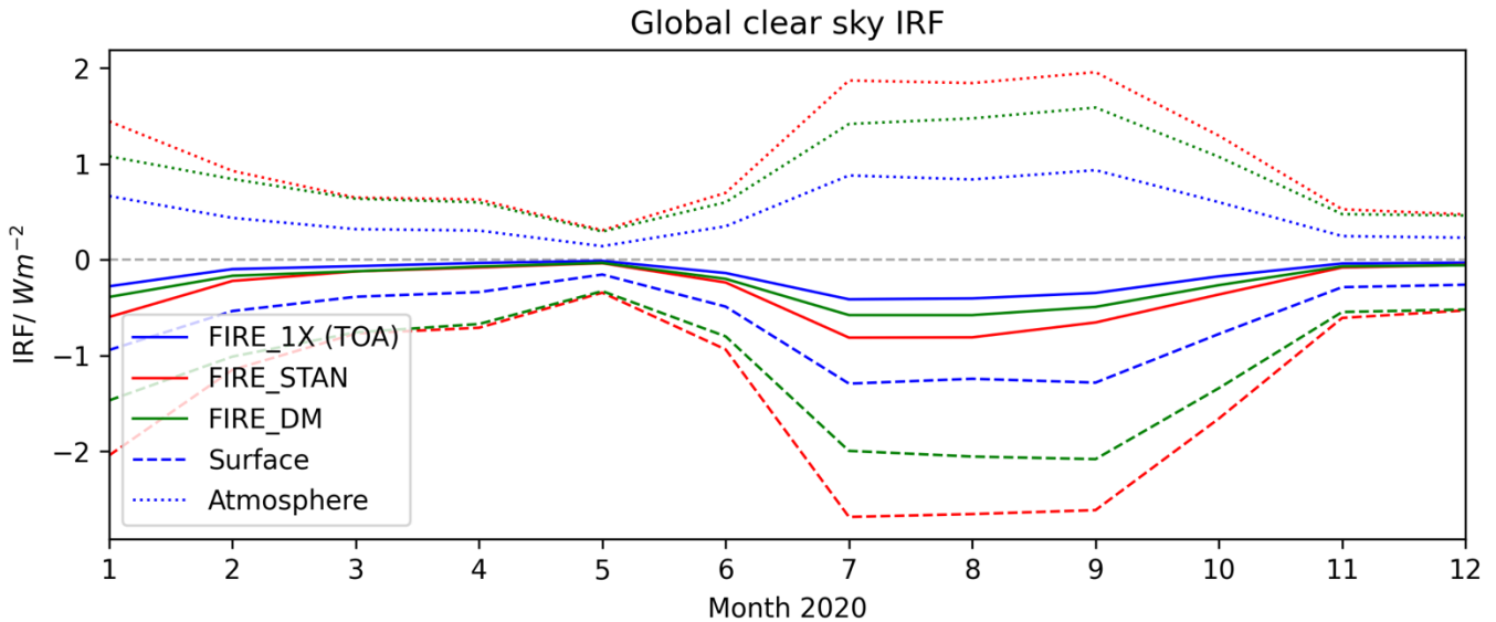
Figure 13: Clear sky (cloud free) shortwave top of atmosphere instantaneous radiative forcing (solid line) of wildfire aerosol globally (i.e. changes in radiative fluxes relative to the NOFIRE simulation), for three simulations: FIRE_1X (blue), FIRE_STAN (red), and FIRE_DM (green), for the year 2020. Dashed line is surface forcing (reduction of the net shortwave clear-sky radiation at the surface), and dotted line is atmospheric forcing (absorption of shortwave radiation in the atmosphere under clear-sky conditions).
