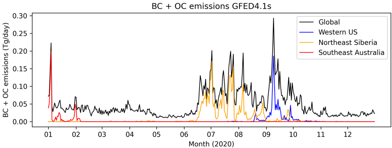
Figure 1: Combined organic carbon (OC) and black carbon (BC) emissions over the year 2020 from GFED4.1s. Black line shows the global total. Blue line shows the western United States emissions ( -125 – 115^{\circ} E, 30 – 50^{\circ} N). Orange line shows the northeast Siberian emissions ( 90 – 175^{\circ} E, 55 – 80^{\circ} N). Red line shows southeast Australian emissions ( 140 – 180^{\circ} E, -30 – 45^{\circ} N).
