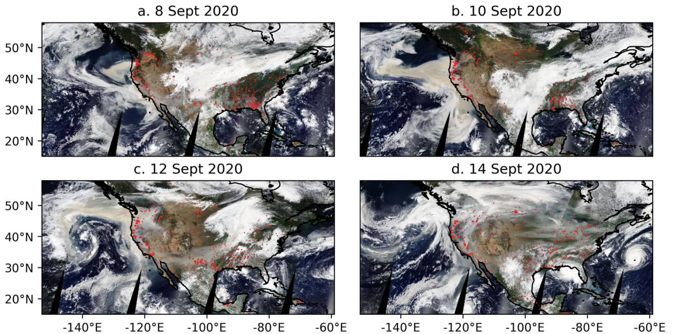
105 Figure 2: MODIS Corrected Reflectance imagery over North America for 8th, 10th, 12th, and 14th September 2020. Red shows active fire detections and thermal anomalies from Suomi NPP / VIIRS (Visible Infrared Imaging Radiometer Suite) Fire and Thermal Anomalies (Day and Night, 375 m). Imagery from the Worldview Snapshots application ( https://wvs.earthdata.nasa.gov ), part of the Earth Science Data and Information System (ESDIS)
