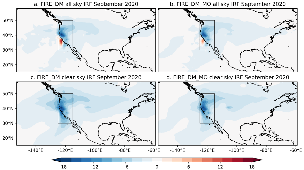
Figure 14: Mean top-of-atmosphere shortwave instantaneous radiative forcing for September 2020, calculated as the difference between FIRE_DM simulations and NOFIRE IRE. a. all-sky FIRE_DM (daily mean emissions) b. all-sky FIRE_DM_MO (monthly mean emissions) c. clear-sky FIRE_DM d. clear-sky FIRE_DM_MO. All-sky includes the effects of clouds (both cloudy and clear regions), clear-sky represents the forcing under cloud free conditions only. The western US region is outlined by the black box and consistent with previous figures and analyses spans -125 – -115^\circ \text{ E} and 30 – 50^\circ \text{ N} .
