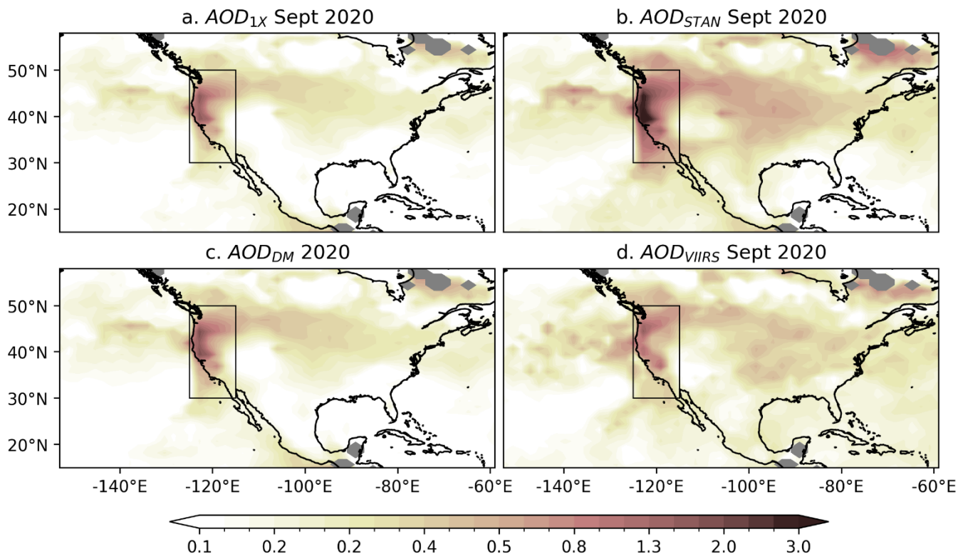
525 Figure 9: Mean Aerosol optical depth for September 2020. a. AOD from simulation FIRE_1X, using unscaled emissions. b. AOD from simulation FIRE_STAN, emissions scaled by 2x. c. AOD from FIRE_DM, emissions are scaled based on dry matter consumption, d. AOD from Suomi VIIRS Deep Blue. The areas of grey represent missing data.
