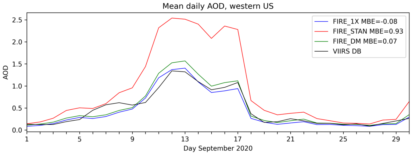
540 Figure 11: Area weighted daily mean AOD for region in western US, bounded by -125–115° E, 30–50° N, as marked in Fig. 9 by black rectangle. The black line is observational data from Suomi VIIRS Deep Blue, blue is the FIRE_1X simulation, red is the FIRE_STAN simulation, and green is FIRE_DM simulation. The Mean Bias Error (MBE) is calculated for each simulation.
