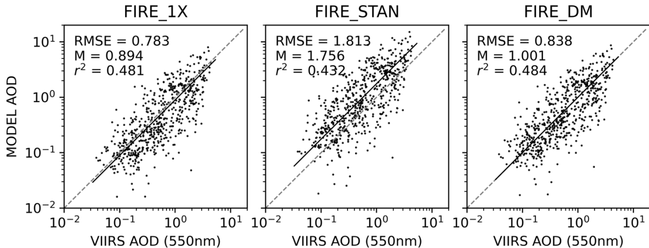
575 Figure 12: Scatter plots of the carbon monoxide screened AOD (CO>100 ppbv) in the western USA, for September 2020. VIIRS Deep Blue AOD against a. FIRE_1X b. FIRE_STAN c. FIRE_DM. In each plot the line of best fit forced through the origin is drawn, the gradient of which (M) is displayed in the top left. The root mean square error (RMSE) and coefficient of determination ( r^2 ) are shown.
