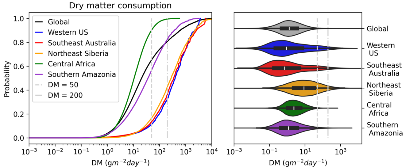
315 Figure 4: Cumulative distribution function of daily mean dry matter (fuel) consumption from biomass burning in 2020 (left). The black line represents the global probability. Regions of fire occurrence are shown in blue (western US), red (southeast Australia), green (central Africa), orange (northeast Siberia), and purple (southern Amazonia). To the right, violin plots show the probability distributions of each region. The white line shows the median value, and the black box shows the interquartile range. In both plots, grey vertical dashed lines represent the FIRE_DM scaling factor thresholds.
