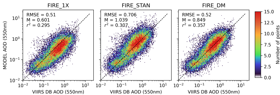
Figure 5: Scatter plots of the carbon monoxide screened AOD ( CO > 100 ppbv) in the selected five regions (boxes in Fig. 10) where biomass burning was a strong source of aerosol in 2020. Colour bar represents overlapping points, where red shows the highest density of points, and dark purple shows just one point. VIIRS Deep Blue AOD against a. FIRE_1X b. FIRE_STAN c. FIRE_DM. In each plot gradient of the line of best fit forced through the origin ( M ) is displayed in the top left. The root mean square error (RMSE) and coefficient of determination ( r^2 ) are also shown here.
