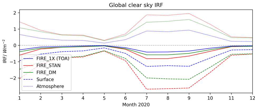
1975 Figure 13: Clear sky (cloud free) shortwave top of atmosphere instantaneous radiative forcing (solid line) of wildfire aerosol globally (i.e. changes in radiative fluxes relative to the NOFIRE simulation), for three simulations: FIRE_1X (blue), FIRE_STAN (red), and FIRE_DM (green), for the year 2020. Dashed line is surface forcing (reduction of the net shortwave clear-sky radiation at the surface), and dotted line is atmospheric forcing (absorption of shortwave radiation in the atmosphere under clear-sky conditions).
