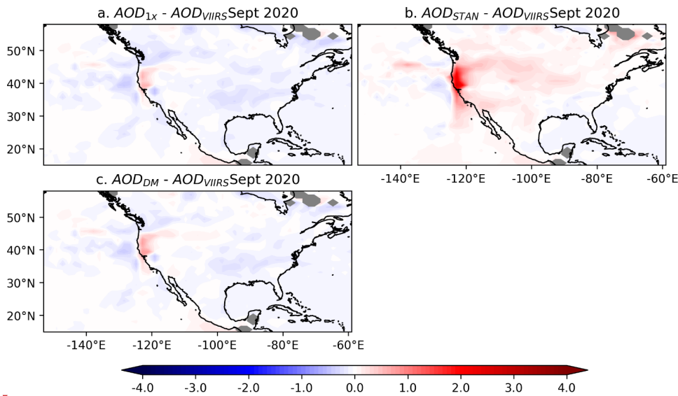
Figure 10: Difference between observations and model, September mean AOD a. FIRE_1X and VIIRS DB, b. FIRE_STAN and VIIRS DB, c. FIRE_DM and VIIRS DB. Blue represents areas where the model simulation is underpredicting the AOD, red represents areas where the AOD is being overestimated by the simulation. The areas of grey represent missing data.
