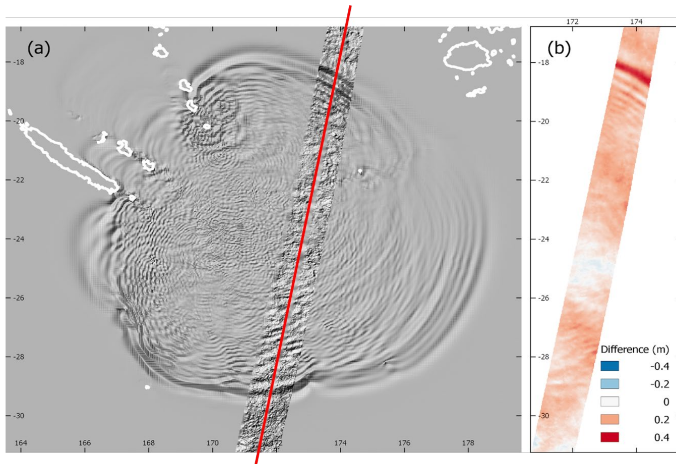
Figure 5: (a) Superposition of the SWOT satellite swath (presented on figure 2) with the simulated tsunami propagation wavefield at t=T_0 (62' after earthquake occurrence time T_e ), using the GCMT-based scenario of coseismic rupture from Roger and Gusman (2024); (b) sea-surface elevation difference between SWOT record and the modelling output. The red line symbolizes the Nadir location in the middle of the swath (KaRIn). Note that SWOT record goes from T_0 = T_e + 62' (SW) to T_1 = T_e + 65' (NE).
