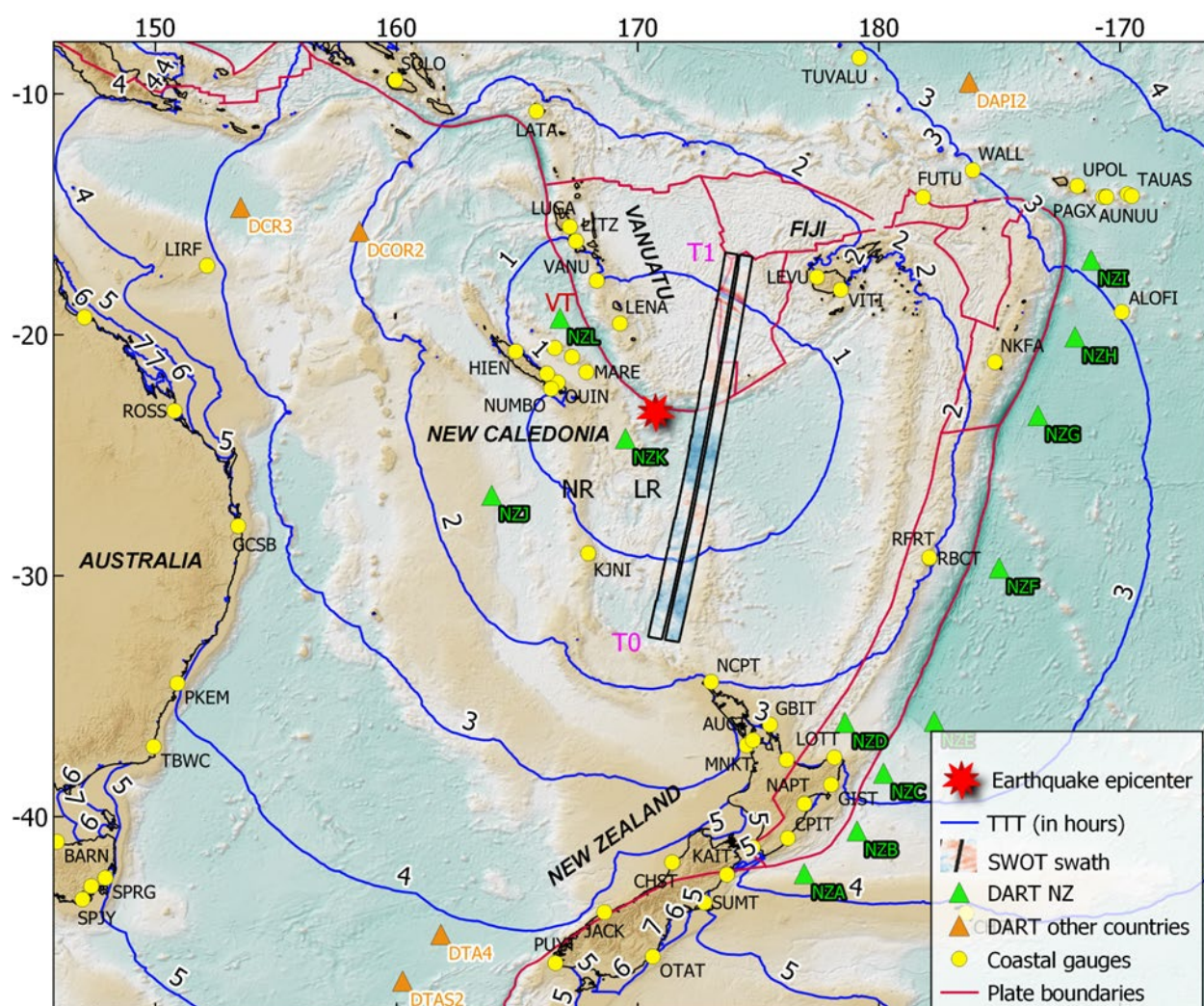
Figure 1: The 19 May 2023 Mw 7.7 earthquake and tsunami. Tsunami travel times from the epicenter were calculated using Mirone software (Luis, 2017). The coloured band symbolizes the swath track of the SWOT satellite dataset presented herein with T0 and T1 symbolizing the start and end time of the swath. VT: Vanuatu Trench; LR: Loyalty Ridge; NR: Norfolk Ridge. Background topography is from GEBCO (GEBCO, 2023).
