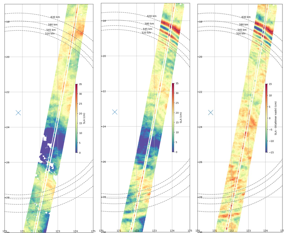
150 Figure 2: The SWOT SLA on pass 147 (left) the 18th of May 2023 (cycle 524) 23h before the Earthquake, (center) the 19th of May (cycle 525) 1h after the earthquake. (right) is the same as (center) but with ocean variability estimated by MIOST removed. The dashed concentric lines symbolize the distance from the epicenter.
