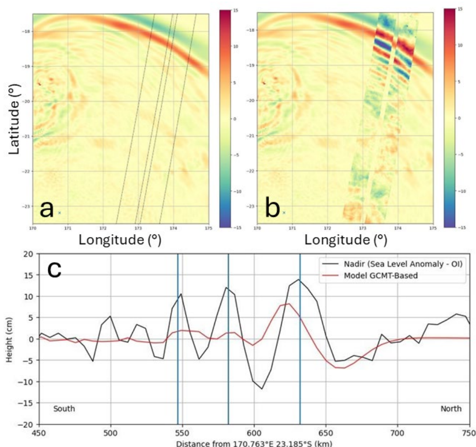
Figure 4: Comparison between nadir SWOT measurements and the model estimation cross-section at T+1h: (a) GCMT-based model only with position of SWOT measurement, (b) SWOT measurement superimposed on the model field, (c) SWOT and model comparison along the nadir.
