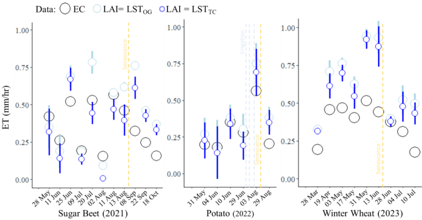
678 Figure C4: Field averages of the TSEB-PT ET estimations comparing the change between using LSTOG and 679 LSTTC in comparisons to the EC ET estimations with (a) sugar beet in 2021 (b) potato in 2022 (c) winter 680 wheat 2023.
