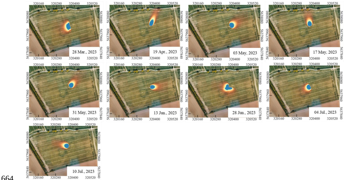
Figure C1: The estimated EC footprints for each TIR campaign flight time interval to be used to compare the TSEB-PT ET values within this spatial extent to the EC ET estimations.
