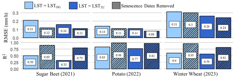
Figure 9: RMSE and R² between modeled TSEB-PT ET and EC derived ET, averaged over the EC flux footprint. Two TSEB-PT model runs are compared based on land surface temperature (LST) input: original (OG) and target corrected (TC). Statistical metrics are presented for the entire growing season and excluding senescence periods, highlighting the influence of canopy condition on model performance.
