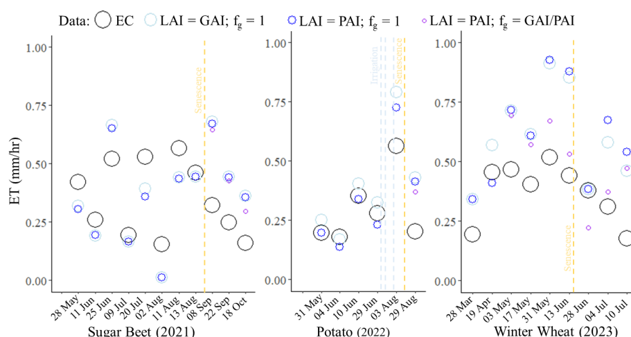
Figure 10: TSEB-PT evapotranspiration (ET) estimates were evaluated using different leaf area index (LAI) inputs: MS derived green area index (GAI), LiDAR derived plant area index (PAI), and their ratio, representing the fraction of green LAI ( f_g ), during periods of known senescence. UAV derived ET was compared against eddy covariance (EC) measurements within the EC flux footprint to assess model sensitivity to LAI input type. Notably, f_g scaling was introduced earlier for winter wheat in the model than the officially declared onset of senescence to account for localized early decline observed in the western portion of the field due to water deficits.
