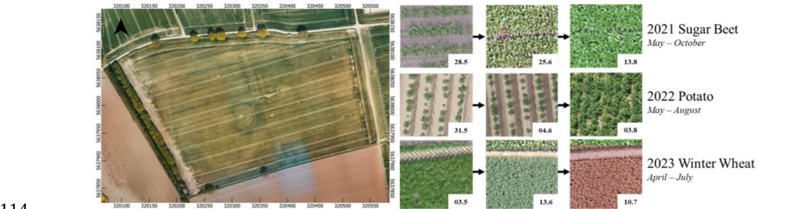
Figure 1: The field experiment site (left) with the EC and meteorological station located in the center of the field. The different crop cover type for each year (right) with example images of plant structure and fraction of vegetation coverage over the field throughout each growing season.
