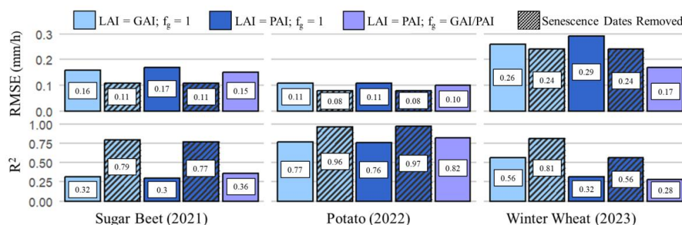
Figure 10: TSEB-PT evapotranspiration (ET) estimates were evaluated using different leaf area index (LAI) inputs: MS derived green area index (GAI), LiDAR derived plant area index (PAI), and their ratio, representing the fraction of green LAI ( f_g ), during periods of known senescence. UAV derived ET was compared against eddy covariance (EC) measurements within the EC flux footprint to assess model sensitivity to LAI input type. Notably, f_g scaling was introduced earlier for winter wheat in the model than the officially declared onset of senescence to account for localized early decline observed in the western portion of the field due to water deficits.
