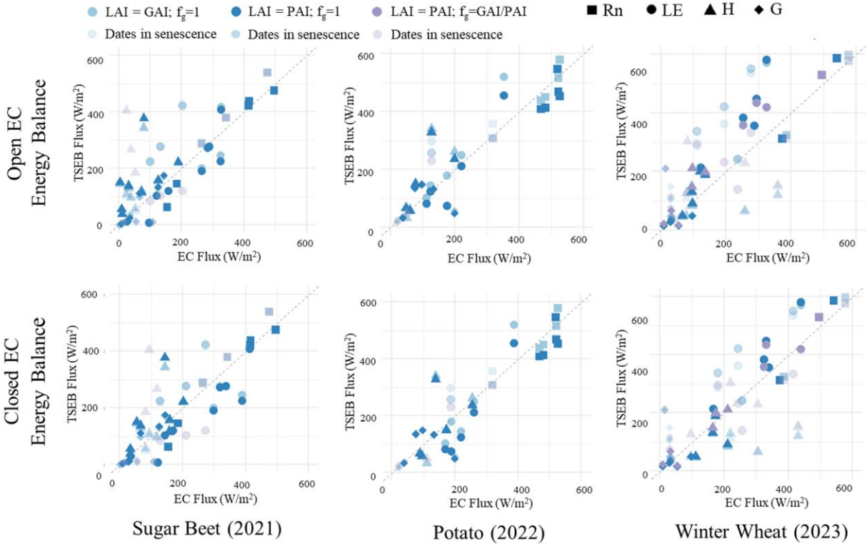
Figure 10. Comparison of modeled TSEB-PT energy fluxes (Rn, LE, H, and G) with eddy covariance (EC) observations across three crop seasons under different LAI and f_g parameterizations. Upper panels show comparisons using open EC fluxes, and lower panels show closed EC energy balance fluxes. Colors indicate model configurations (GAI; PAI; PAI with dynamic ( f_g ), symbols indicate flux components, and lighter markers represent senescence-period observations.
