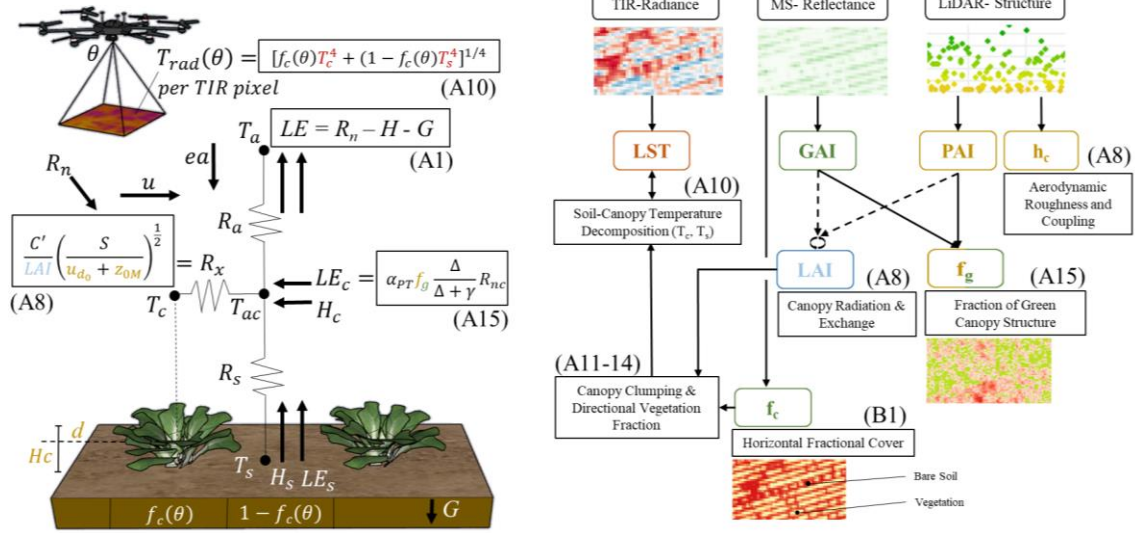
Figure 4. Conceptual schematic and example data illustrating how UAV-derived inputs constrain energy-balance partitioning within the TSEB-PT model. The left panel shows the model architecture, highlighting the partitioning of net radiation ( R_n ) into latent ( LE ), sensible ( H ), and ground ( G ) heat fluxes and the pathways through which UAV-derived variables influence these components. Key inputs include land surface temperature ( LST ), leaf area index ( LAI ), fractional cover ( f_c ), fraction of LAI that is green ( f_g ), and canopy height ( h_c ). The right panel illustrates the corresponding UAV-derived spatial inputs and their roles within pyTSEB. Spatially varying multispectral NDVI-derived fractional cover was supplied as the f_c input for sugar beet and potato, whereas f_c = 1 was used for the nearly closed winter wheat canopy. Within pyTSEB, LAI and f_c contribute to canopy clumping and the directional vegetation fraction f_c(\theta) used for soil–canopy radiometric temperature decomposition. The f_g scales potential canopy transpiration within the Priestley–Taylor formulation, while LiDAR-derived h_c contributes to aerodynamic roughness and turbulent heat exchange. Example spatial data are shown for sugar beet. Abbreviations: R_a ( s\ m^{-1} ), aerodynamic resistance to heat transport; R_x ( s\ m^{-1} ), canopy boundary-layer resistance; R_s ( s\ m^{-1} ), soil boundary-layer resistance; T_c and T_s (K), canopy and soil component temperatures; z_{0M} (m), aerodynamic roughness length for momentum; d_0 (m), zero-plane displacement height; and \alpha_{PT} (–), Priestley–Taylor coefficient.
