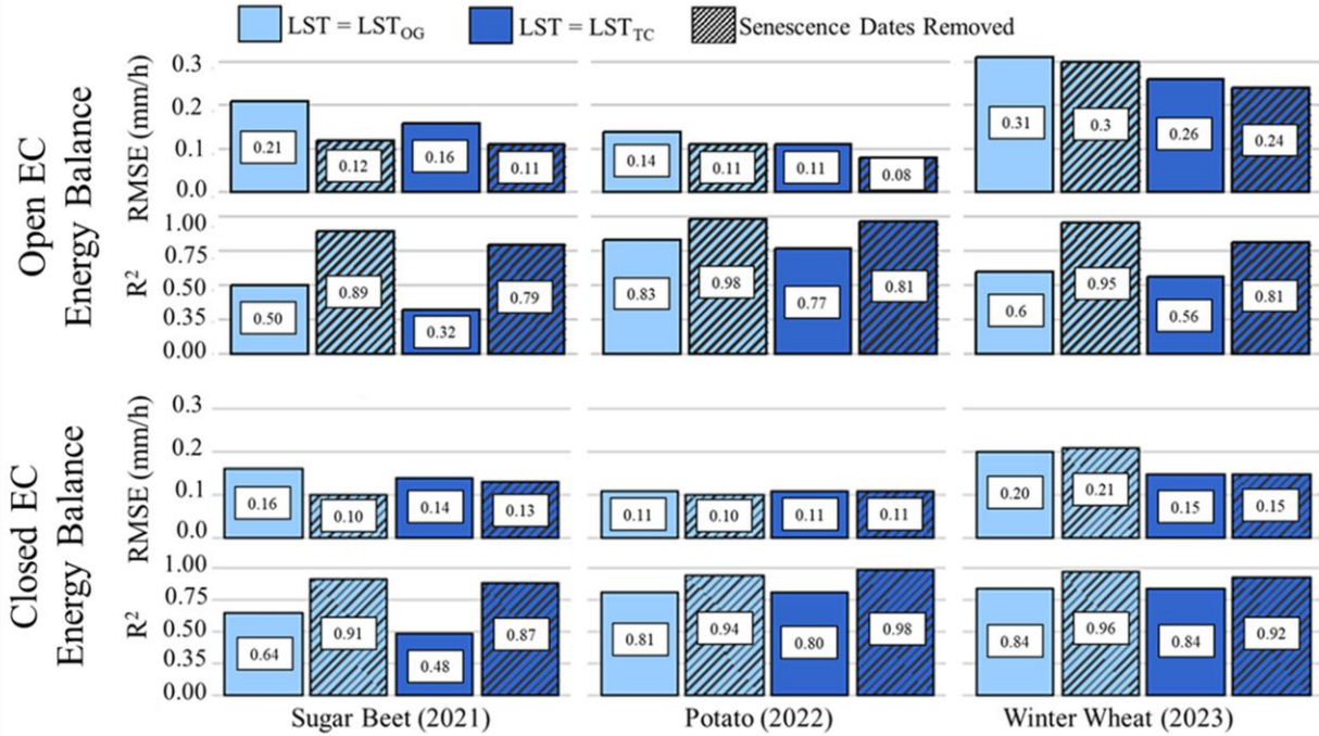
Figure 9. RMSE and R^2 between modeled TSEB-PT ET and EC-derived ET under open and closed energy balance conditions, averaged over the EC flux footprint. Model runs are compared using original (LST og ) and target corrected (LST Tc ) land surface temperature inputs. Metrics are shown for the full growing season and with senescence periods excluded.
